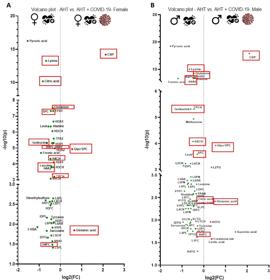
417 418 Fig 4. Univariate comparison of AHT cohorts with and without COVID-19, separated by gender, respectively 419 FC > 1.2 , p < 0.05 , FDR < 0.01 : The red features are significantly increased in COVID-19 patients, while the green ones are 420 decreased. Plot (A) shows the comparison of AHT vs. AHT + COVID-19 for females, plot (B) shows this comparison for male 421 gender. Features in red boxes are common in both genders and in COVID-19 affected considering AHT. AHT= Arterial hyper- 422 tension, Creatinine.lab= Creatinine from laboratory report, CRP= C-reactive protein, 3-HBA= 3- Hydroxybutyric acid. 423
