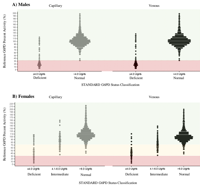
Figure 2. G6PD activity classification of the STANDARD G6PD and reference assays for A) males and B) females. G6PD status classification measured by the STANDARD G6PD test is shown on the X-axis, for capillary (grey) and venous (black) specimens, respectively. Results are plotted by the reference G6PD percent activity (Y-axis). Shaded areas correspond to true G6PD normal (green), intermediate (yellow), and deficient (red) status classifications on the reference assay.
