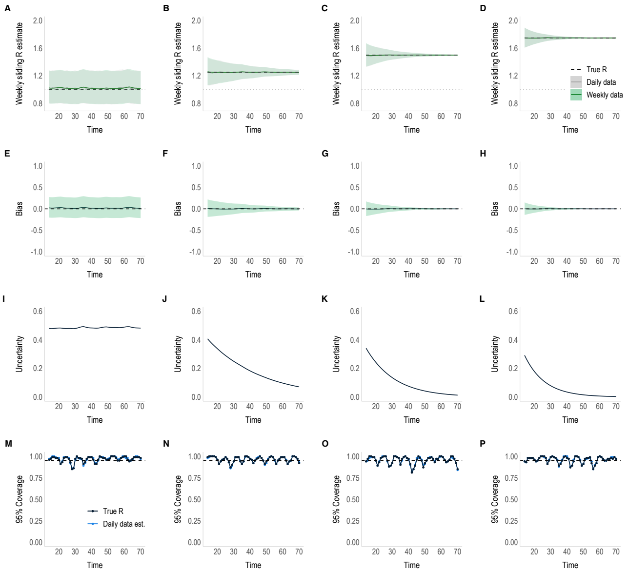
Figure S9. Performance of the method when estimating a constant R_t for 100 simulated epidemics. A-D) The mean weekly sliding R_t estimates using daily data (grey) and weekly data (green). The black dashed line represents the true value of R_t that the 100 simulations are based on, which is either A) 1, B) 1.25, C) 1.5, or D) 1.75. The estimates and their 95% credible intervals (shaded areas) are very similar and therefore overlap. E-H) The bias (or absolute difference) in the mean R_t estimated from weekly data compared to the true value of R_t . The shaded area corresponds to the 95% quantiles of the bias across the 100 simulations. I-L) The uncertainty (mean width of the 95% credible interval) in the R_t values estimated from weekly data. M-P) The proportion of the 100 R_t estimates obtained from weekly data where the 95% credible interval encompasses either the true value of R_t (black) or the value of R_t that would have been estimated from daily data (blue). Here, the 95% coverage is similar for both the true value of R_t and the daily data estimate, and therefore they overlap.
