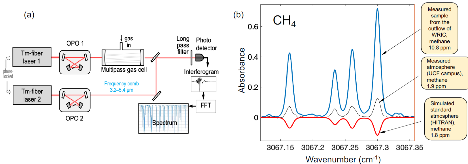
Supplemental Figure 3. (a) Schematic of the MIR DCS setup. A pair of phase-locked Tm-fiber lasers pump a pair of subharmonic OPOs. The two beams are combined, passed through a multipass gas cell with an equivalent path length of 76 m, and detected with a fast infrared detector. The detector signal is digitized, and fast Fourier transformed to retrieve the optical spectrum. (b) Measured and simulated absorption spectra of \text{CH}_4 . Measured are examples of sample from whole room indirect calorimetry (WRIC) at the translational research institute (TRI) and University of Central Florida (UCF) A simulated spectrum (HITRAN) is inverted for clarity.
