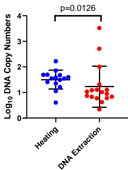
Figure 3. Detection of sporozoites by qPCR in the heating and DNA extraction arms. The error bars show the mean and the standard deviation. Each dot represents a mosquito.
