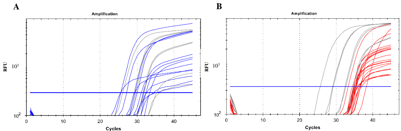
Figure 1. A qPCR amplification plot showing successful amplification of malaria parasite DNA from oocysts and sporozoites. Panel A represents the amplification of parasite DNA from oocysts with the blue curves being the parasite DNA and the grey being the plasmid controls of known concentrations that were used as positive controls. Panel B represents the amplification of parasite DNA from sporozoites with the red curves being the parasite DNA while the grey lines represent the plasmid controls of known concentrations that were used as positive controls. The blue horizontal line represents the threshold value; any curve above this is considered an infection. RFU - relative fluorescence unit
