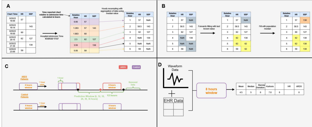
Supplemental Figure 1: Depiction of Hourly Resampling (A), Accounting for Missing Data (B), Windowing Data for Classification (C), and Statistics Used for Continuous Variables That Make Up Features (D)
