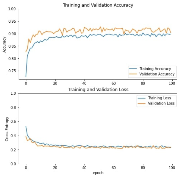
(a) Resnet50 training and validation accuracy vs epochs(Top)
