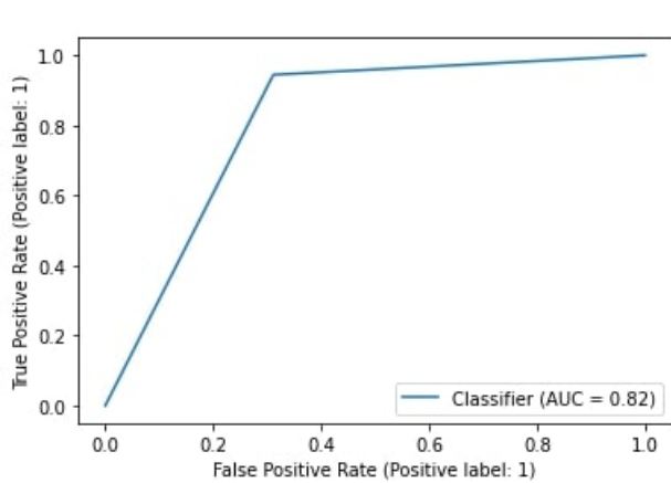
(a) Densenet121 ROC curve
