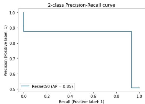
(b) Resnet50 precision-recall curve
