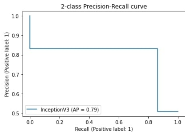
(b) InceptionV3 precision-recall curve
