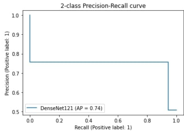
(b) Densenet121 precision-recall curve
