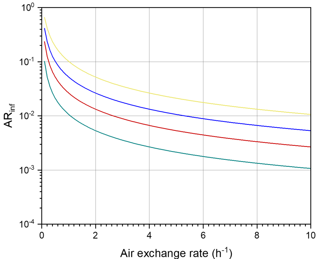
Figure 5. Absolute risk of infection AR_{inf} according to Wells-Riley depending on the air exchange rate. The calculation was carried out with equation (1) for different quanta, see text for parameters and colors of the curves.
