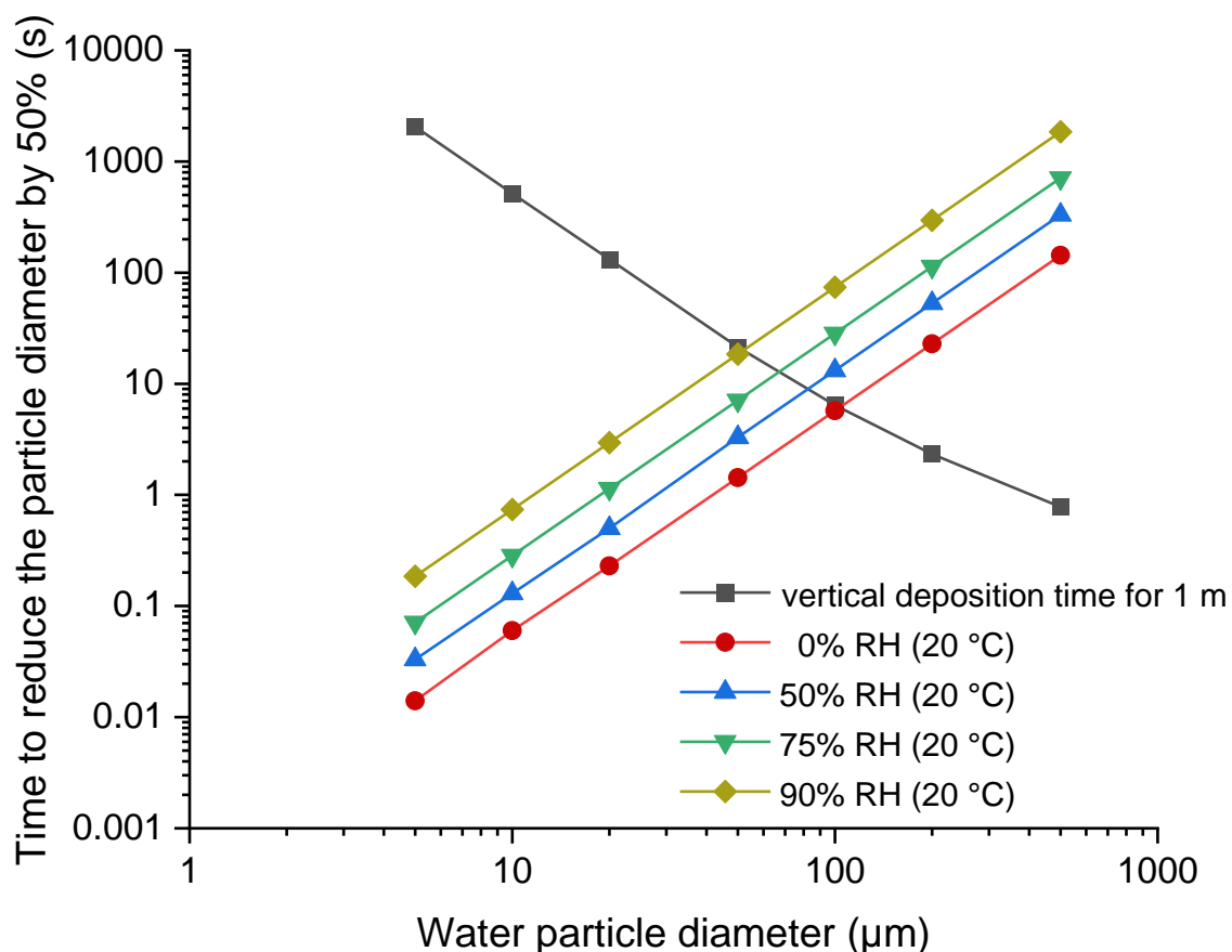
Figure 2. Time required for the diameter of aqueous particles to decrease by 50% through evaporation at 20 °C and various relative humidities. For comparison, the time required for a particle to sink by 1 m in still air is also plotted (black curve).
