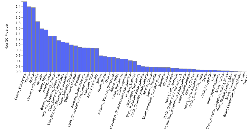
(a) GWAS
