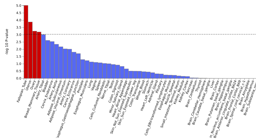
(b) WGWS
