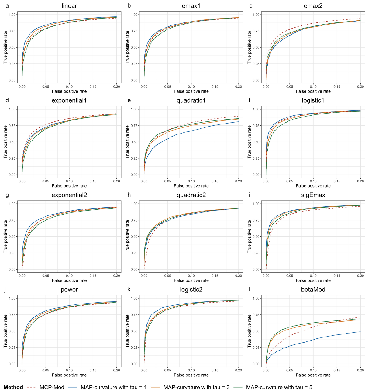
Figure 2: ROC curves of MAP-curvature and MCP-Mod across different true dose-response models with the sample size of 40 patients per arm. The ROC curves of MCP-Mod in (a)-(f) are produced with the true dose-response model not included in the candidate model set, and the ROC curves of MCP-Mod in (g)-(l) are produced with the true dose-response model not included in the candidate model set.
