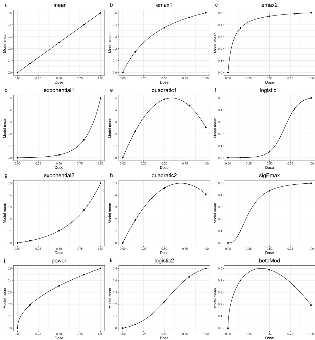
Figure 1: Dose-response shapes selected for the true dose-response model.
