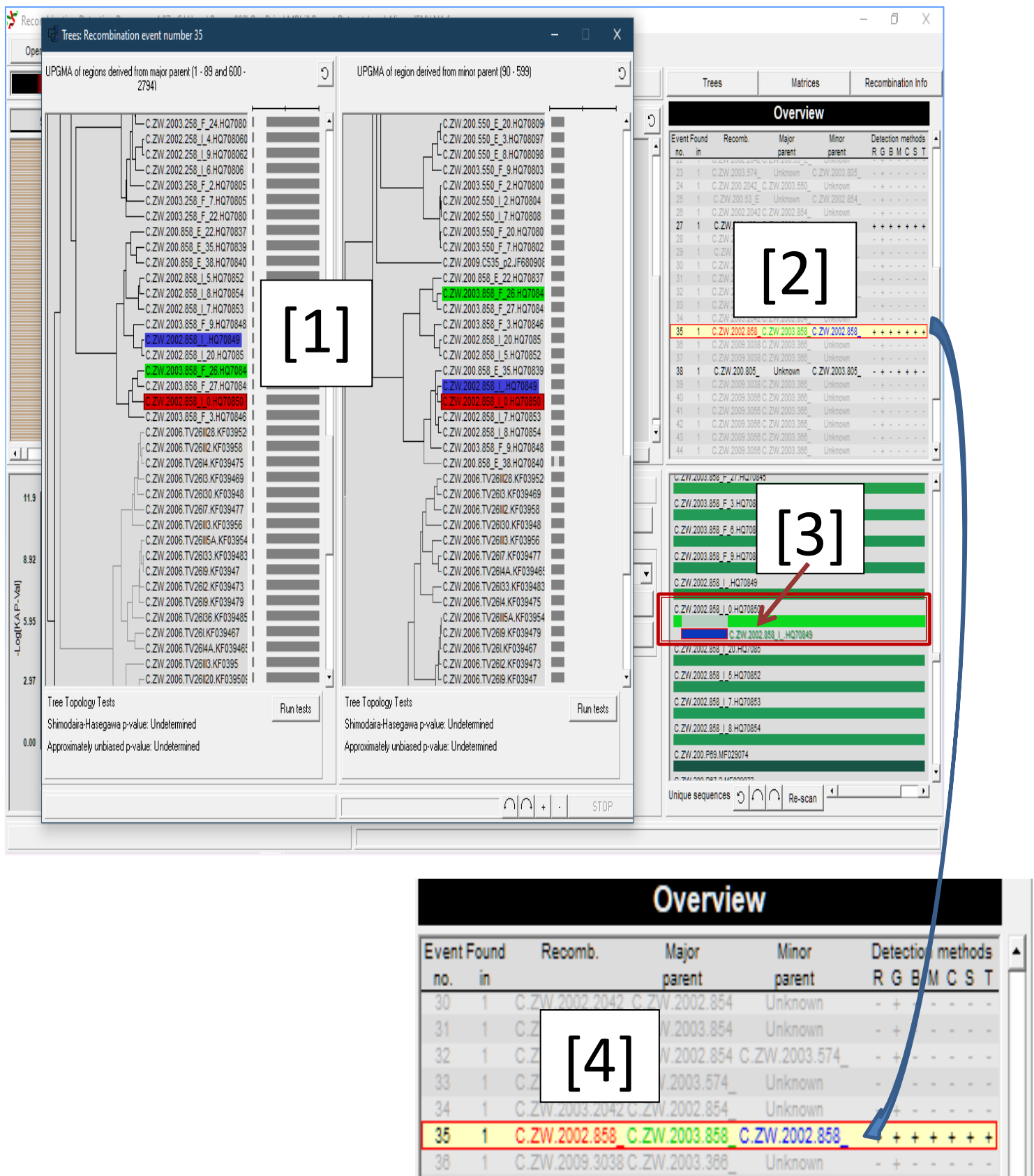
Fig 1: Overall analysis of recombination using GENECONV analysis method in RDP 4. The sequences are colour-coded as follows: Recombinant = Red, Major Parent = Green, Minor Parent = Blue. [1] UPGMA Phylogenetic tree to show how the best representative of evidence of recombination is related, the left phylogenetic tree shows the related region derived from the Major Parent (The derived regions' nucleotide positions provided) in contrast to the minor parent, the right phylogenetic tree illustrates the phylogenetic relationship of the region derived from the minor parent and the recombinant in contrast to the major parent (the
