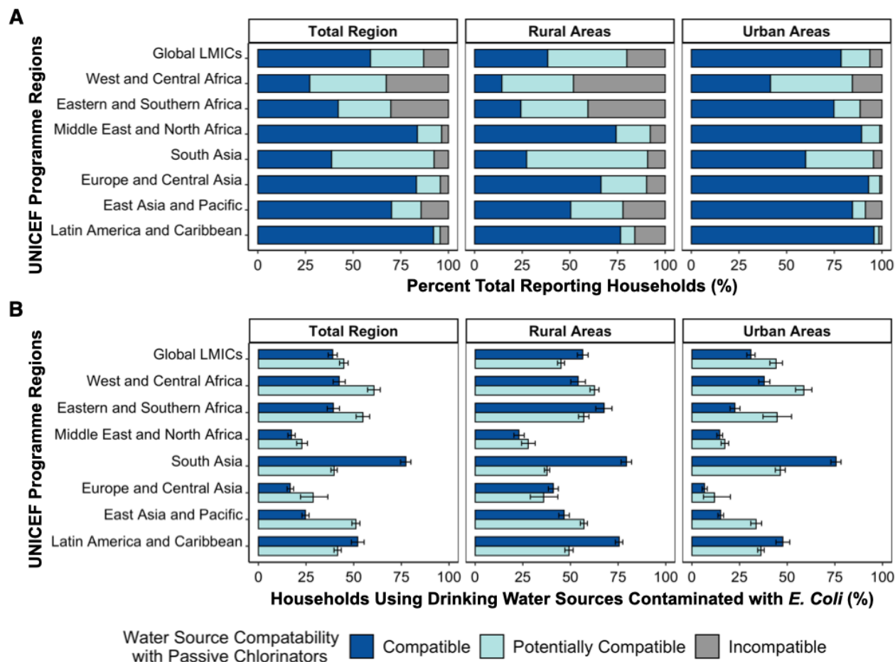
Figure 2. Household primary drinking water source compatibility with passive chlorinators (A), and (B) Percent (%) of compatible and potentially compatible water sources contaminated with E. coli . Water source categories are classified as being compatible in dark blue (piped supplies and water kiosks), potentially compatible in light blue (improved non-piped sources excluding protected dugwells), or incompatible in gray (unimproved sources and protected dugwells). Panel B data on regional microbial ( E. coli ) water contamination in urban and rural households was obtained from water quality questionnaires in Multiple Indicator Cluster Surveys (MICS 5 & 6). Error bars in panel B represent 95% confidence intervals calculated assuming an underlying binomial distribution. Additional data related to this figure can be found in Tables S6, S7, and S8 in the Supporting Information.
