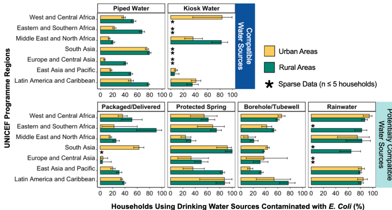
Figure 1. Microbial contamination of primary household drinking water sources, by facility type.
