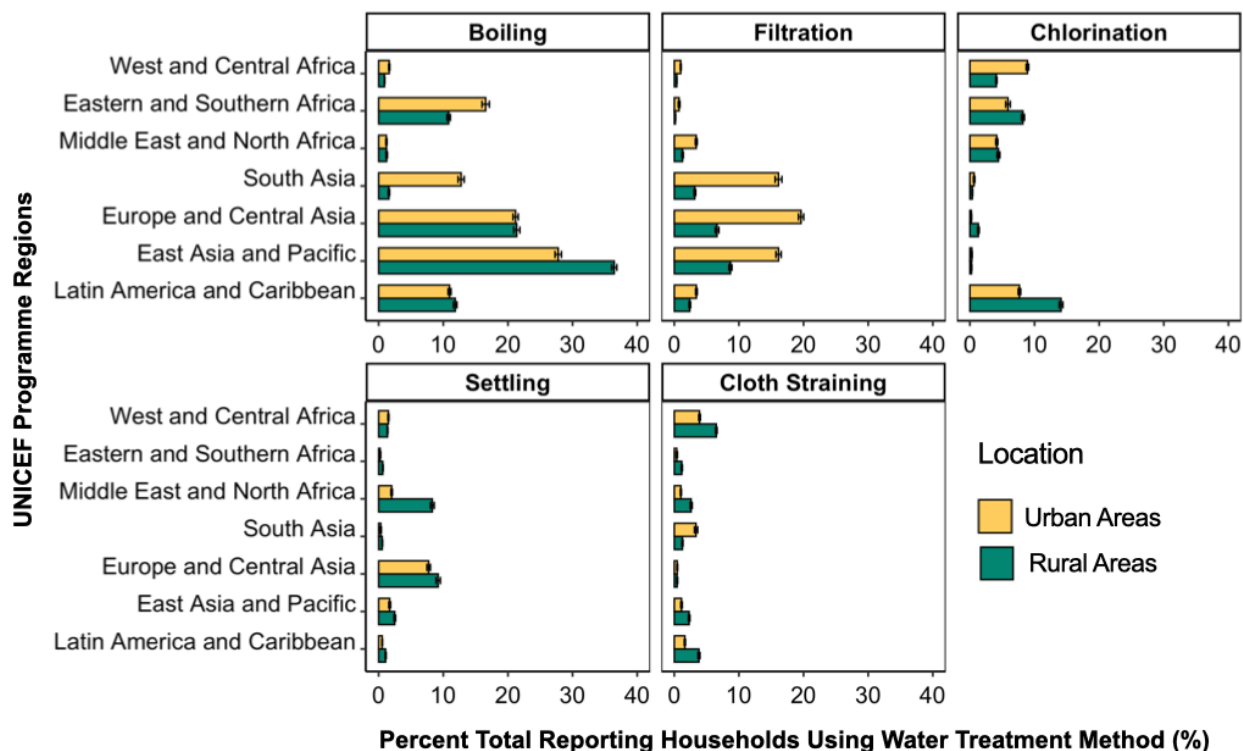
Figure 4. Household drinking water treatment practices , reported as percent (%) of total urban and rural households. Households could report multiple methods used including boiling, filtration (ceramic, sand, or composite filters), chlorination, settling, and/or cloth straining. Responses with proportions below < 1 % across regions (e.g., solar disinfection) are not shown. Error bars represent 95% confidence intervals calculated assuming an underlying binomial distribution. The total number of households in each region surveyed are as follows: West and Central Africa (216,419), Eastern and Southern Africa (68,056), Middle East and North Africa (87,161), South Asia (73,862), Europe and Central Asia (65,646), East Asia and Pacific (85,264), and Latin America and Caribbean (124,046). Full data is available in Table S11 in the Supporting Information.
