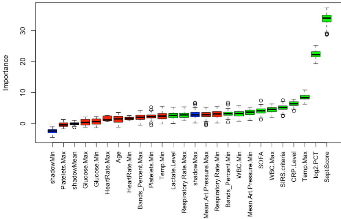
Figure S5. Boruta Random Forest analysis. RPD = forced (176 sepsis, 243 SIRS). In this figure, the blue boxes correspond to minimum, mean and maximum Z scores of shadow attributes. The red and green boxes, respectively, represent Z scores of rejected and confirmed attributes.
