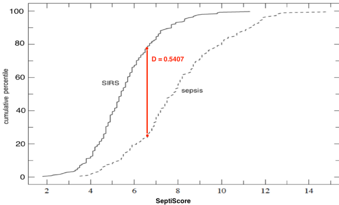
Figure S6. Cumulative distribution curves for the SeptiScore. There were 243 SIRS datapoints and 176 sepsis datapoints with SeptiScore values available ( 417/419 = 100.0\% of all patients in cohort).
