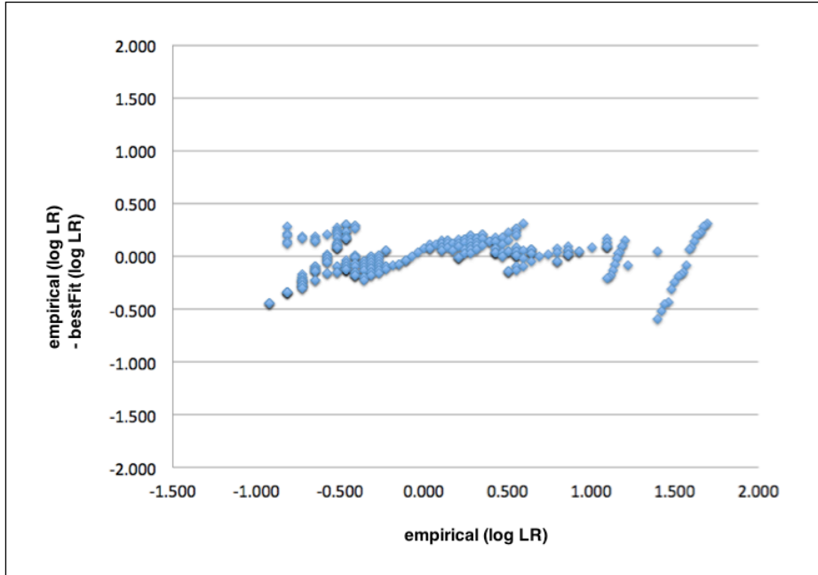
Figure S9. Plot of residuals for the equation described in Figure S8, in log space, centered around zero. The empirical best-fit equation is an exponential function, with x = SeptiScore, LR=10^y and y = 0.0168x^2 + 0.1047x - 1.3376 and R^2 = 0.93811 .
