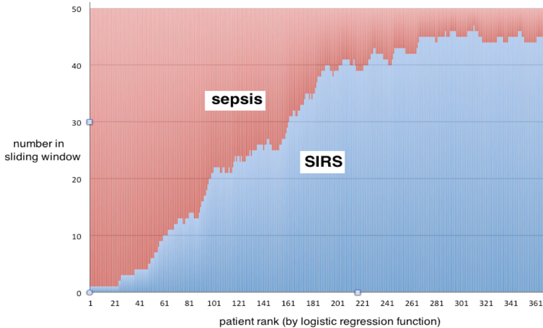
Figure S11. Number of SIRS and sepsis patients, per (50 patient wide) sliding window defined by the logistic regression function given by Eq. (S4).
