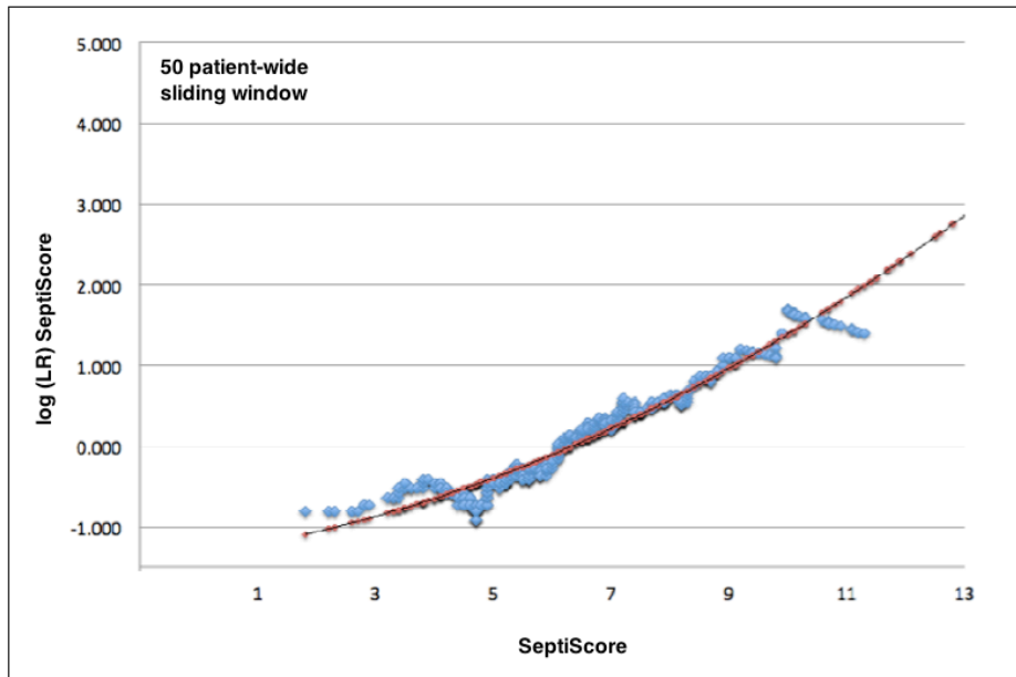
Figure S8. Likelihood ratio (LR) plot for the SeptiScore. (A) The empirical best-fit equation is an exponential function, with x = \text{SeptiScore} , LR=10^y and y = 0.0168x^2 + 0.1047x - 1.3376 . For the fit shown in this graphic, R^2 = 0.93811 .
