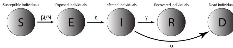
Figure 1. The basic SEIRD Model. The whole population is divided into 5 compartments: Susceptible, Exposed, Infected, Recovered, and Dead. \beta , \epsilon , \gamma , and \alpha are parameters characterizing transitions between the relevant compartments. These transition parameters are described below. Although there are technically links between the S, E, and R compartments to D (through natural deaths), adding all of them would clutter the diagram, so we have left them out.
