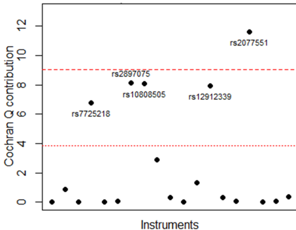
Figure 3: Identification of pleiotropic instruments in the MR on the effect of IPF on GERD. Individual variant contributions to Cochran's Q heterogeneity statistic with the 5 th (dotted line) and Bonferroni corrected (0.05/19 th ) percentiles (dashed line) of a chi-squared with 1 degree of freedom.
