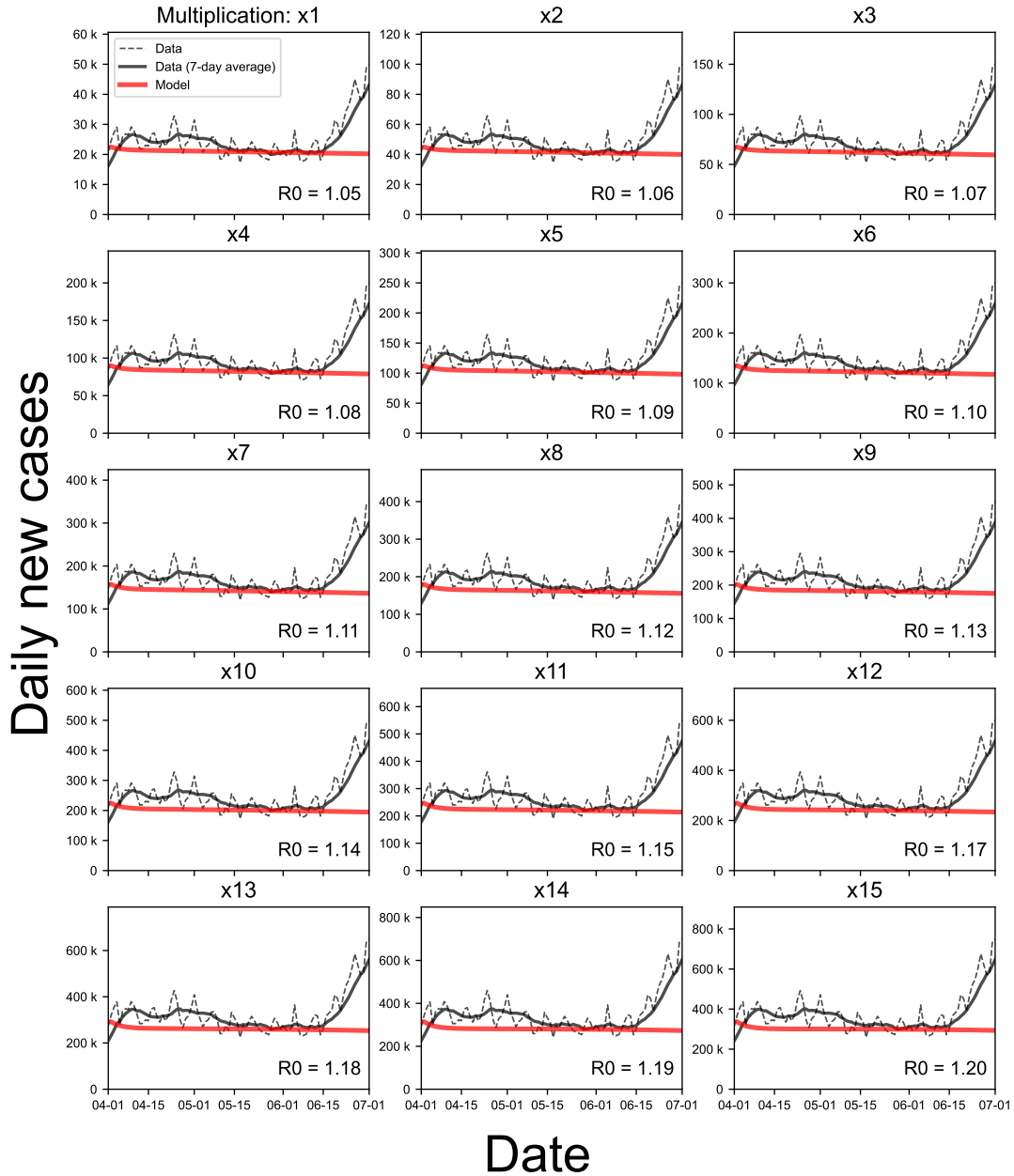
Supplementary Figure S2: Baseline epidemic model for multiplied epidemic trends. Each subplot shows the result of the baseline epidemic model for multiplied epidemic trends by different multiplication factors ranging from 1 to 15. The black curves show the total daily new cases over the entire US from April 1, 2020 to July 1, 2020 (dotted for the multiplied data and solid for the 7-day averages). The red curves describe the trend simulated by our epidemic model for the reproduction number that best describes the trend. The multiplication factor and the reproduction number are shown in each subplot.
