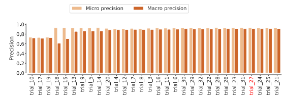
3H T5 optimization: precision
