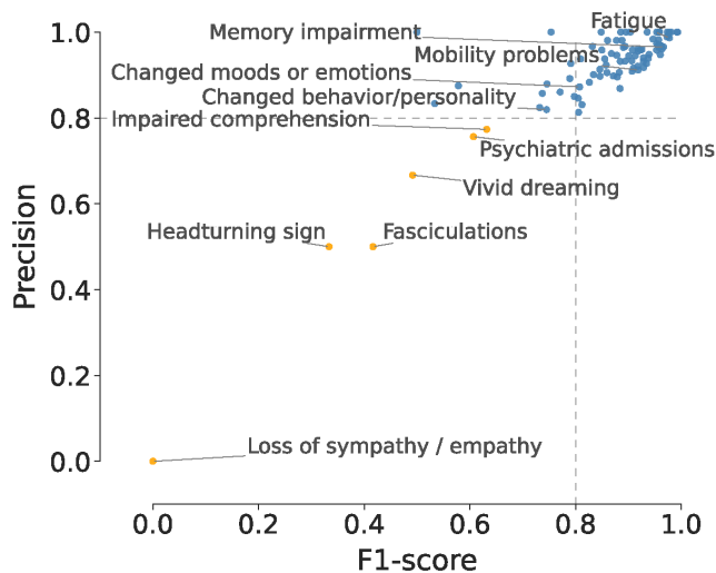
3C Bio_ClinicalBERT
