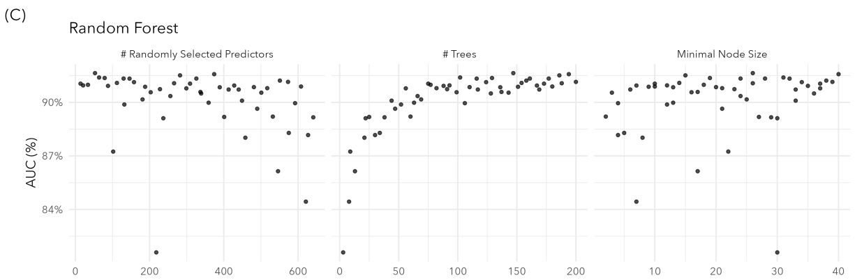
Supplemental Figure 5. Results from the five-fold cross-validation used to determine the top performing machine learning model. Area under the curve (AUC) are presented according to hyperparameters for (A) LASSO, (B) XGBoost, and (C) Random Forest.
