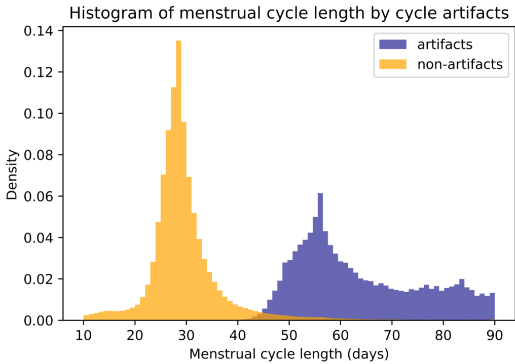
Figure SM2 Histograms of cycle length among cycles that were identified as potential artifacts and those that were not.
