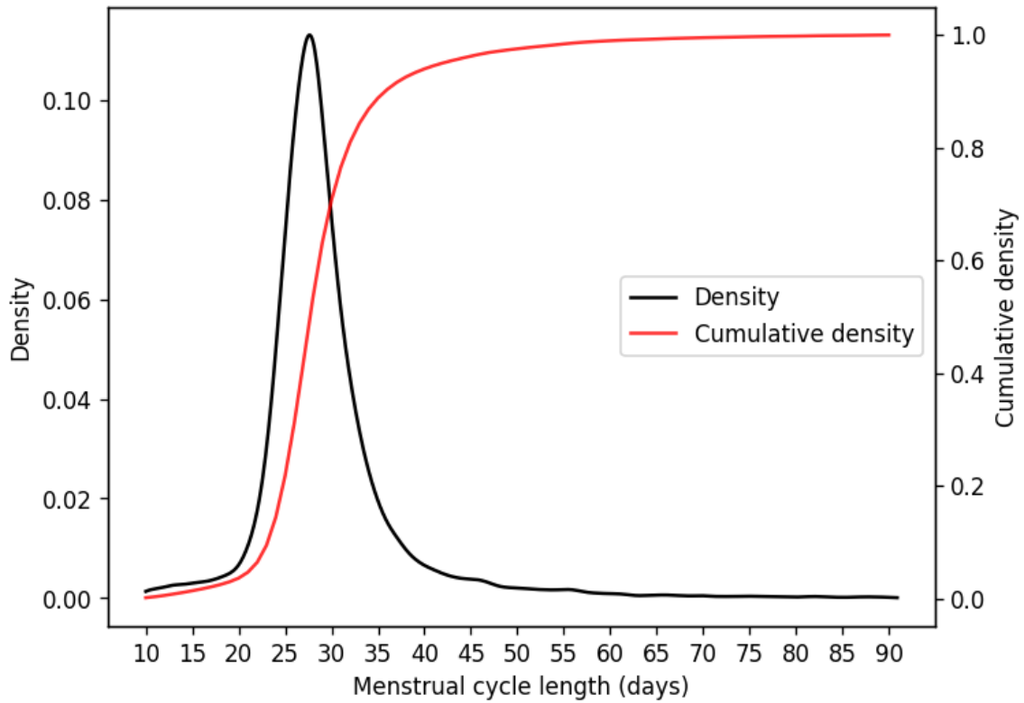
Figure S2 By-participant distribution (density and cumulative density) of menstrual cycle length across 165,668 cycles from 12,608 participants in the AWHs
