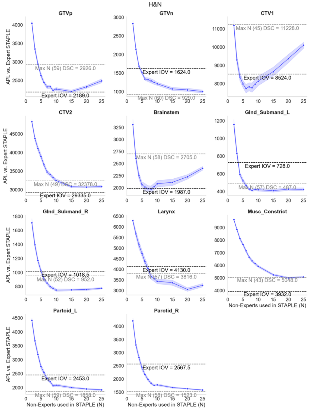
Figure D11. Bootstrap experiment results for H&N case using APL.
