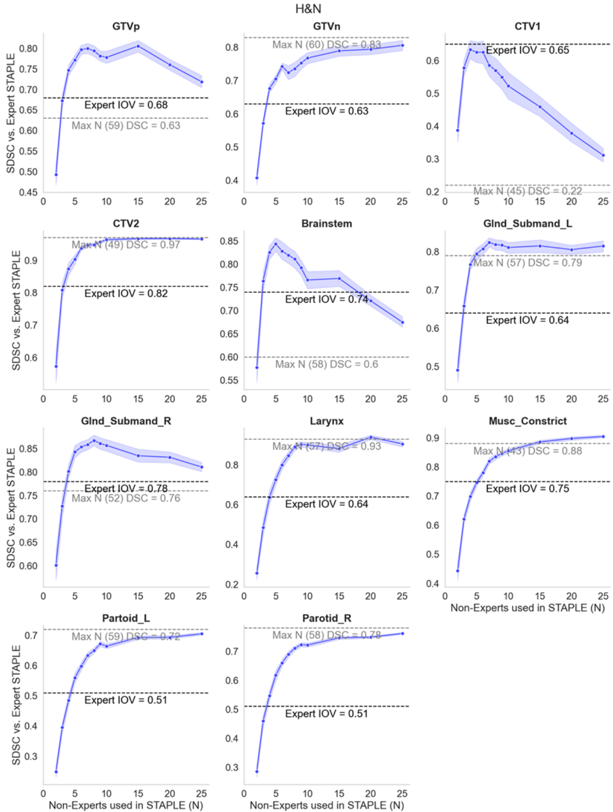
Figure D9. Bootstrap experiment results for H&N case using SDSC.
