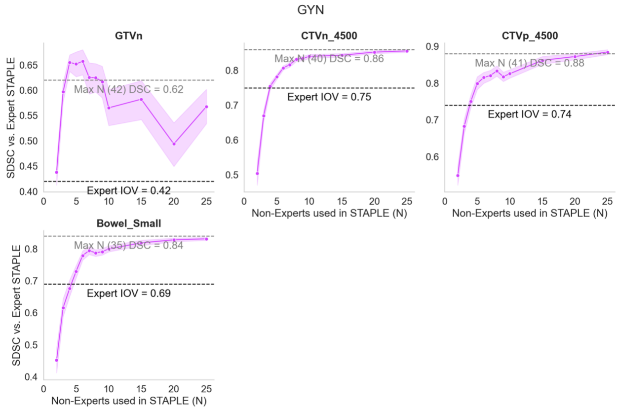
Figure D12. Bootstrap experiment results for GYN case using SDSC.
