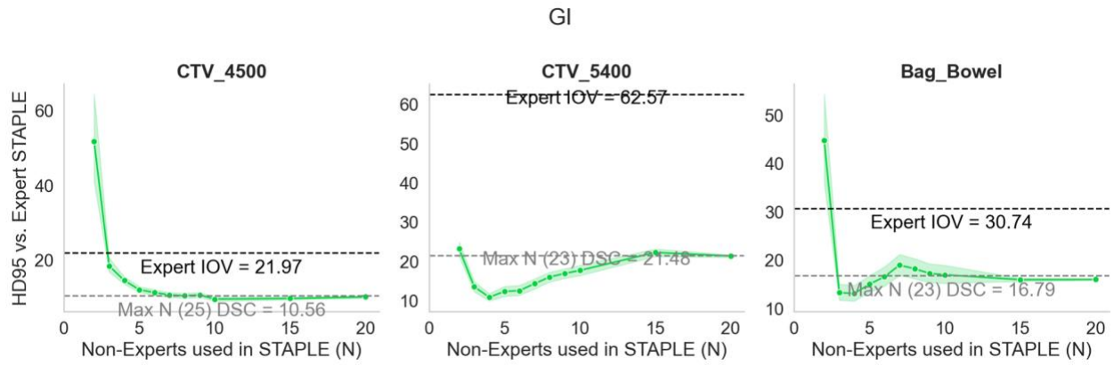
Figure D16. Bootstrap experiment results for GI case using HD95.
