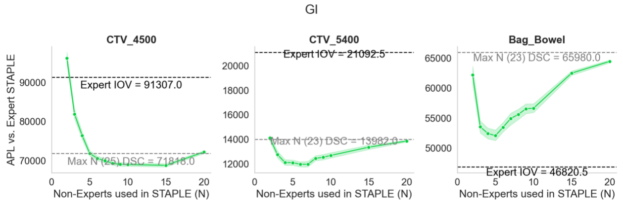
Figure D17. Bootstrap experiment results for GI case using APL.
