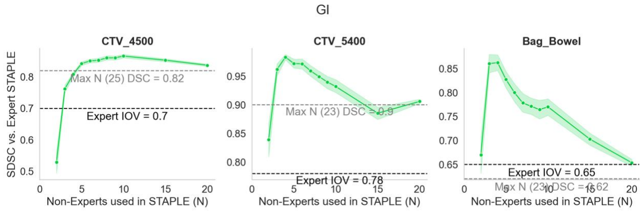
Figure D15. Bootstrap experiment results for GI case using SDSC.
