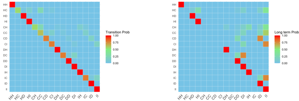
Figure 5: Transition matrix (left) and long term transition matrix (right).
