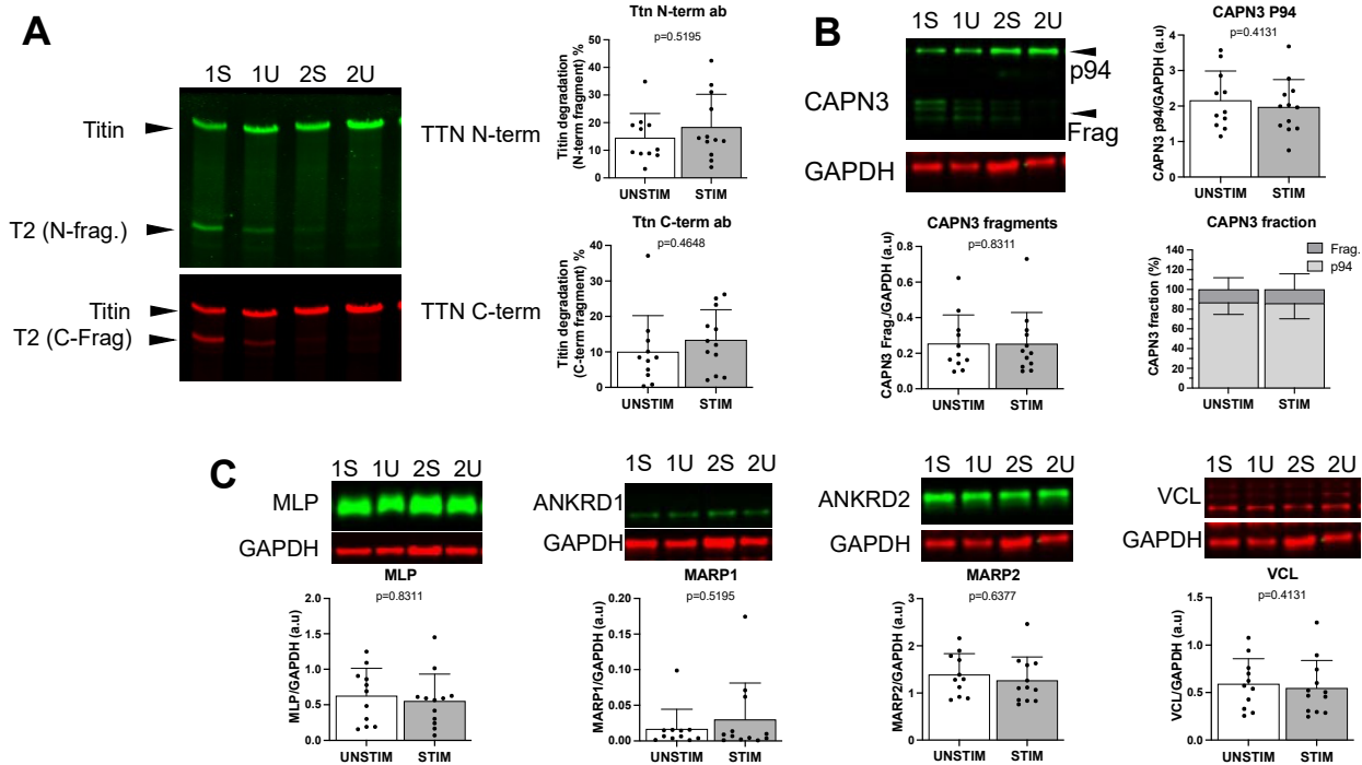
Figure 3. Content of titin fragments and titin-binding proteins. Western blot images and data of the N-terminal and C-terminal fragments of titin ( A ). ( B ) Calpain-3 (CAPN3), muscle specific protease at the N2A region of titin. Full-length, inactive calpain-3 (P94) and calpain fragments comprise the CAPN3 fraction. ( C ) Titin-binding proteins. Muscle Lim-Protein (MLP), telethonin-binding protein in the Z-disk region; muscle ankyrin repeat proteins 1 and 2 (MARP1 and MARP2), stress-responsive proteins at the N2A region of titin; and vinculin (VCL), membrane protein involved in sarcomere stability. Sample Western blot images are from the stimulated (STIM) and unstimulated (UNSTIM) sides of subjects 1 and 2. P-values shown from Wilcoxon tests; mean and standard deviation shown.
