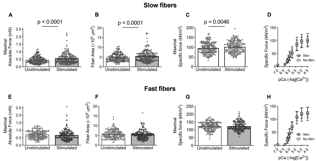
Figure 2. In slow fibers, maximal calcium activated force ( A ), fiber cross-sectional area ( B ), and maximal specific force ( C ) were significantly greater in the stimulated hemidiaphragm. Averaged specific force vs pCa relationship ( D ). In fast fibers, no significant differences in maximal force ( E ), fiber cross-sectional area ( F ), maximal specific force ( G ), or the specific force vs pCa relationship ( H ) were detected. Mixed effect model; mean and standard deviation shown. A-C and E-G dots are data from individual fibers. Statistical analysis by linear mixed model.
