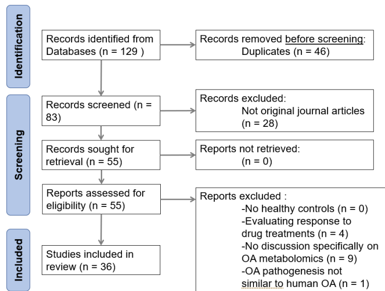
Figure 1: Flow diagram of literature search performed on July 20, 2021, displaying the study selection process.
