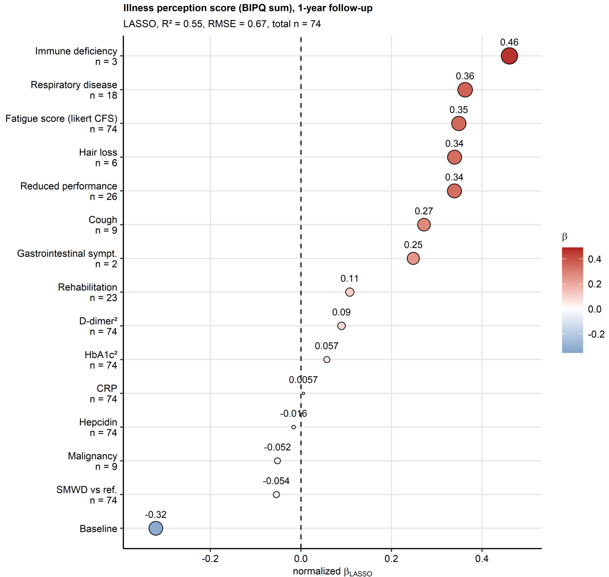
Supplementary Figure S4. Non-zero coefficient estimates of the LASSO multi-parameter model.
