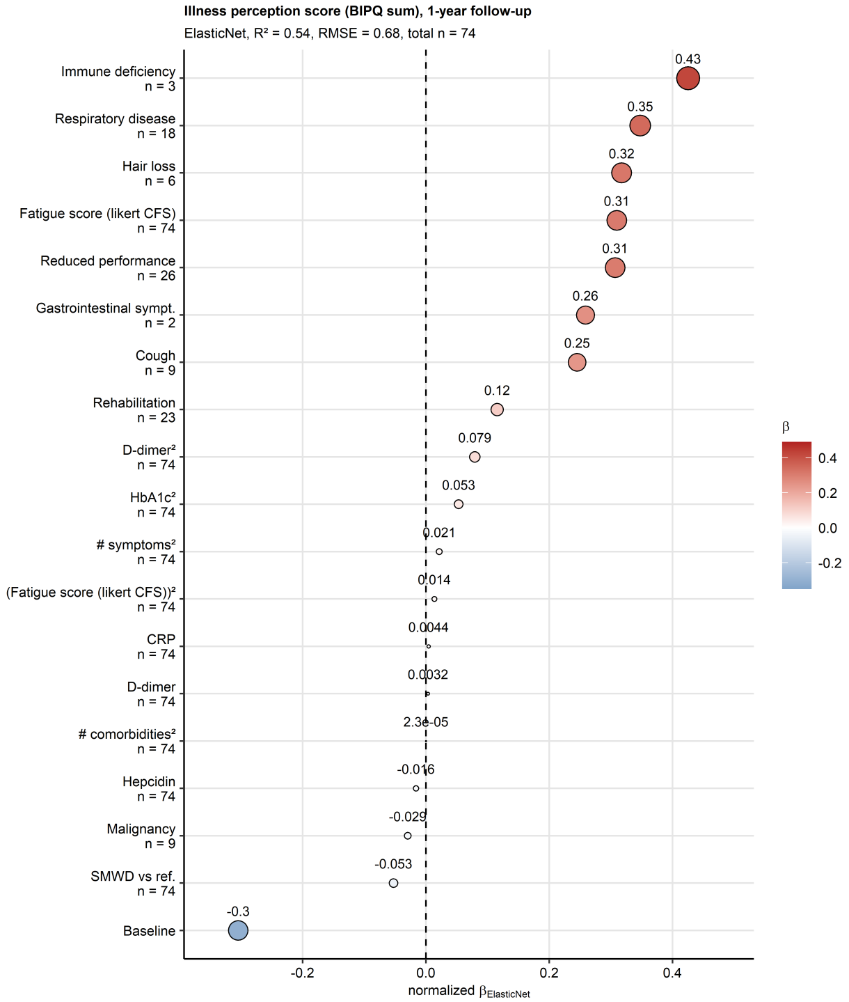
Supplementary Figure S3. Non-zero coefficient estimates of the Elastic Net multi-parameter model.
