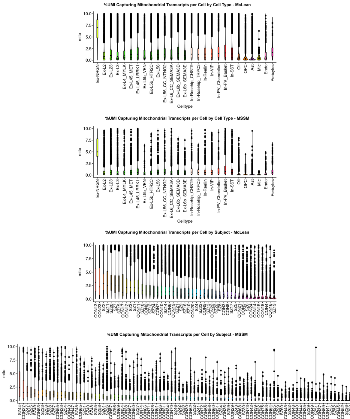
Extended Data Fig. 2c. Mitochondrial transcript capture across cell-types and individuals. Distribution of UMI percentages that map to mitochondrially encoded genes across cells of each type or individual for each cohort. Box plots are centered around the median, with the interquartile range (IQR) defining the box. The upper whisker extends to the largest value no further than 1.5 \times \text{IQR} from the end of the box. The lower whisker extends to the smallest value at most 1.5 \times \text{IQR} from the end of the box.
