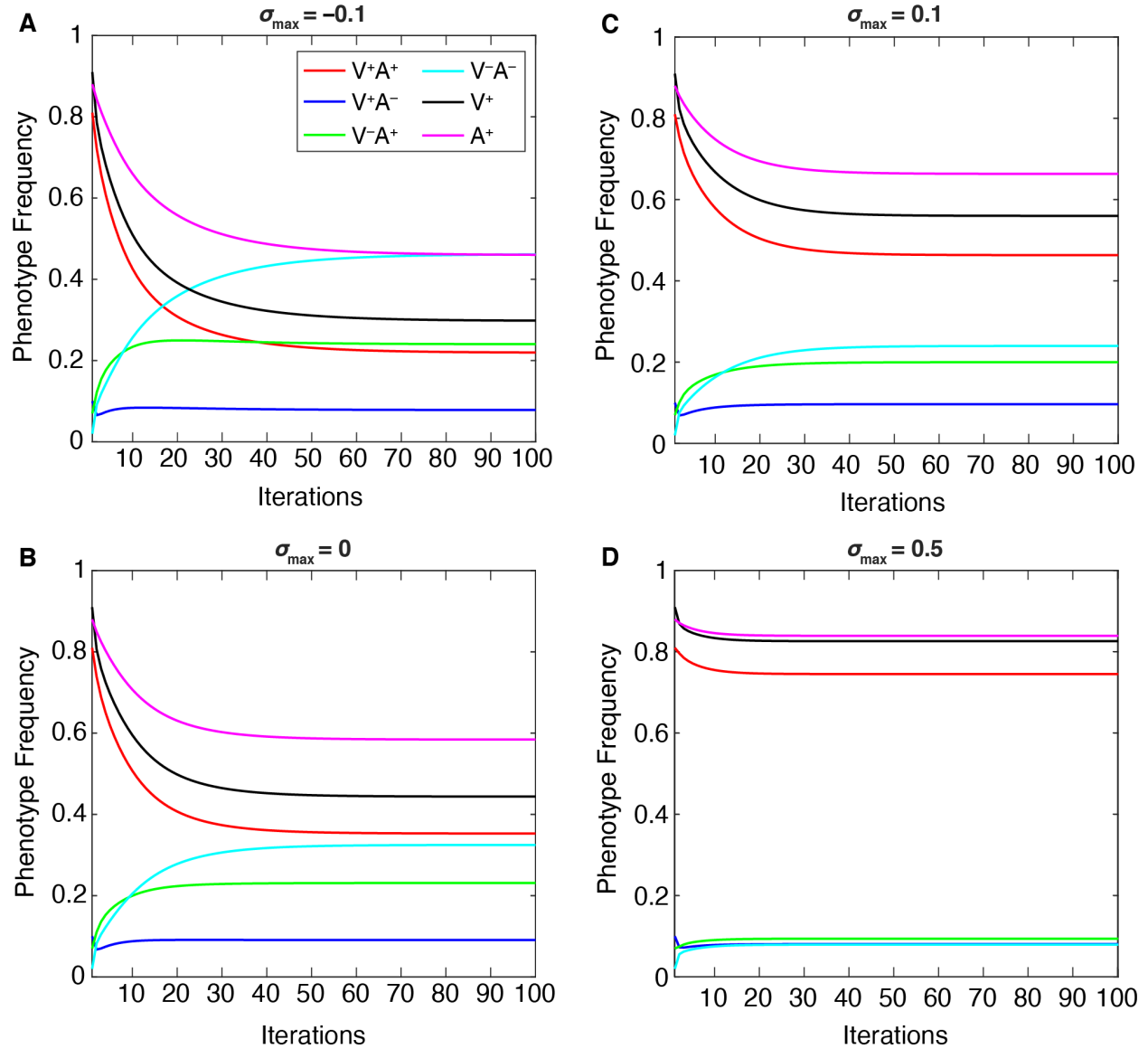
Figure S3: Temporal effects of cultural selection (with oblique transmission). The equilibrium phenotype frequencies change as the maximum cultural selection coefficient ( \sigma_{\max} ) is varied: A. \sigma_{\max} = -0.1 ; B. \sigma_{\max} = 0 ; C. \sigma_{\max} = 0.1 ; D. \sigma_{\max} = 0.5 . Oblique transmission is included, and other parameters are held at default values ( Table 1 ). (Compare this figure with Figure 3 (bottom row) , which shows results with vertical transmission only.) Cultural selection against vaccinated individuals increases the frequency of V^-A^- , while decreasing the other frequencies ( A ), whereas increased cultural selection favoring vaccinated individuals increases V^+A^+ frequencies while decreasing the other frequencies ( C, D ). The highest levels of conflicting phenotypes ( V^+A^- and V^-A^+ ) were observed when cultural selection was neutral ( B ).
