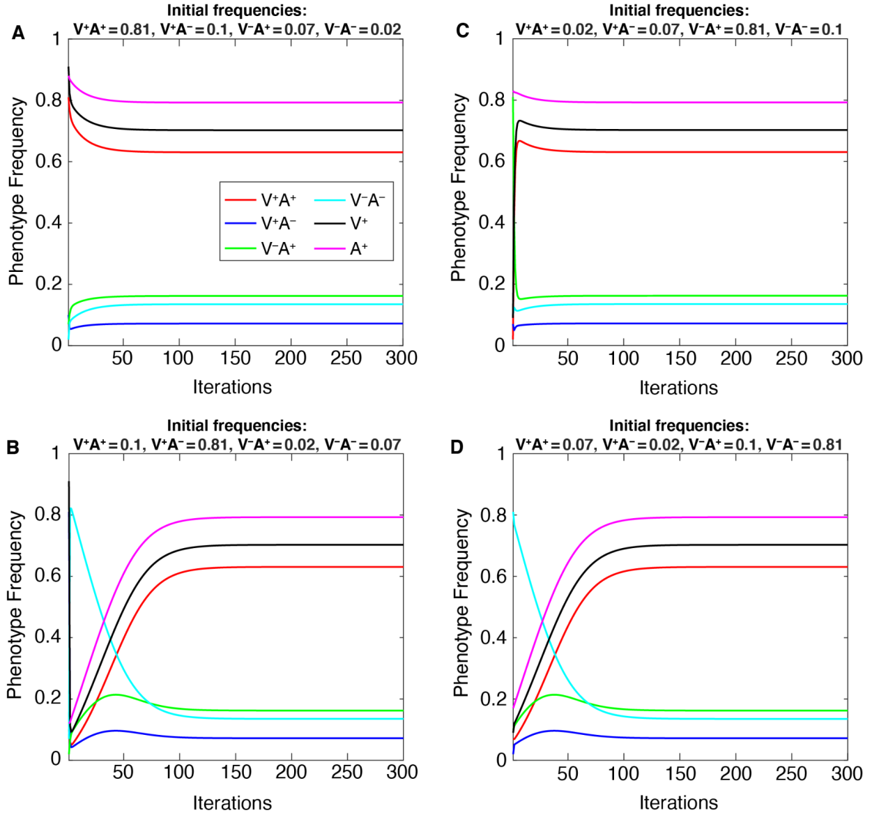
Figure S1: Population frequencies reach stable equilibria determined by the parameter space, not by initial frequencies. Each phenotype approaches the same equilibrium frequency for a given set of parameters regardless of its initial frequency in our simulations. Each of the four phenotype frequencies and the total V^+ and A^+ frequencies (vertical axis) approach equilibrium values prior to iteration 300 and remain stably at those frequencies (compare this figure with Figure 3 (top row) , which shows the first 100 iterations of the same simulations). We varied the initial frequencies, such that we begin each simulation with a different phenotype at an initial high frequency (0.81): A ) x_1 (V^+A^+) = 0.81 , x_2 (V^+A^-) = 0.1 , x_3 (V^-A^+) = 0.07 , x_4 (V^-A^-) = 0.02 ; B ) x_1 (V^+A^+) = 0.1 , x_2 (V^+A^-) = 0.81 , x_3 (V^-A^+) = 0.02 , x_4 (V^-A^-) = 0.07 ; C ) x_1 (V^+A^+) = 0.02 , x_2 (V^+A^-) = 0.07 , x_3 (V^-A^+) = 0.81 , x_4 (V^-A^-) = 0.1 ; D ) x_1 (V^+A^+) = 0.07 , x_2 (V^+A^-) = 0.02 , x_3 (V^-A^+) = 0.1 , x_4 (V^-A^-) = 0.81 . The remaining parameters are held at default values ( Table 1 ) and simulations were performed without oblique transmission (only parent-to-offspring transmission) . These results indicate that equilibrium frequencies are determined by the parameter space, not initial frequencies.
