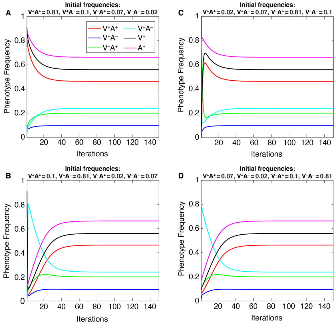
Figure S2: Population frequencies reach stable equilibria determined by the parameter space, not by initial frequencies (with oblique transmission). Each phenotype approaches the same equilibrium frequency for a given parameter set regardless of its initial frequency in our simulations. Each of the four phenotype frequencies and the total V^+ and A^+ frequencies (vertical axis) approach equilibrium values prior to iteration 300 and remain stably at those frequencies (compare this figure with Figure 3 (top row) , which shows results with only vertical transmission). We varied the initial frequencies, such that we begin each simulation with a different phenotype at an initial high frequency (0.81): V^+A^+ in panel A , V^+A^- in panel B , V^-A^+ in panel C , V^-A^- in panel D ; the remaining phenotypes are set to lower frequencies (0.1, 0.07, 0.02). See Figure S1 for a full listing of these initial frequencies. The remaining parameters are held at default values ( Table 1 ) and these simulations included both vertical and oblique transmission .
