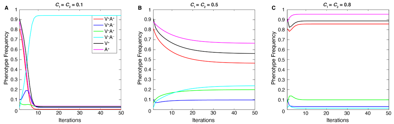
Figure S4: Temporal effects of confidence transmission (with oblique transmission). The change in phenotype frequencies over 50 iterations as vaccine confidence transmission in mixed couples ( C_1=C_2 ) is varied ( A . C_1=C_2=0.1 ; B . C_1=C_2=0.5 ; C . C_1=C_2 = 0.8 ). Oblique transmission is included and other parameters are held at default values (Table 1). The population equilibrates at over 90% V^-A^- at low confidence transmission ( A ). Increasing the probability of confidence transmission results in higher V^+A^+ frequencies and lower V^-A^- ( B , C ). In comparison to simulations with only vertical transmission ( Figure 4 ), phenotype frequencies reach equilibrium at values closer to mid-range levels (i.e. V^+A^+ levels at equilibrium are reduced while other frequencies are increased). It is also worth noting that the V^-A^- equilibrium value is higher than V^-A^+ at C_1=C_2 = 0.5 when oblique transmission is added.
