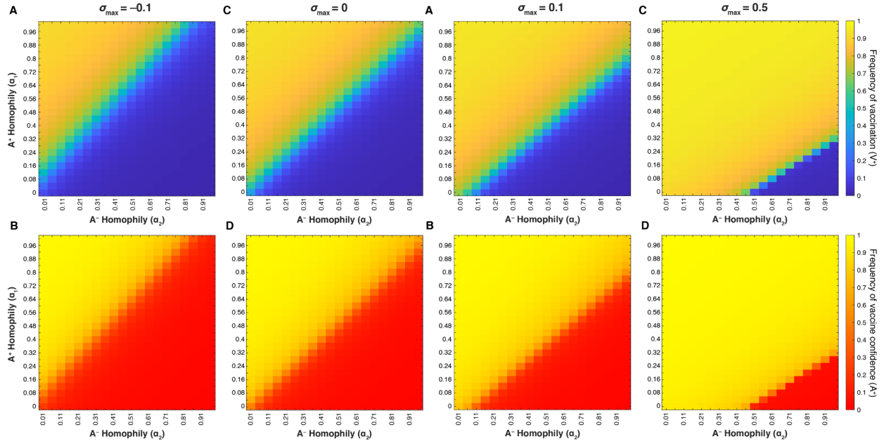
Figure S7: Homophily between individuals with similar vaccine beliefs can shift the equilibrium frequencies of both vaccination coverage and confidence (without oblique transmission). Heatmaps showing final vaccination coverage ( A, C ) and final vaccine confidence ( B, D ) after 100 timesteps without oblique transmission (only parent-to-offspring transmission; compare to Figure 11 ). As in previous figures, unspecified parameters are given in Table 1 . As vaccine-hesitant individuals ( A^- ) increasingly prefer to pair with one another (increasing \alpha_2 ; horizontal axis), vaccine-confident individuals ( A^+ ) must also preferentially interact to maintain high vaccine coverage ( \alpha_1 ; vertical axis); this tradeoff is modulated by the cultural selection pressures on vaccination ( \sigma_{\max} = -0.1 ( A, B ), \sigma_{\max} = 0 ( C, D ), \sigma_{\max} = 0.1 ( E, F ) and \sigma_{\max} = 0.5 ( G, H )).
