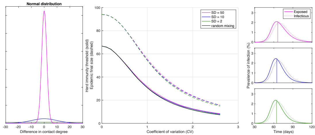
37 Figure S1: Herd immunity threshold and epidemic final size with gamma- 38 distributed exposure to infection and assortative mixing. Curves in central panel 39 generated with the SEIR model (Equation 1-4) assuming \mathcal{R}_0 = 3 and gamma- 40 distributed connectivity. Assortative mixing is implemented by imposing a normal 41 distribution for contact preferences such that individuals contact preferentially with 42 those with the similar contact degree (left). This illustration used normal distributions 43 with standard deviation SD = 50 (green); SD = 10 (blue); and SD = 2 (magenta). 44 More assortative mixing leads to more skewed epidemics. Herd immunity thresholds 45 were calculated numerically as the percentage of the population no longer susceptible 46 when new outbreaks are effectively prevented (approximately when the exposed 47 fraction crosses the peak in the absence of mitigation). Final sizes of the 48 corresponding unmitigated epidemics are also shown. Representative epidemics are 49 depicted on the right based on the rightmost CVs represented on the main panel (with 50 vertical lines marking the point when herd immunity is achieved). 51
