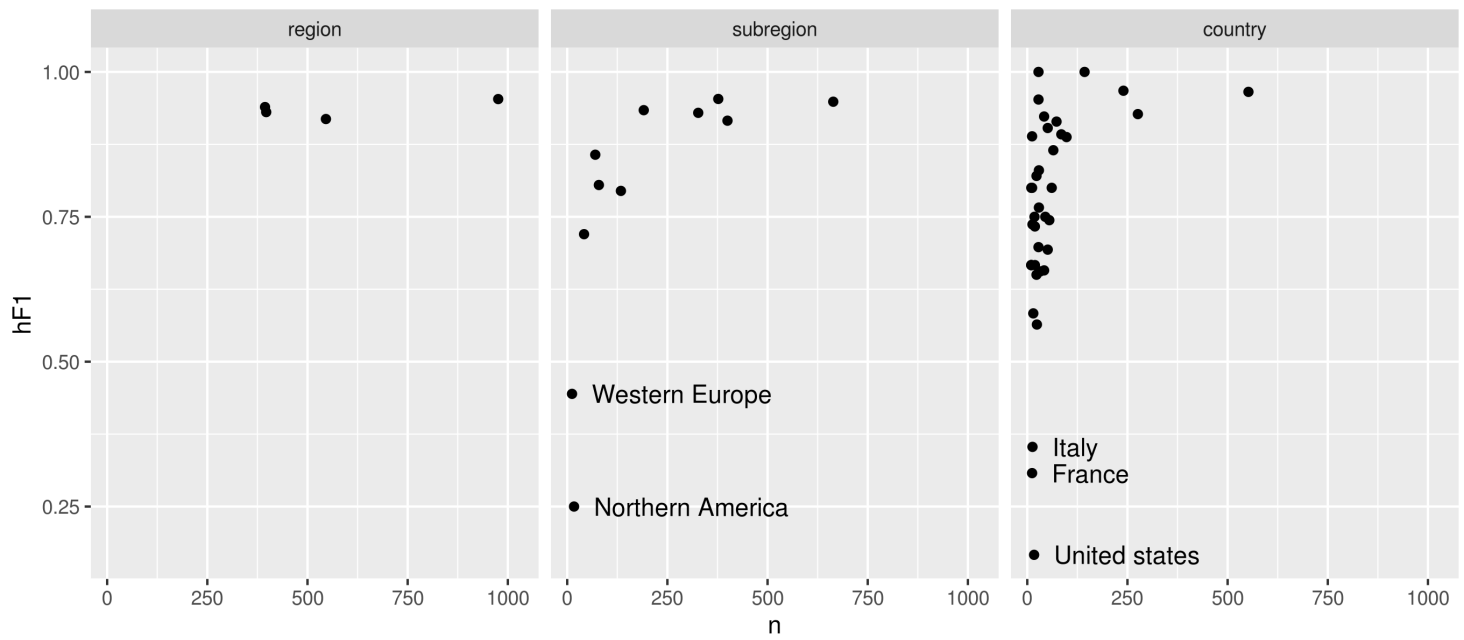
Figure S2. Scatter plots summarising the number of samples (x axis) vs hF1 score (y axis) generated by the optimised hML model. The three hierarchical levels (country/subregion/region) are represented by a separate plot panels. Each point is the hF1 score per class at that hierarchical level.
