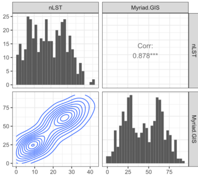
Figure S3. Distribution for the nLST score and Myriad GIS on 405 patients from the PAOLA-1 trial and their paired comparison.
