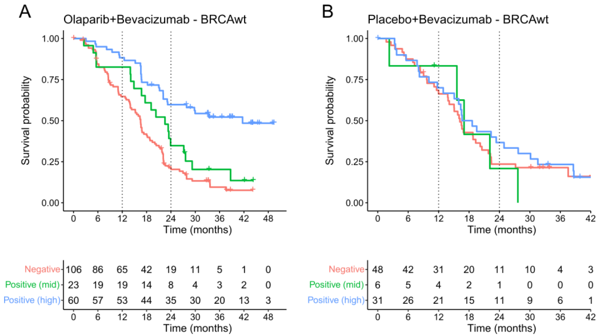
Figure S4. Kaplan-Meier plot of a three-way classification of the Myriad GIS score, with thresholds at 33 and 42, in the BRCA wild-type population upon A) Olaparib+Bevacizumab and B) Placebo+Bevacizumab treatment.
