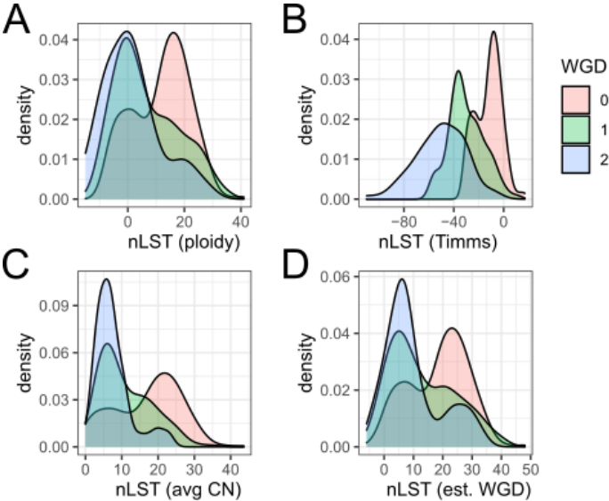
Figure S1. Normalized LST score distribution according to different methods and the number of WGD events as given by the ABSOLUTE software. A) Ploidy-based method with k=3.5 . B) Ploidy-based method with k=15.5 . C) Method based on the average copy number. D) WGD-based method.
