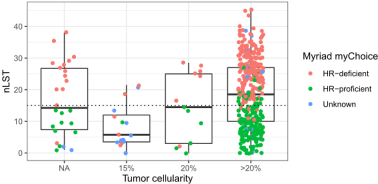
Figure S2. Distribution of nLST scores with respect to the tumor content as estimated by the Oncoscan analysis software.
