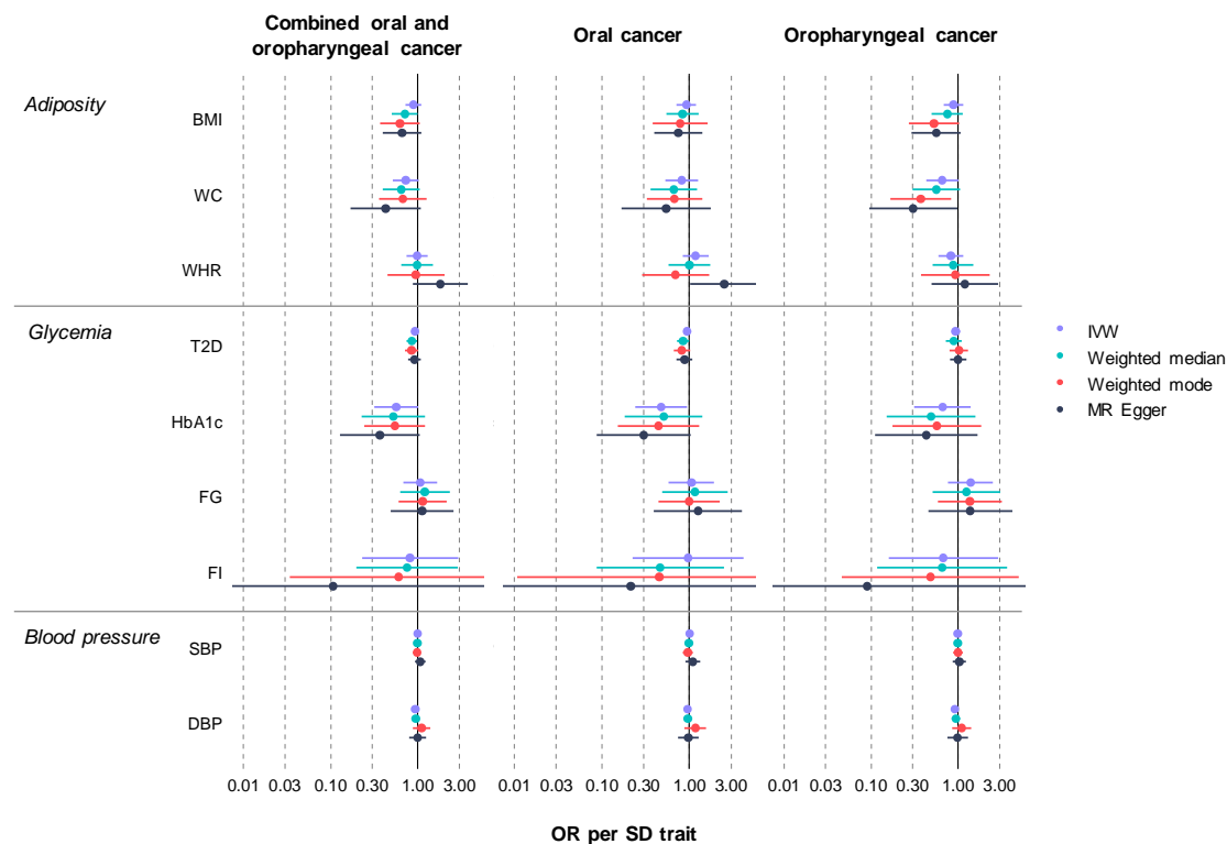
297 Figure 2. Mendelian randomization results of genetically-proxied metabolic disorders with 298 risk of oral and oropharyngeal cancer including sensitivity analyses in GAME-ON 299
