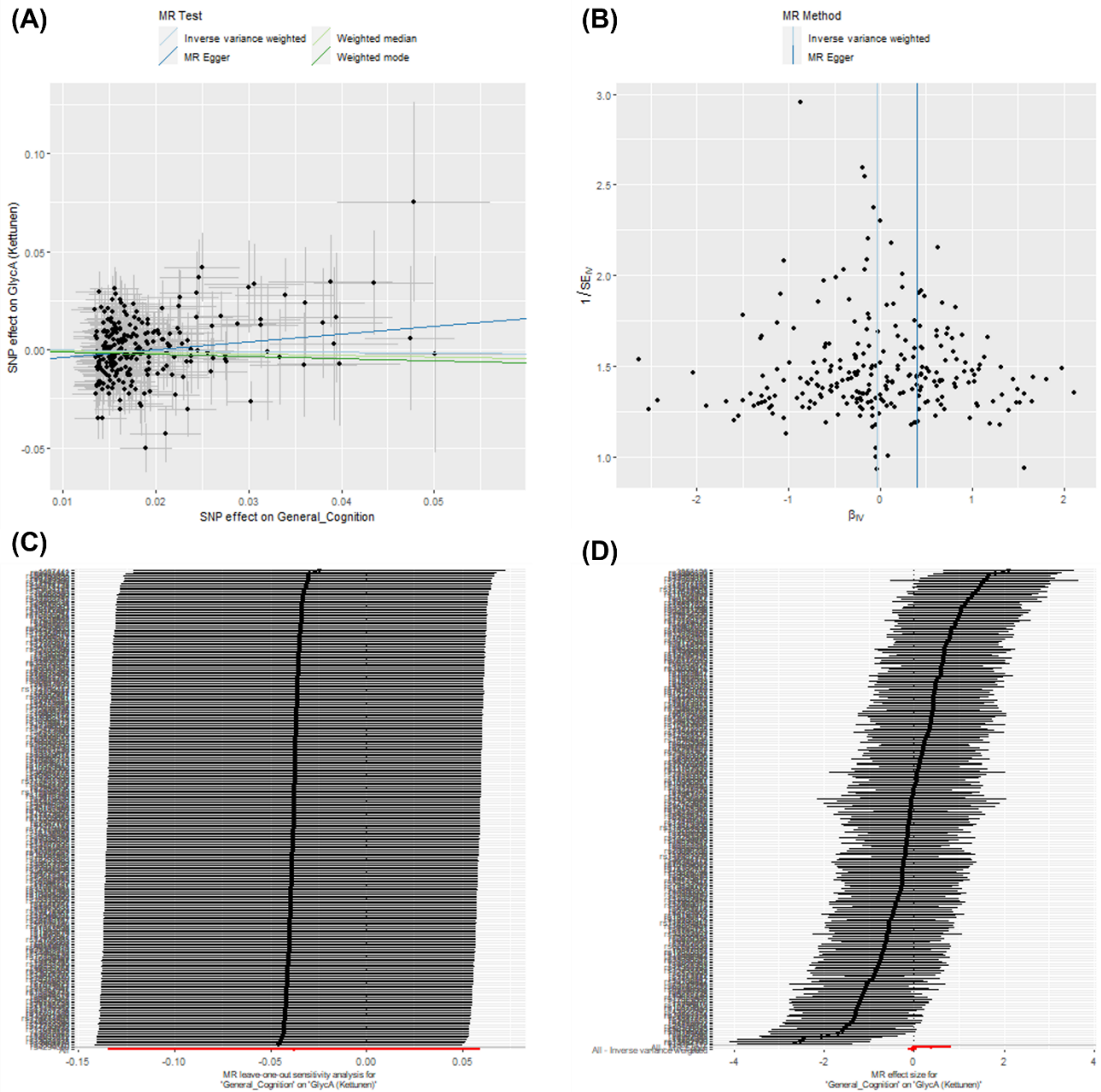
Figure S15. Two-sample MR sensitivity plots: effect of general cognitive ability on GlycA (Kettunen et al. GWAS). Graphs include (A) scatter plot of results from four main MR methods, (B) funnel plot showing each SNP causal estimate against its precision (asymmetry may indicate directional pleiotropy), (C) leave-one-out plot showing inverse-variance weighted estimates after removing each individual SNP in turn, (D) forest plot of causal estimates for each SNP.
