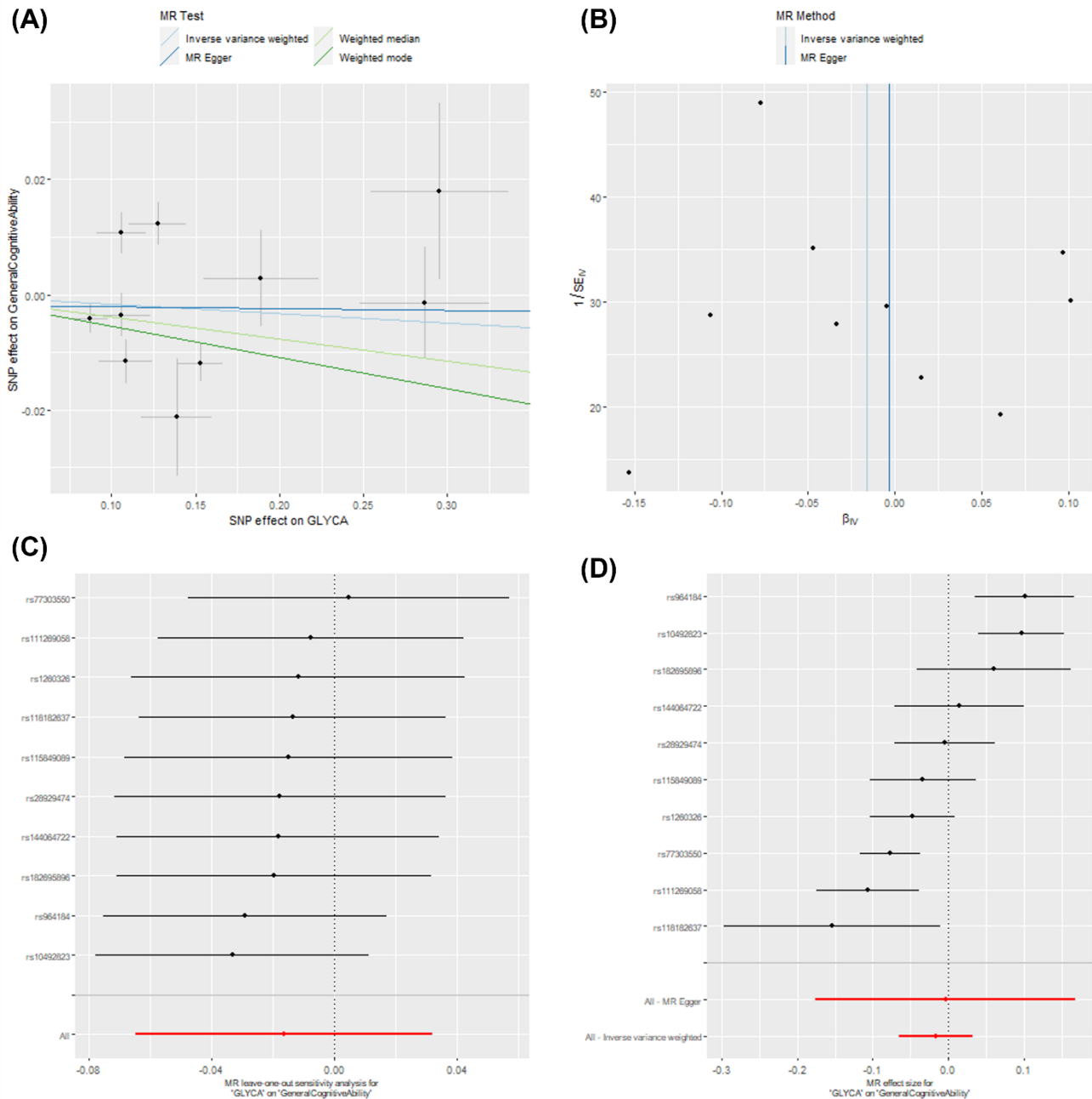
Figure S10. Two-sample MR sensitivity plots: effect of GlycA (Kettunen instrument) on general cognitive ability. Graphs include (A) scatter plot of results from four main MR methods, (B) funnel plot showing each SNP causal estimate against its precision (asymmetry may indicate directional pleiotropy), (C) leave-one-out plot showing inverse-variance weighted estimates after removing each individual SNP in turn, (D) forest plot of causal estimates for each SNP.
