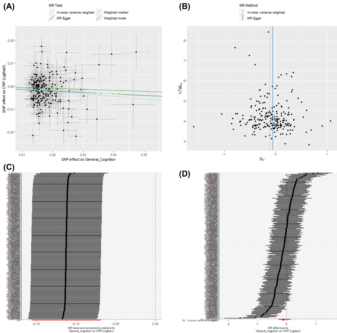
Figure S11. Two-sample MR sensitivity plots: effect of general cognitive ability on CRP (Ligthart et al. GWAS). Graphs include (A) scatter plot of results from four main MR methods, (B) funnel plot showing each SNP causal estimate against its precision (asymmetry may indicate directional pleiotropy), (C) leave-one-out plot showing inverse-variance weighted estimates after removing each individual SNP in turn, (D) forest plot of causal estimates for each SNP.
