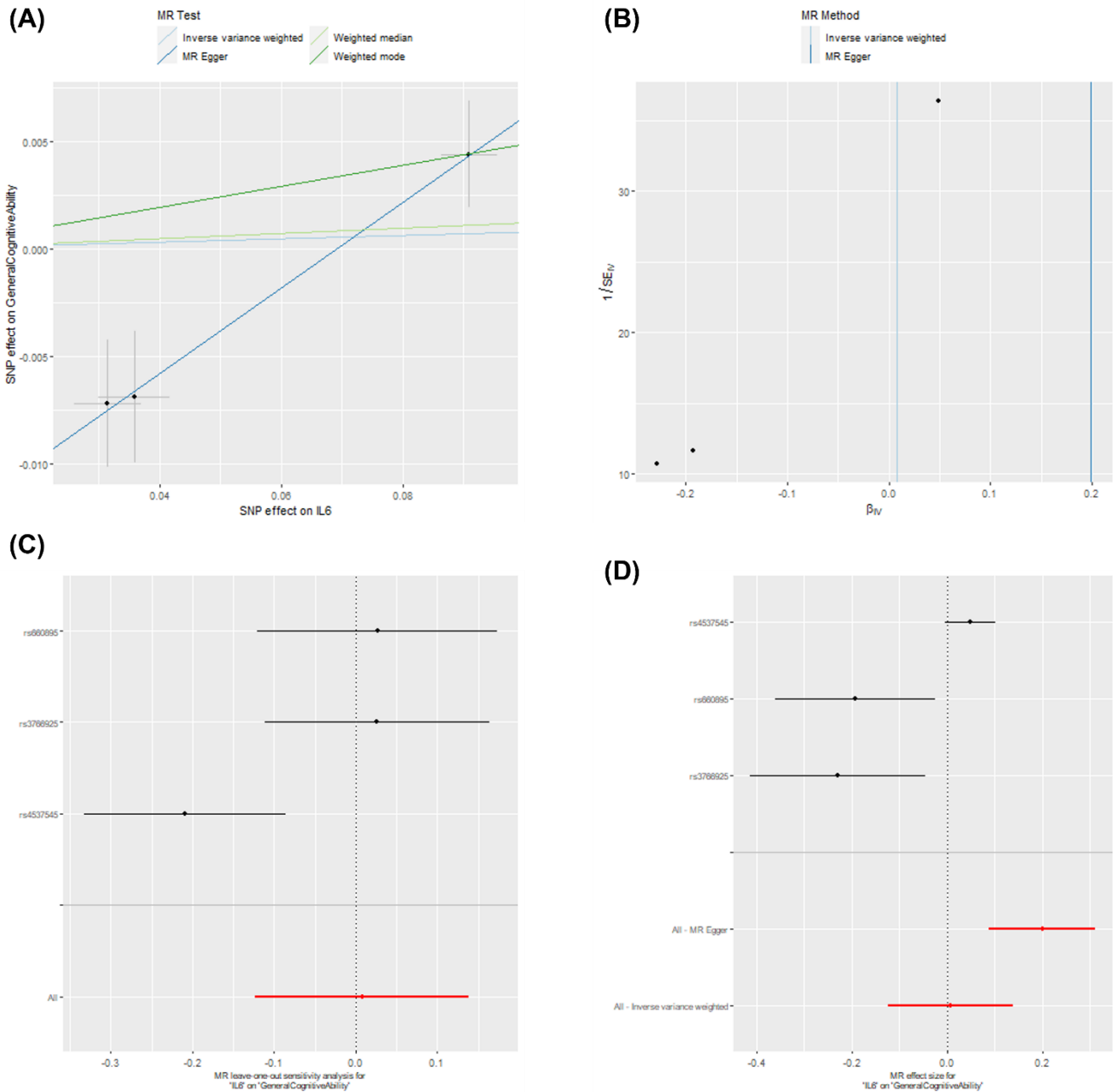
Figure S8. Two-sample MR sensitivity plots: effect of IL-6 (Ahluwalia genome-wide instrument) on general cognitive ability. Graphs include (A) scatter plot of results from four main MR methods, (B) funnel plot showing each SNP causal estimate against its precision (asymmetry may indicate directional pleiotropy), (C) leave-one-out plot showing inverse-variance weighted estimates after removing each individual SNP in turn, (D) forest plot of causal estimates for each SNP.
