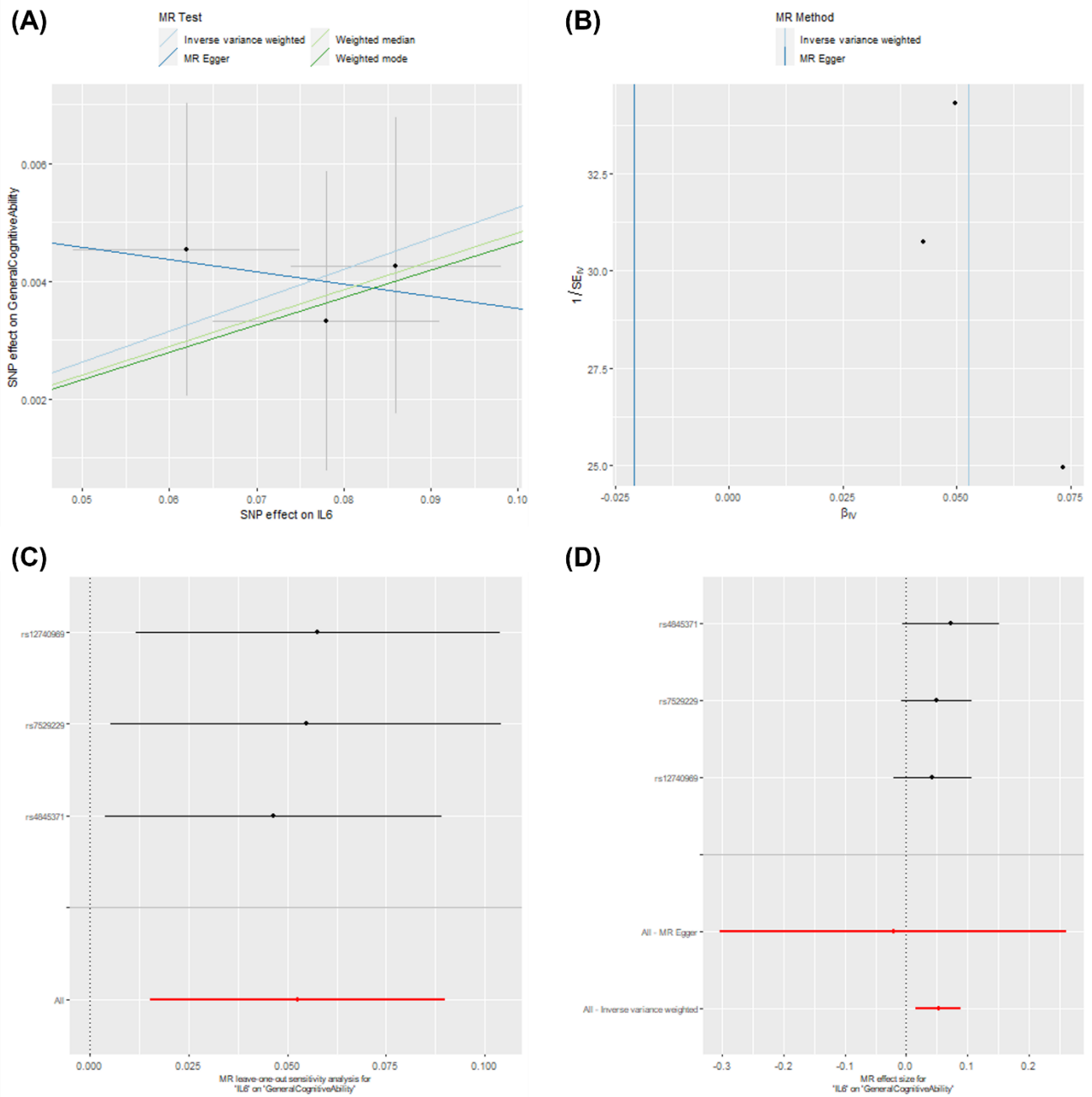
Figure S9. Two-sample MR sensitivity plots: effect of IL-6 (Swerdlow instrument) on general cognitive ability. Graphs include (A) scatter plot of results from four main MR methods, (B) funnel plot showing each SNP causal estimate against its precision (asymmetry may indicate directional pleiotropy), (C) leave-one-out plot showing inverse-variance weighted estimates after removing each individual SNP in turn, (D) forest plot of causal estimates for each SNP.
