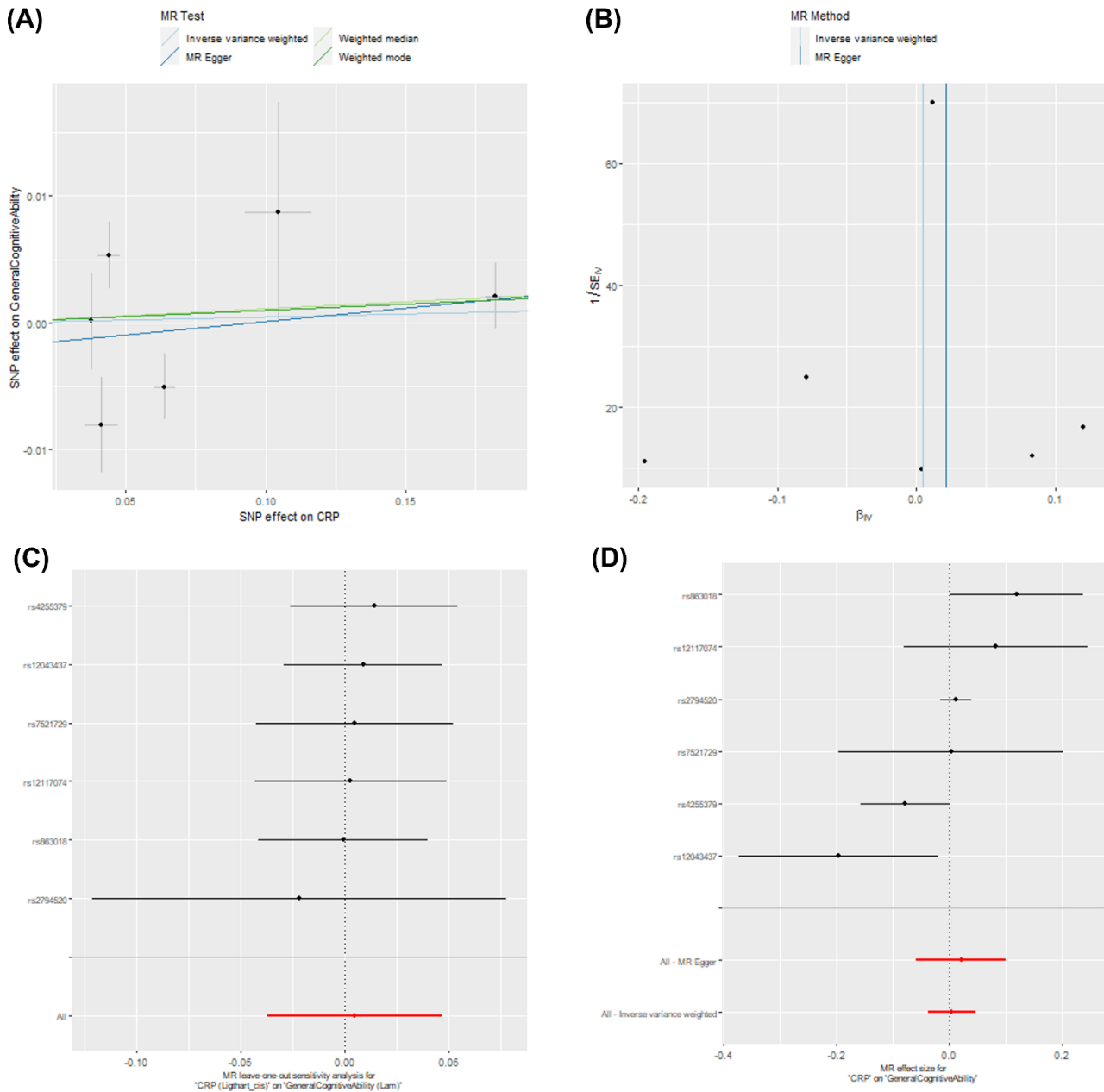
Figure S1. Two-sample MR sensitivity plots: effect of CRP (Lighthart cis instrument) on general cognitive ability. Graphs include (A) scatter plot of results from four main MR methods, (B) funnel plot showing each SNP causal estimate against its precision (asymmetry may indicate directional pleiotropy), (C) leave-one-out plot showing inverse-variance weighted estimates after removing each individual SNP in turn, (D) forest plot of causal estimates for each SNP.
