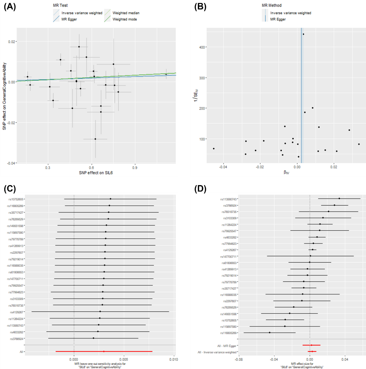
Figure S4. Two-sample MR sensitivity plots: effect of sIL-6R ( Rosa instrument) on general cognitive ability. Graphs include (A) scatter plot of results from four main MR methods, (B) funnel plot showing each SNP causal estimate against its precision (asymmetry may indicate directional pleiotropy), (C) leave-one-out plot showing inverse-variance weighted estimates after removing each individual SNP in turn, (D) forest plot of causal estimates for each SNP.
