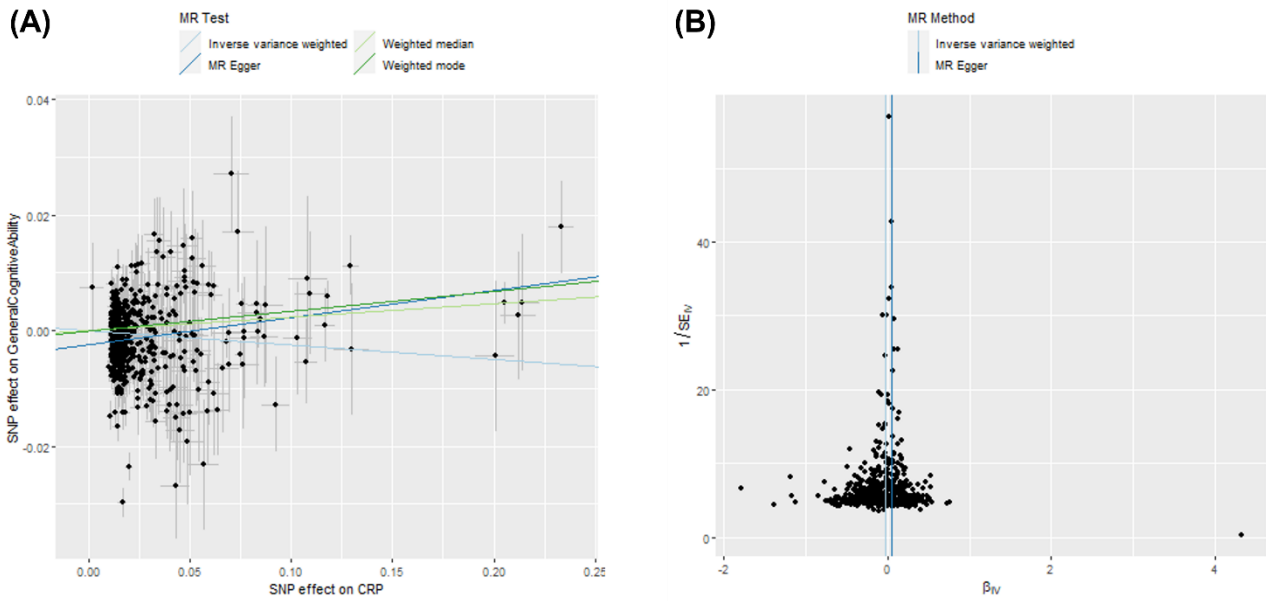
Figure S7. Two-sample MR sensitivity plots: effect of CRP (Han genome-wide instrument) on general cognitive ability. Graphs include (A) scatter plot of results from four main MR methods, (B) funnel plot showing each SNP causal estimate against its precision (asymmetry may indicate directional pleiotropy). Due to a large number of SNPs being used, leave-one-out plot and forest plot are not shown due to poor visibility visualising all SNPs.
