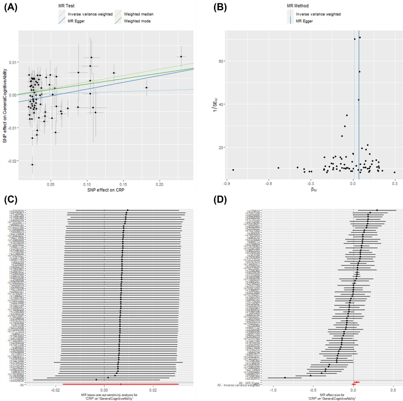
Figure S6. Two-sample MR sensitivity plots: effect of CRP (Ligthart genome-wide instrument) on general cognitive ability. Graphs include (A) scatter plot of results from four main MR methods, (B) funnel plot showing each SNP causal estimate against its precision (asymmetry may indicate directional pleiotropy), (C) leave-one-out plot showing inverse-variance weighted estimates after removing each individual SNP in turn, (D) forest plot of causal estimates for each SNP.
