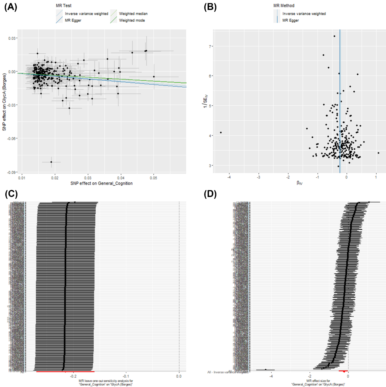
Figure S14. Two-sample MR sensitivity plots: effect of general cognitive ability on GlycA (Borges et al. GWAS). Graphs include (A) scatter plot of results from four main MR methods, (B) funnel plot showing each SNP causal estimate against its precision (asymmetry may indicate directional pleiotropy), (C) leave-one-out plot showing inverse-variance weighted estimates after removing each individual SNP in turn, (D) forest plot of causal estimates for each SNP.
