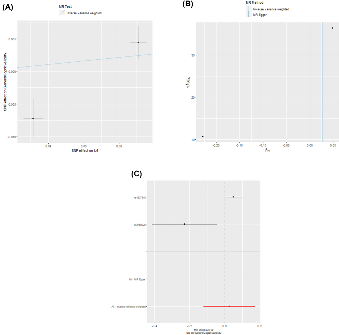
Figure S3. Two-sample MR sensitivity plots: effect of IL-6 ( Ahluwalia cis instrument) on general cognitive ability. Graphs include (A) scatter plot of results from inverse-variance weighted methods, (B) funnel plot showing each SNP causal estimate against its precision (asymmetry may indicate directional pleiotropy), (C) forest plot of causal estimates for each SNP. Leave-one-out plot not shown due to too few SNPs in this instrument.
