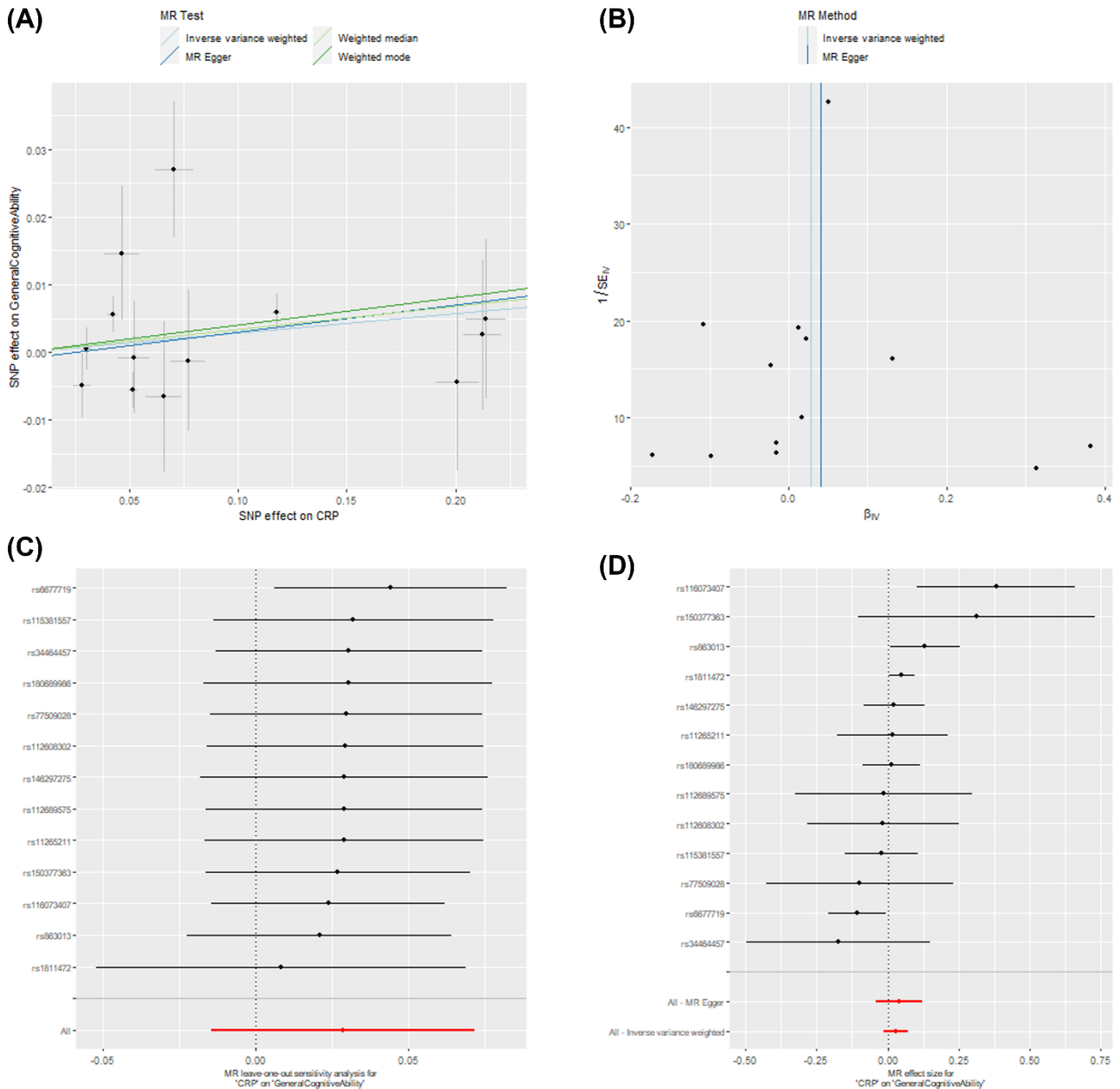
Figure S2. Two-sample MR sensitivity plots: effect of CRP (Han cis instrument) on general cognitive ability. Graphs include (A) scatter plot of results from four main MR methods, (B) funnel plot showing each SNP causal estimate against its precision (asymmetry may indicate directional pleiotropy), (C) leave-one-out plot showing inverse-variance weighted estimates after removing each individual SNP in turn, (D) forest plot of causal estimates for each SNP.
