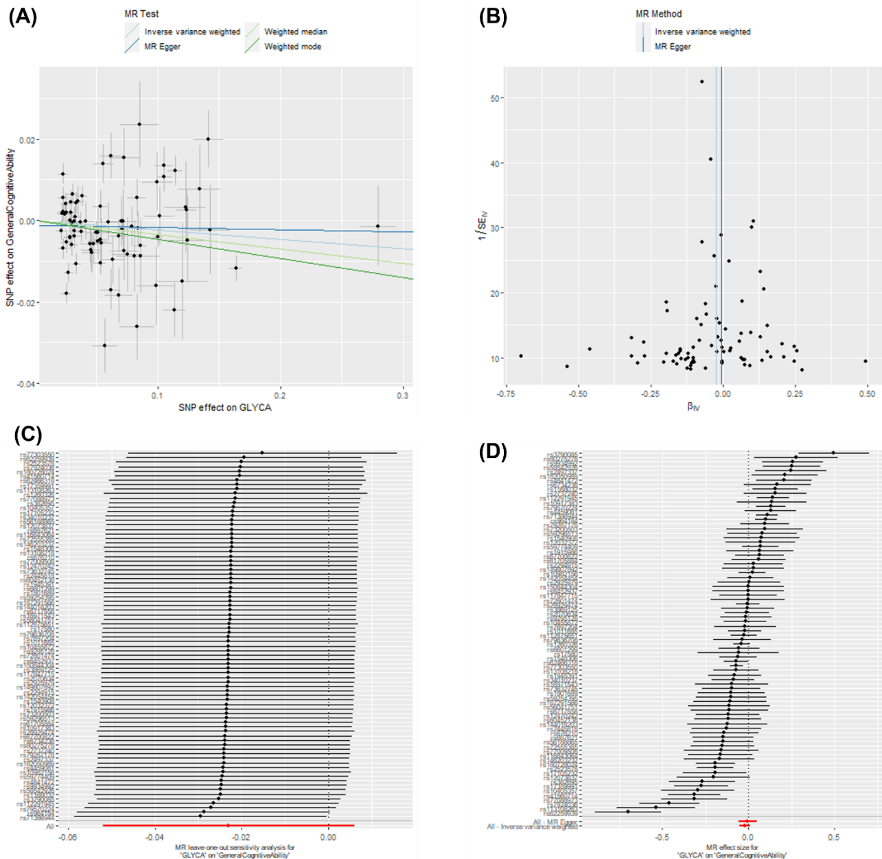
Figure S5. Two-sample MR sensitivity plots: effect of GlycA (Borges instrument) on general cognitive ability. Graphs include (A) scatter plot of results from four main MR methods, (B) funnel plot showing each SNP causal estimate against its precision (asymmetry may indicate directional pleiotropy), (C) leave-one-out plot showing inverse-variance weighted estimates after removing each individual SNP in turn, (D) forest plot of causal estimates for each SNP.
