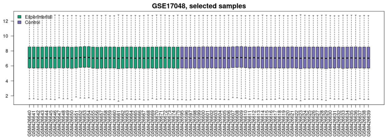
Figure 1: Gene expression value distribution for dataset GSE17048 with each box representing the gene expression values for 1 sample. The green bars correspond to the experimental samples of MS patients while the purple bars correspond to the control samples of the healthy individuals.
