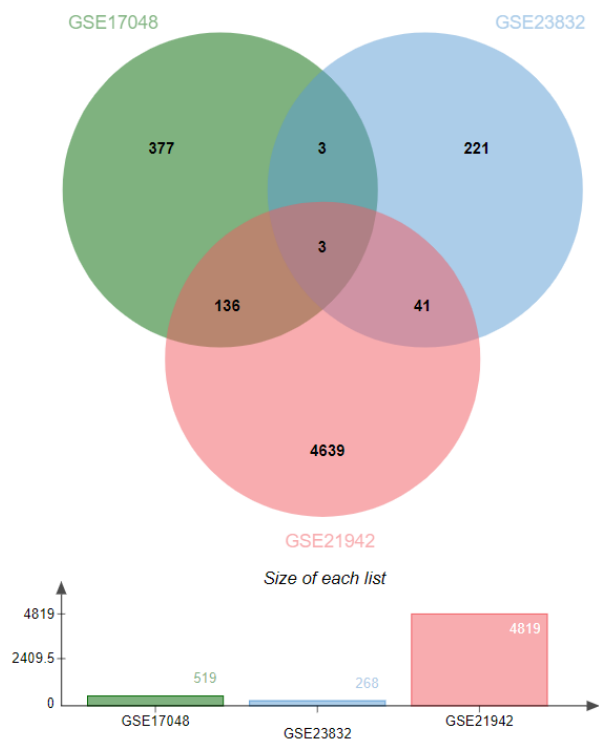
Figure 4: The Venn Diagram depicts the overlap of genes between the 3 datasets. For example, there are 41 genes that are common to GSE23832 and GSE21942.
