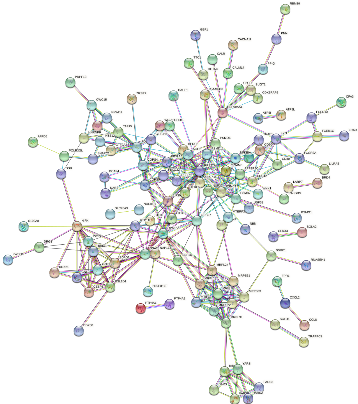
Figure 5: This network generated by STRING displays 164 DEGs as the isolated genes have been omitted. The color of each protein is not of relevance but the lines connecting the nodes indicate how the interaction was determined. For example, the light blue line indicates that information regarding the interaction was already present in the database while the pink line indicates that the interaction was experimentally demonstrated.
