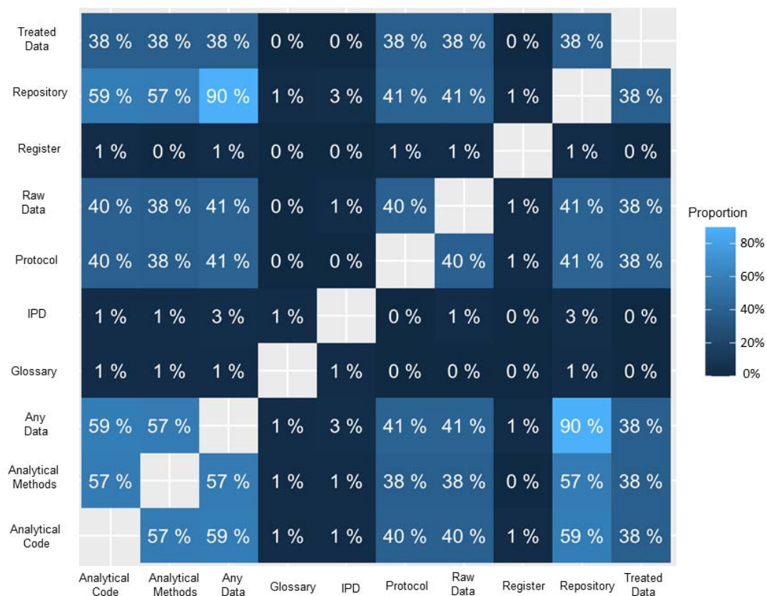
Figure 2. Pairwise cross-tabulation density plot between variables containing guidance herein.
