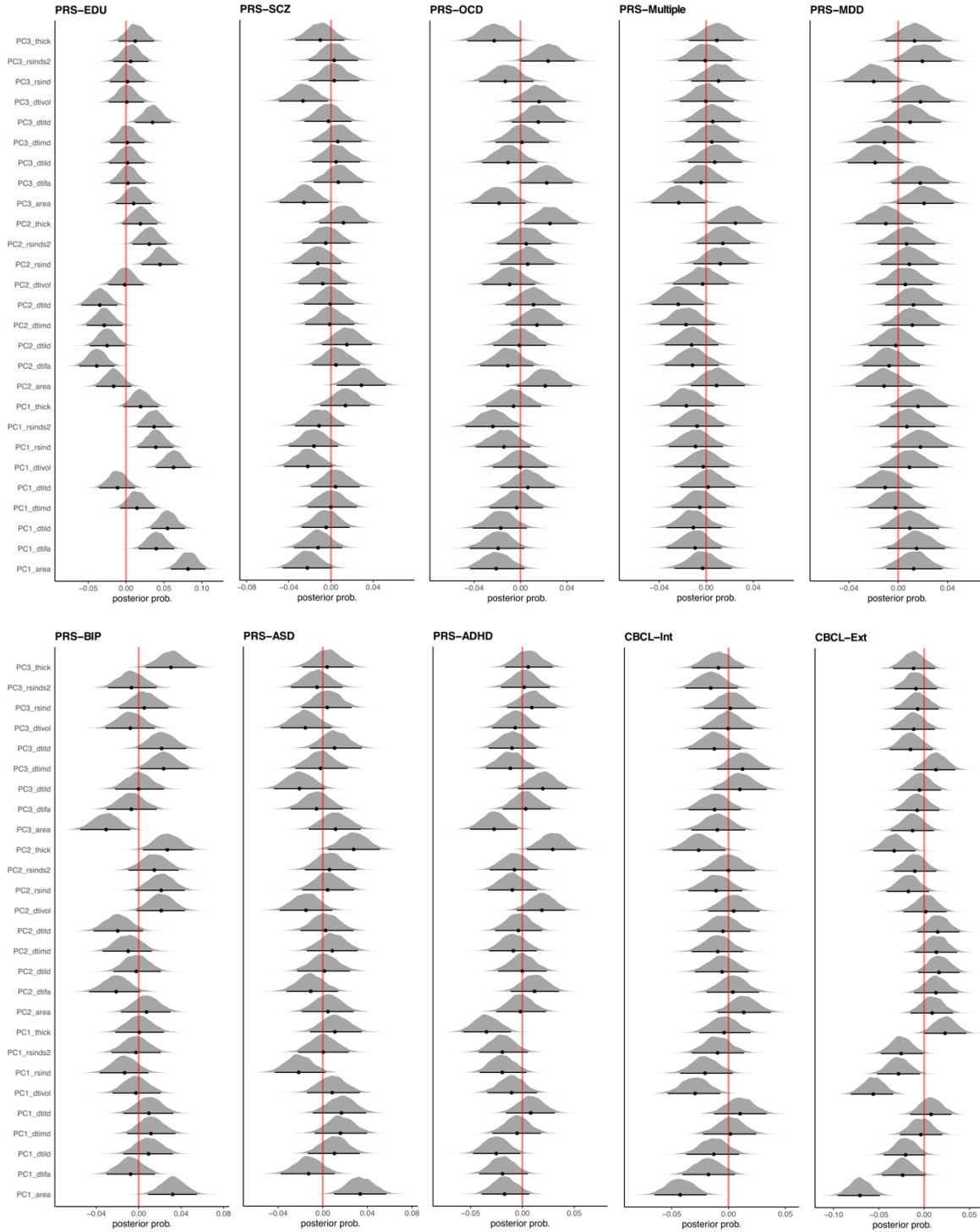
Supplementary Figure 6. Posterior distributions of the univariate Bayesian models examining the relationships between PRS and imaging components. Distributions of the posterior densities. Dots show the mean of the posterior distributions and lines represent the 95% Credible Interval.
