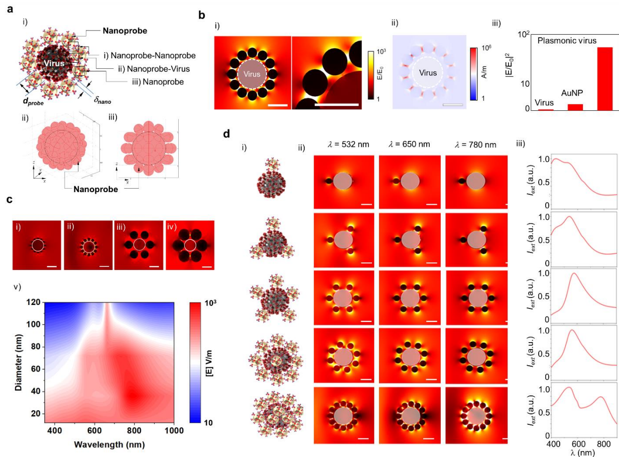
Figure 2. Schematic and characteristics of Plasmonic virus. a) Scheme of a plasmo-virus particle formed of assembled plasmonic nanoprobe with specific size and density leading to plasmonic nanogap on SARS-CoV-2 virus. b) i) E-field and ii) power distribution around a plasmo-virus structure. A highly enhanced E-field is focused on each plasmonic nanogap between assembled plasmonic nanoprobe on the SARS-CoV-2 virus (scale bar = 100 nm) and iii) Comparison of E-field enhancement of virus, AuNP, and plasmo-virus. c) E-field distribution at nanoprobe with different sizes of i) 10, ii) 50, iii) 100, and iv) 150 nm. Heat map of E-field for probe diameter vs. wavelength from \lambda = 350 to 1,000 nm (scale bars = 100 nm). d) Effect of the nanoprobe density around a virus particle on the plasmo-virus particle's optical properties; i)
