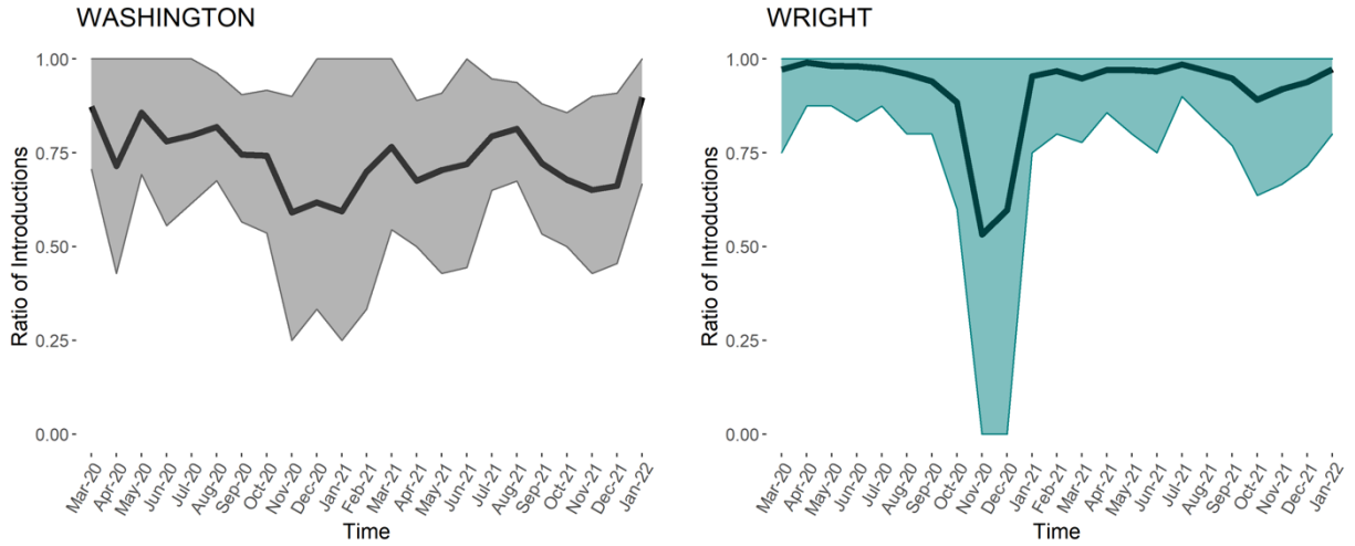
Supplemental Fig. 1. Ratio of introductions to total viral flow into and out of the respective county by month for each county from March 2020 – January 2022. We show the posterior mean ratio and 95% Bayesian highest posterior density interval. Many of the counties contain uncertainty around the median ratio given their limited number of sequences.
