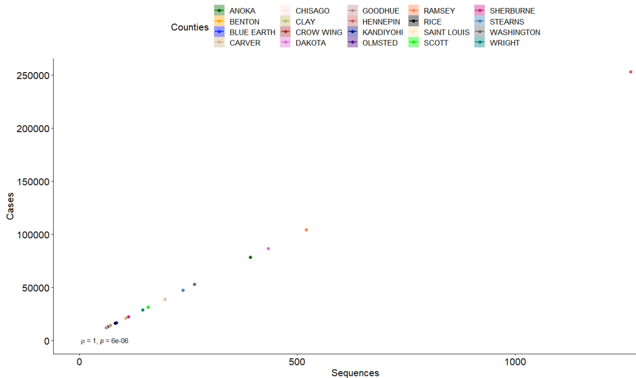
Supplemental Fig. 2. Correlation between subsampled counties sequences and COVID-19 cases. Correlation coefficient via Spearman's Rho ( \rho = 1 ).
