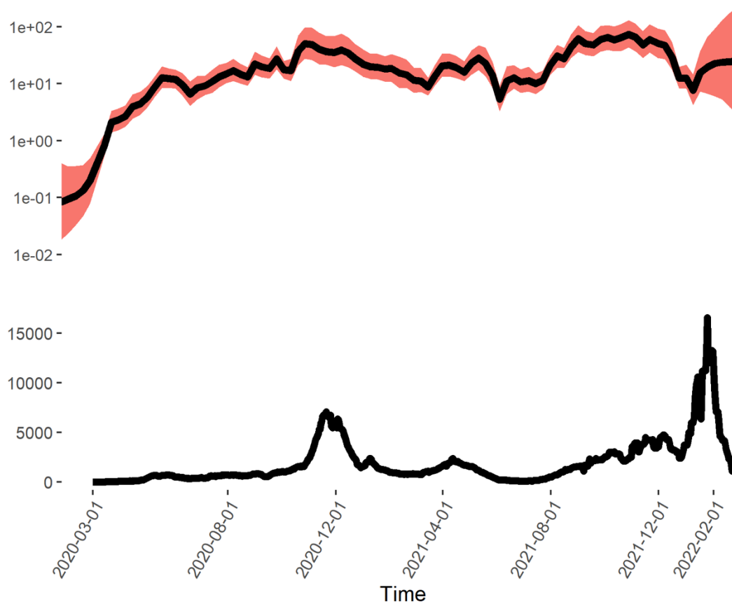
Supplemental Fig. 3. Effective population size of SARS-CoV-2 and confirmed cases in Minnesota. A) Bayesian Skygrid plot of effective population size over time of SARS-CoV-2 in Minnesota. The line represents the median value while the shaded region is the 95% Bayesian highest posterior density region. B) Seven-day rolling average of confirmed cases of COVID-19 in Minnesota 1 .
