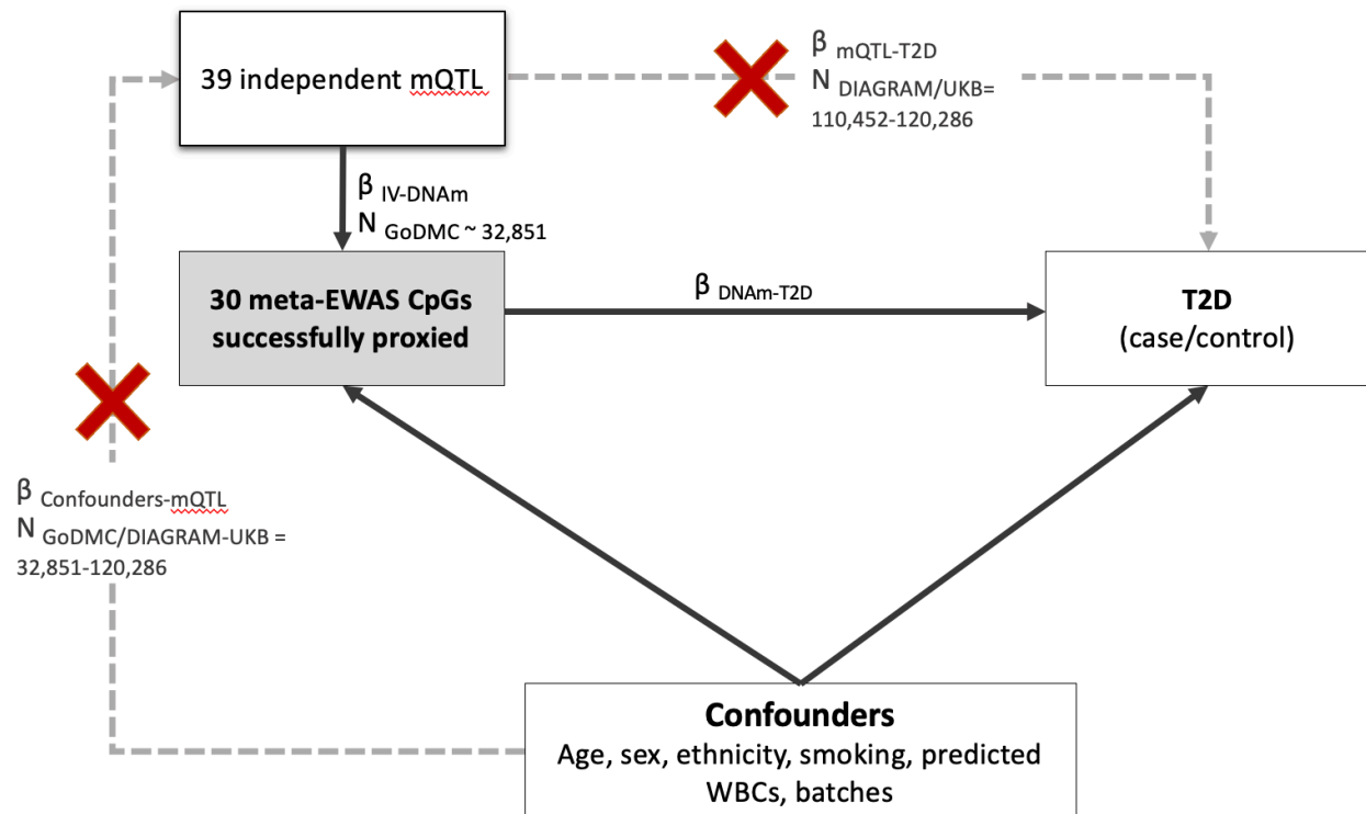
Figure 2. Study design of the reverse two-sample MR (2SMR) investigating the causal effect of differences in DNAm on T2D risk. 58 CpGs were previously identified in association with T2D in a meta-analysis of EWAS (meta-EWAS), but only 30 of them were proxied by a mQTL SNP in GoDMC with available GWAS data for T2D in MR-Base. IV: instrumental variable, PCs: genetic principal components, UKB: UK-Biobank.
