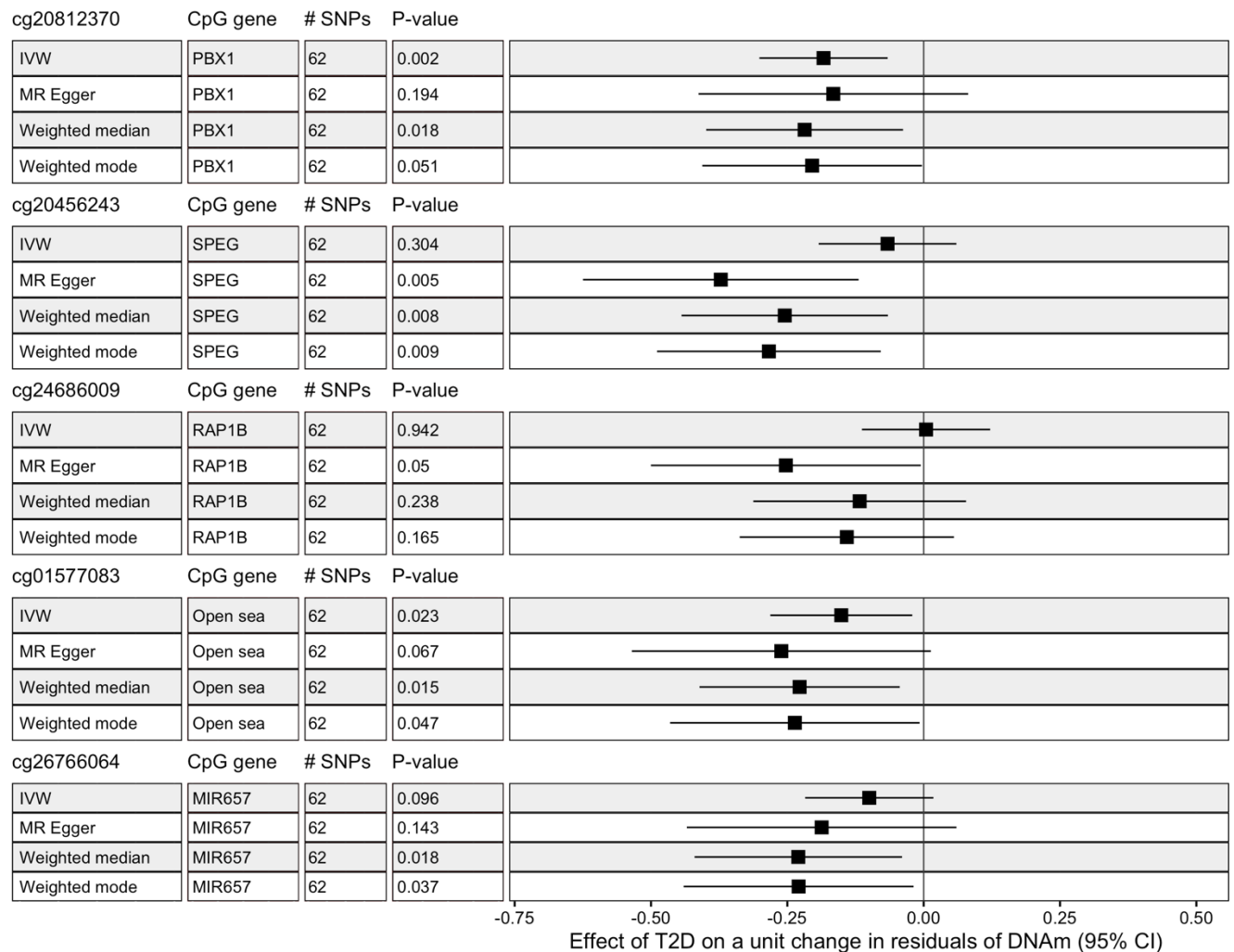
Figure 3 Forest plot showing causal effect estimates from a two-sample MR looking at the effect of prevalent T2D on the difference in DNAm at five meta-EWAS CpGs identified with the strongest evidence of causality in the forward 2SMR. Mean causal effect for each CpG and MR method is represented by the black square, and the line across is the 95% confidence interval. IVW: inverse-variance weighted random effect regression. # SNPs: number of valid single nucleotide polymorphisms used as proxies for T2D in the forward MR analysis. P-value: unadjusted P-value. Associations were borderline significant at unadjusted- P < 0.05 , or significant at adjusted- P < 0.001 .
