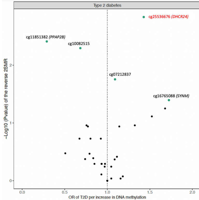
Figure 4 Summarizing evidence of the reverse 2SMR for the association between inverse-normal transformed residuals of DNAm at five meta-EWAS CpGs, and risk of prevalent T2D. CpGs illustrated showed the smallest P-value in the reverse 2SMR. A) Volcano plot showing MR estimates using the Wald ratio and a single SNP as proxy for each CpG analyzed. Highlighted in red is the CpG cg25536676 (DHCR24) identified as causally associated with T2D ( P = 0.001 ). Green dots are CpGs identified with unadjusted P < 0.05 or -\text{Log}_{10}(\text{P-value}) > 1.3 in the 2SMR. Vertical dashed line represents the line of null associations at \text{OR} = 1.0 . B) Forest plot showing mean and standard error of the causal estimates at top five CpGs identified in the reverse 2SMR. Results for each CpG are grouped by the MR method applied, which differed only for the CpG cg25536676 (DHCR24) proxied by 3 mQTL. 2SMR: Two-sample Mendelian randomization.
