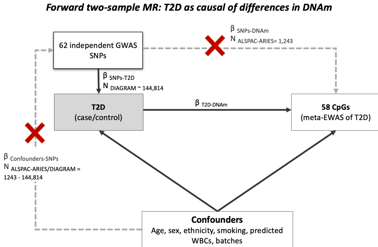
Figure 1. Study design of the forward two-sample MR (2SMR) investigating the causal effect of T2D on differences in DNAm at 58 CpG sites. CpGs were previously identified in association with T2D in a meta-analysis of EWAS (meta-EWAS). IV: instrumental variable, WBC: white-blood cells.
