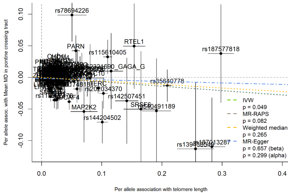
eFigure 59. SNP-mean MD in pontine crossing tract association plotted against SNP-telomere length association, labelled by the mapped gene, with MR slope estimates shown
