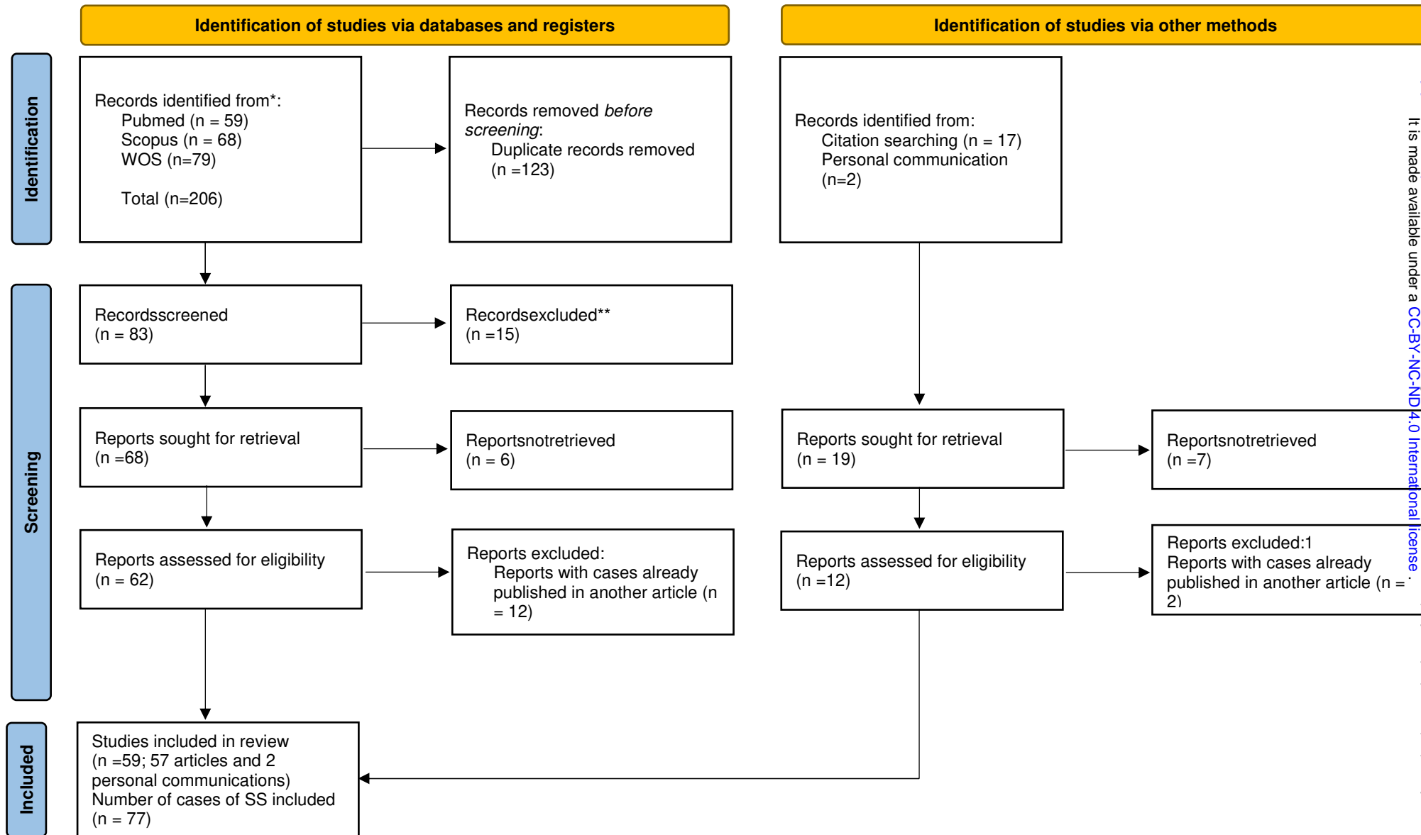
Figure 1: PRISMA 2020 flowdiagram [8]
