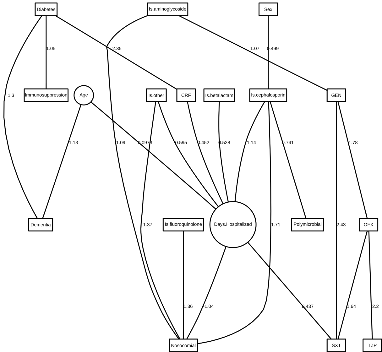
Figure S4: Final DAG for K pneumoniae in urine.
