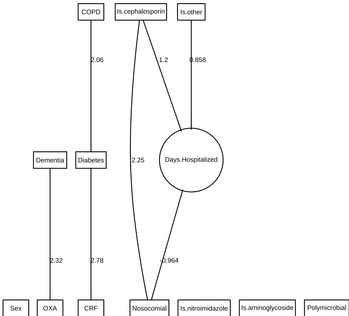
Figure S14: Final DAG for S aureus in aerobic blood.
