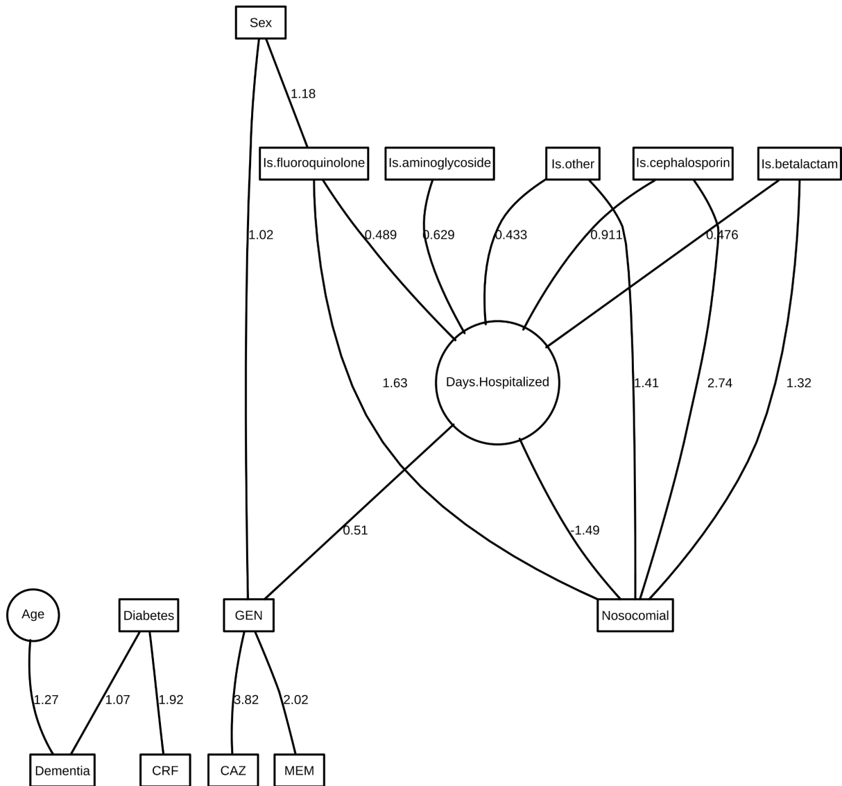
Figure S7: Final DAG for P aeruginosa in urine.
