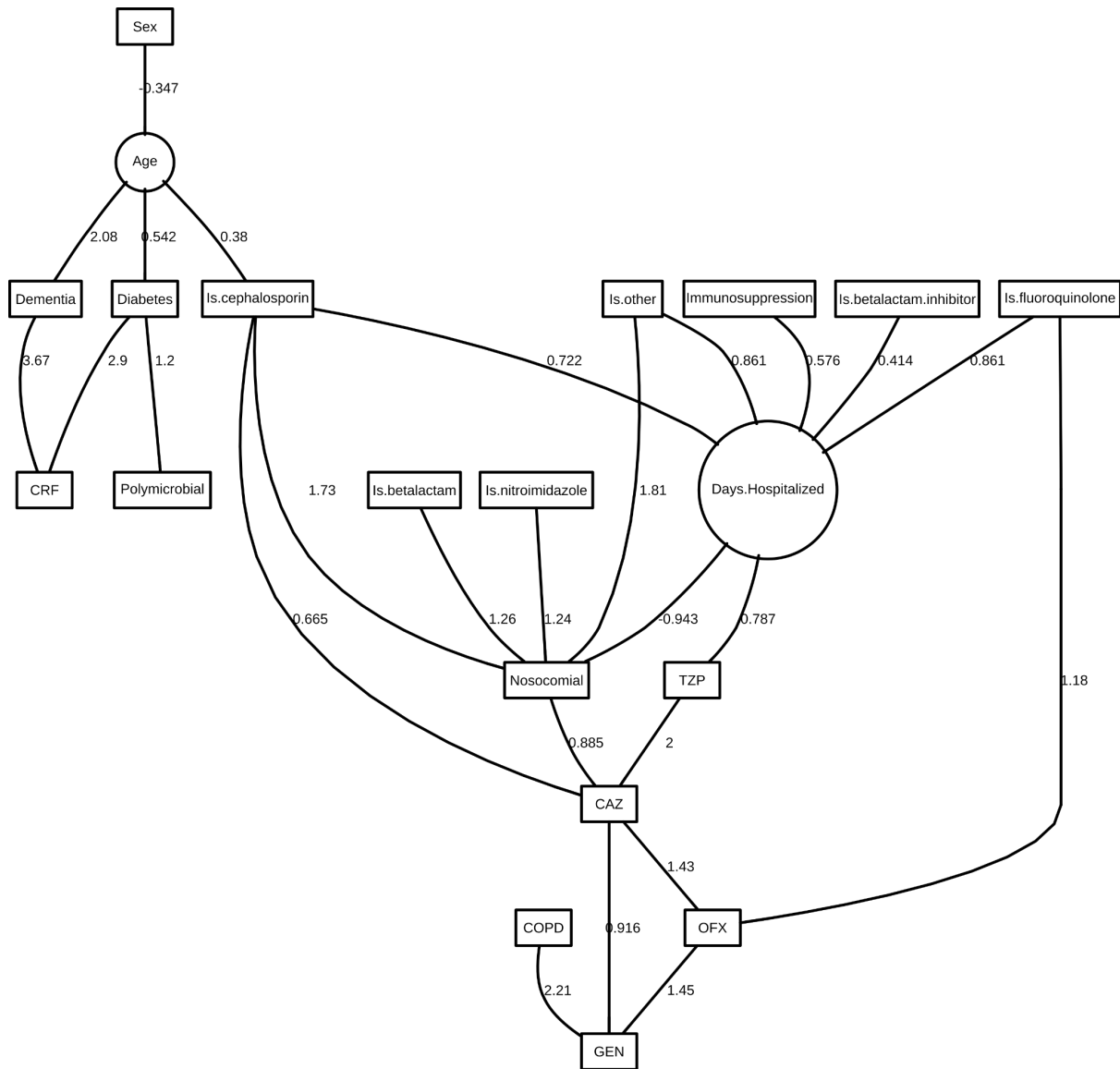
Figure S2: Final DAG for E coli in wound.
