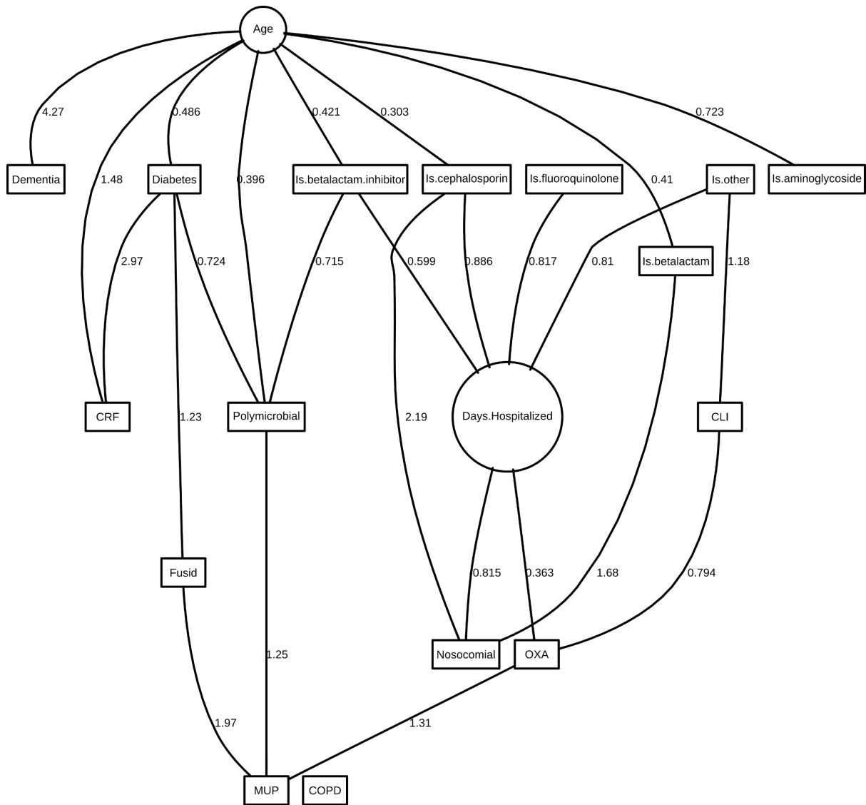
Figure S13: Final DAG for S. aureus in wound.
