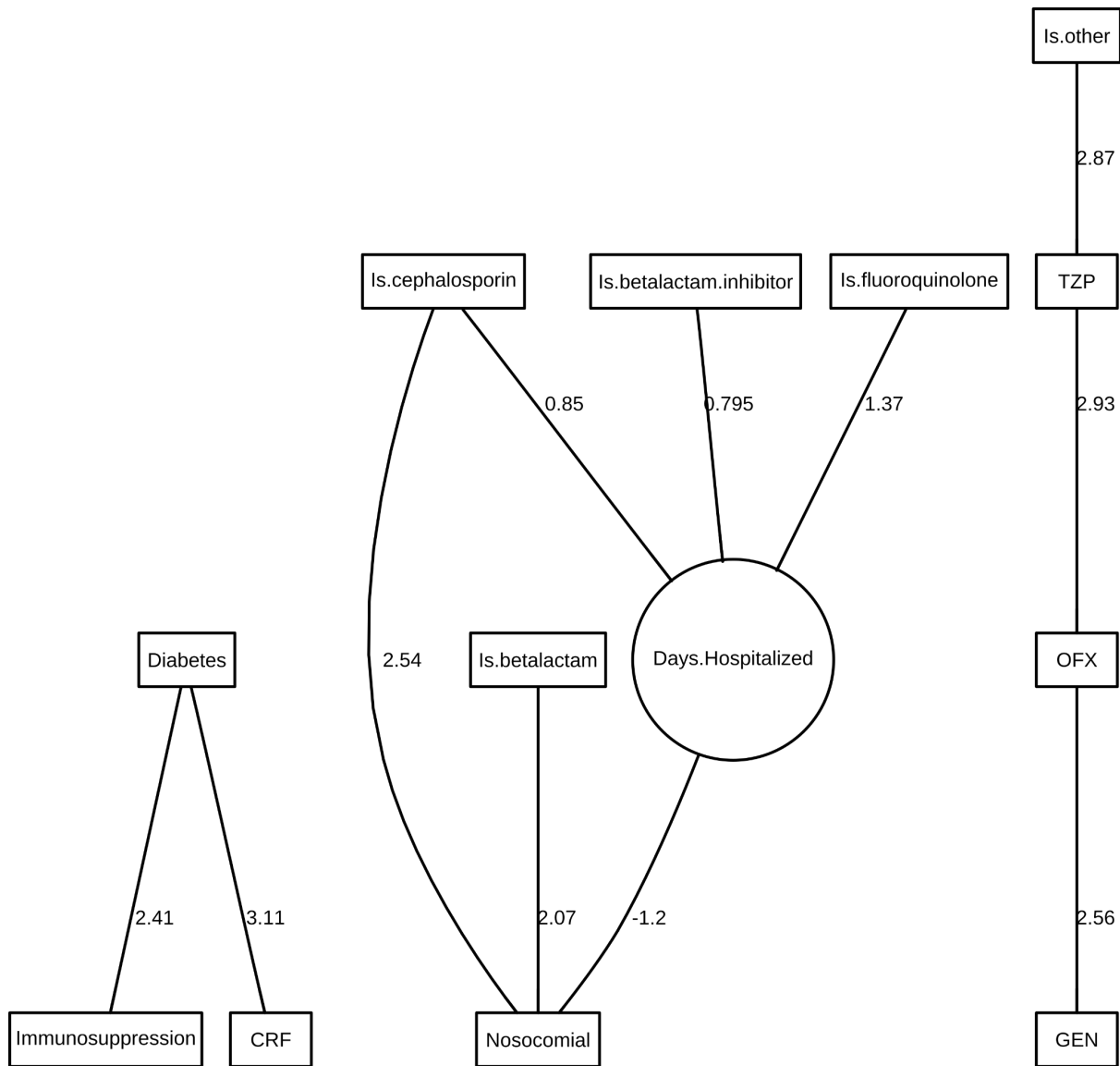
Figure S5: Final DAG for K pneumoniae in wound.
