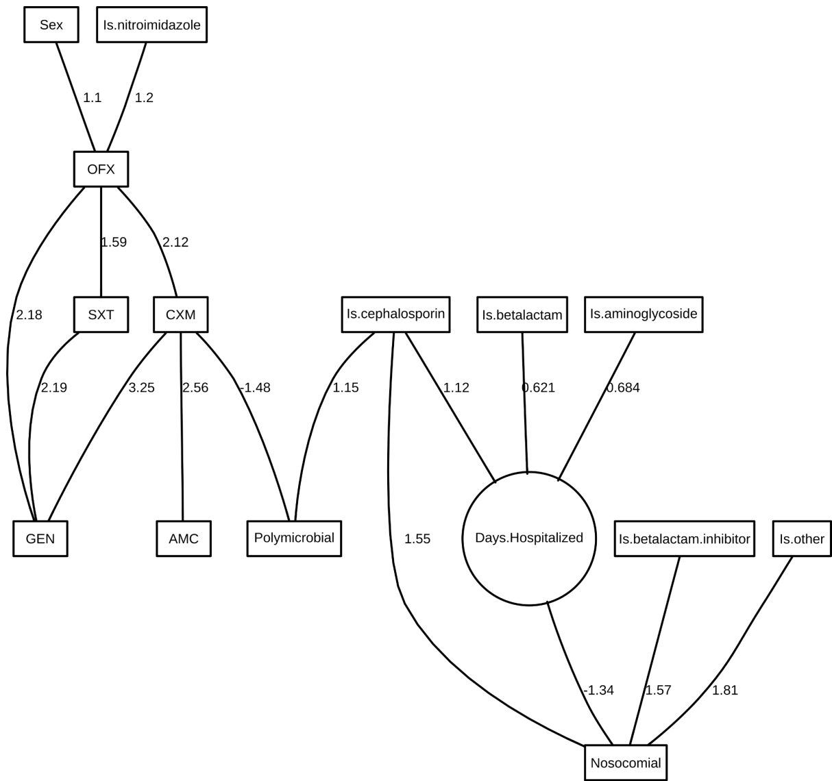
Figure S10: Final DAG for P mirabilis in urine.
