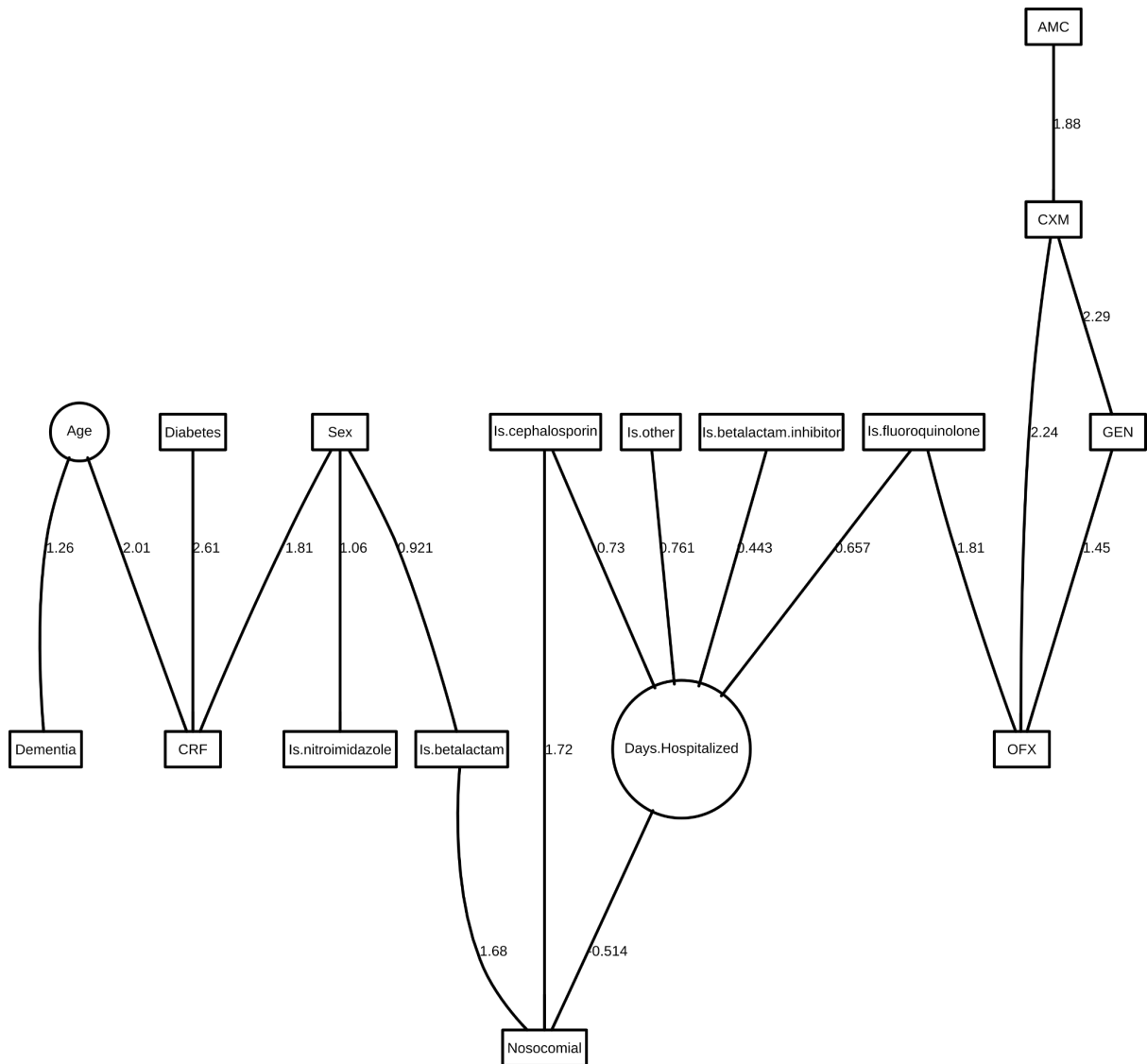
Figure S11: Final DAG for P mirabilis in wound.
