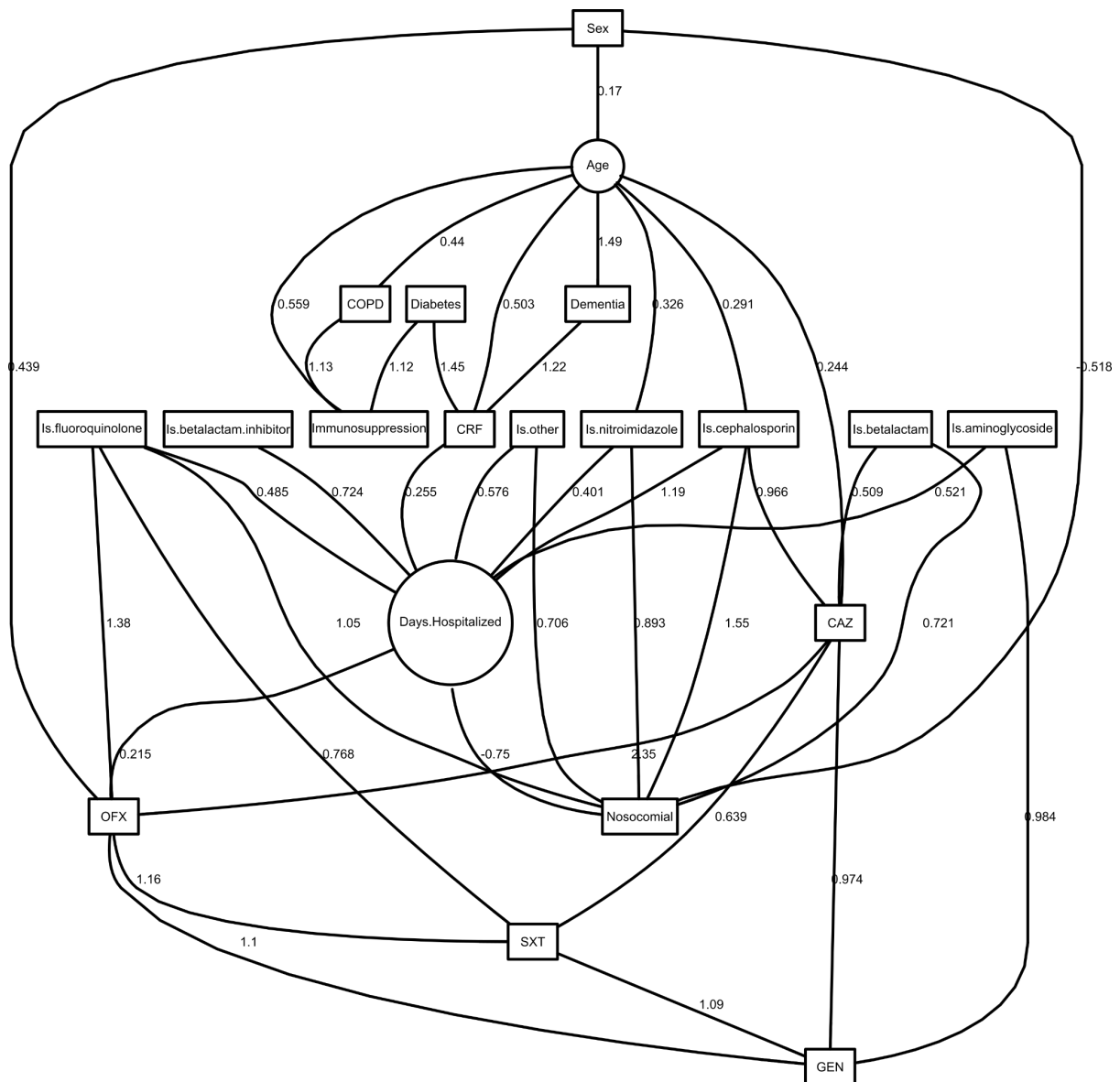
Figure S1: Final DAG for E coli in urine.
