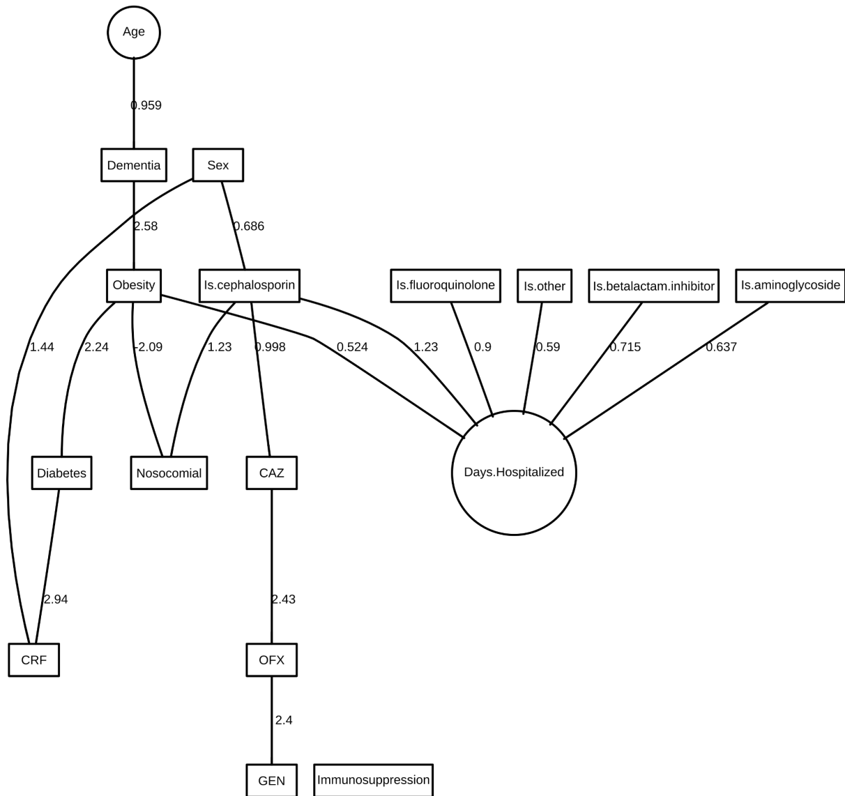
Figure S3: Final DAG for E coli in aerobic blood.
