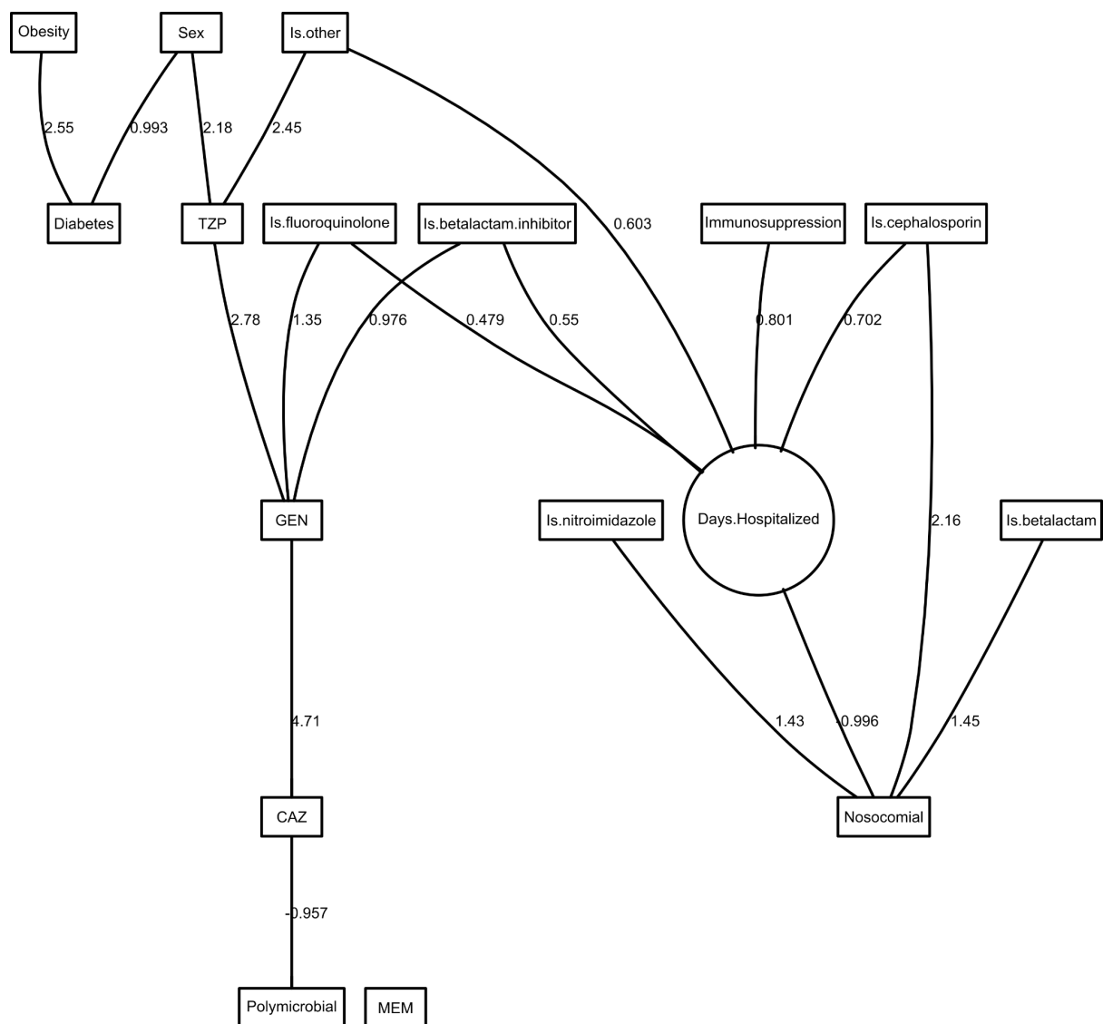
Figure S8: Final DAG for P aeruginosa in wound.
