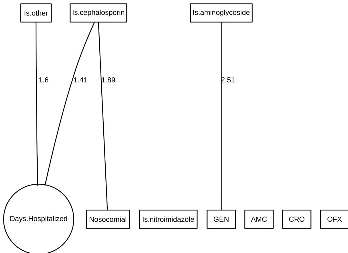
Figure S12: Final DAG for P mirabilis in aerobic blood.
