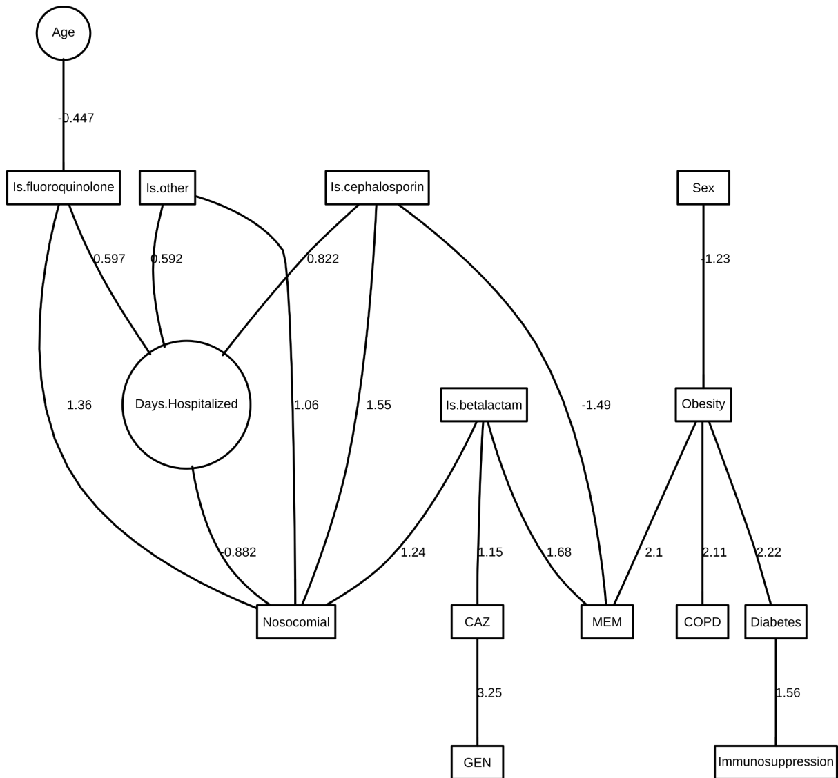
Figure S9: Final DAG for P aeruginosa in sputum.
