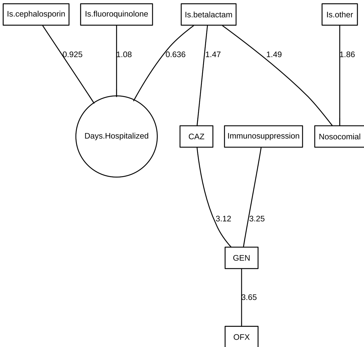
Figure S6: Final DAG for K pneumoniae in aerobic blood.
