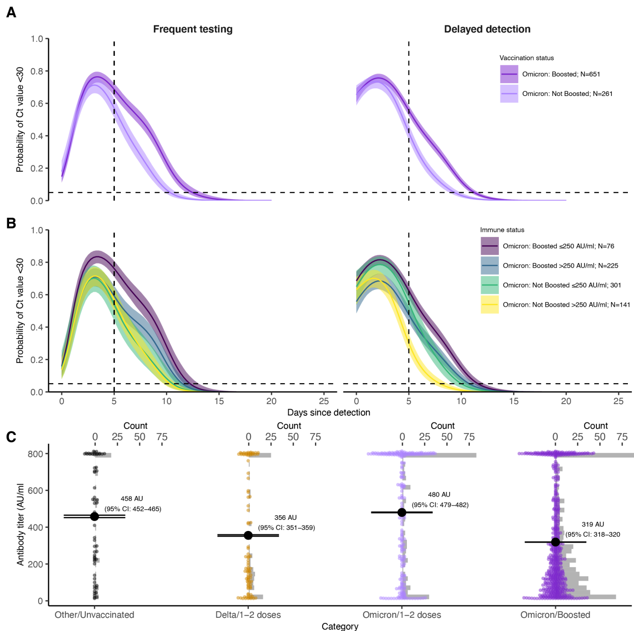
200 201 Figure 2. (A) Proportion of confirmed and suspected Omicron BA.1 infections with Ct<30 on each day post 202 detection by vaccination status and detection group. Solid colored lines and shaded ribbons depict posterior 203 estimates from a generalized linear model predicting probability of Ct<30 as a function of days since detec- 204 tion, vaccination status and variant, showing the posterior mean (solid line) and 95% credible intervals 205 (shaded ribbon) of each conditional effect. Dotted horizontal and vertical lines mark 5% probability and day 206 5 post detection, respectively. (B) As in (A), but additionally stratified by single point-in-time anti-spike 207 antibody titer against the ancestral SARS-CoV-2 (WA1) strain as measured by the Diasorin Trimeric Assay. 208 (C) Distribution of antibody titers (colored points) stratified by variant and vaccination status of each de- 209 tected infection, with mean titers (large black points) and bootstrapped 95% confidence intervals for the 210 mean (horizontal lines). Grey bars are histograms of antibody titer counts in bins of 10 arbitrary units 211 (AU)/ml. Note that stratification is by infection and not individual, and that antibody titers were measured at 212 a single point in time rather than near the time of infection. The Diasorin Trimeric Assay values are truncated 213 between 13 and 800 AU/ml.
