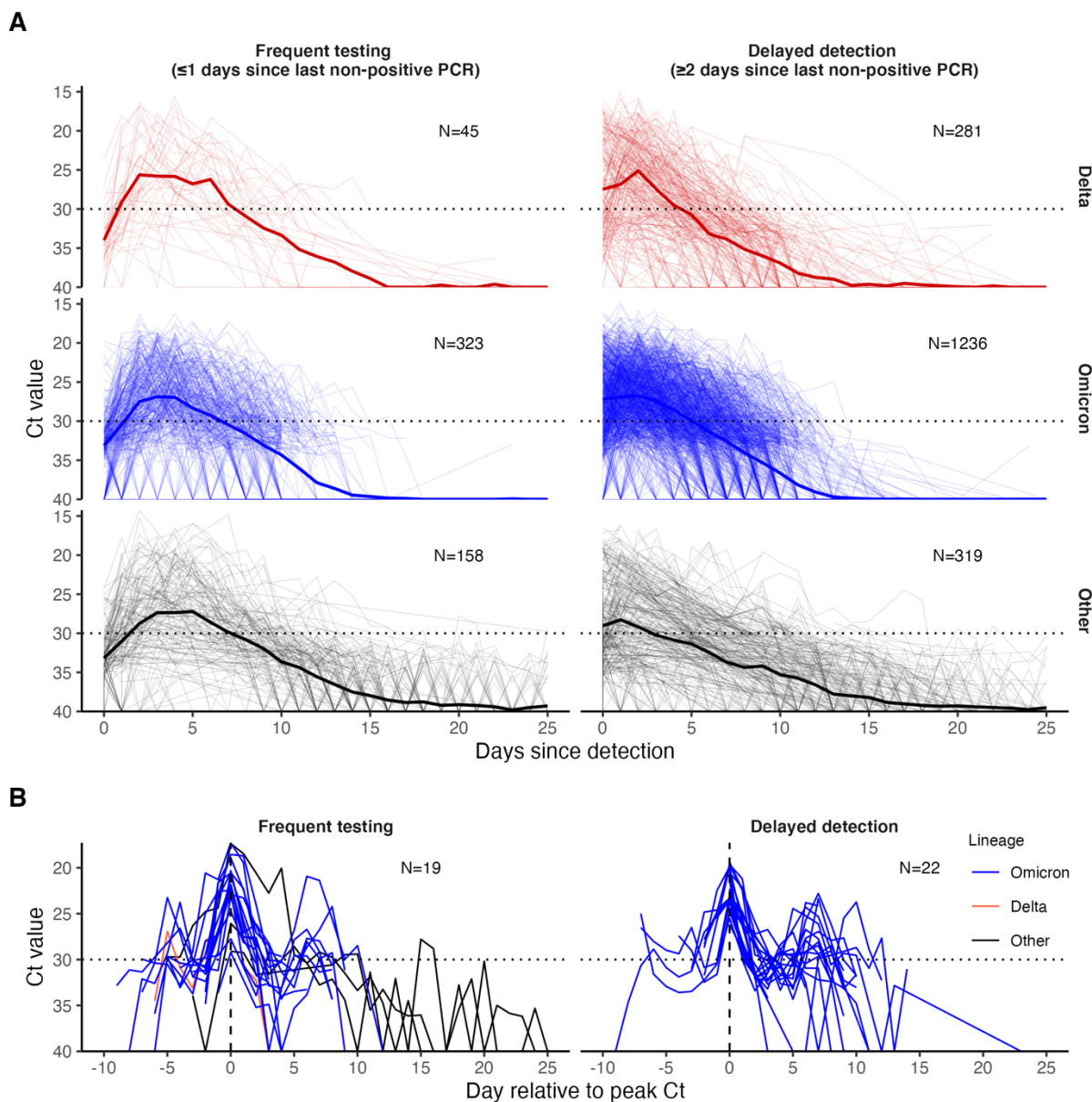
147 148 Figure 1. PCR Ct value trajectories for confirmed and suspected infections. (A) PCR Ct value trajec- 149 tories for each acute Delta (red), Omicron BA.1 (blue), and other (black) infection. Individuals are grouped 150 by the gap between detection and their most recent negative or inconclusive PCR test (Frequent testing 151 vs. Delayed detection). Thick lines depict the mean Ct value over time, counting negative tests as Ct=40. 152 Thin lines depict individual level Ct values over time. The horizontal dotted lines mark Ct=30, which we 153 consider here as a proxy for possible infectiousness and antigen test positivity. (B) Subsets of PCR Ct 154 value trajectories that were classified as rebounds, stratified by testing frequency group. Rebounds are 155 defined here as any trajectory with an initial Ct value <30, followed by a sequence of two or more consec- 156 utive negative tests or tests with Ct value \geq 30 , and subsequently followed by two or more consecutive tests 157 with Ct value <30.
