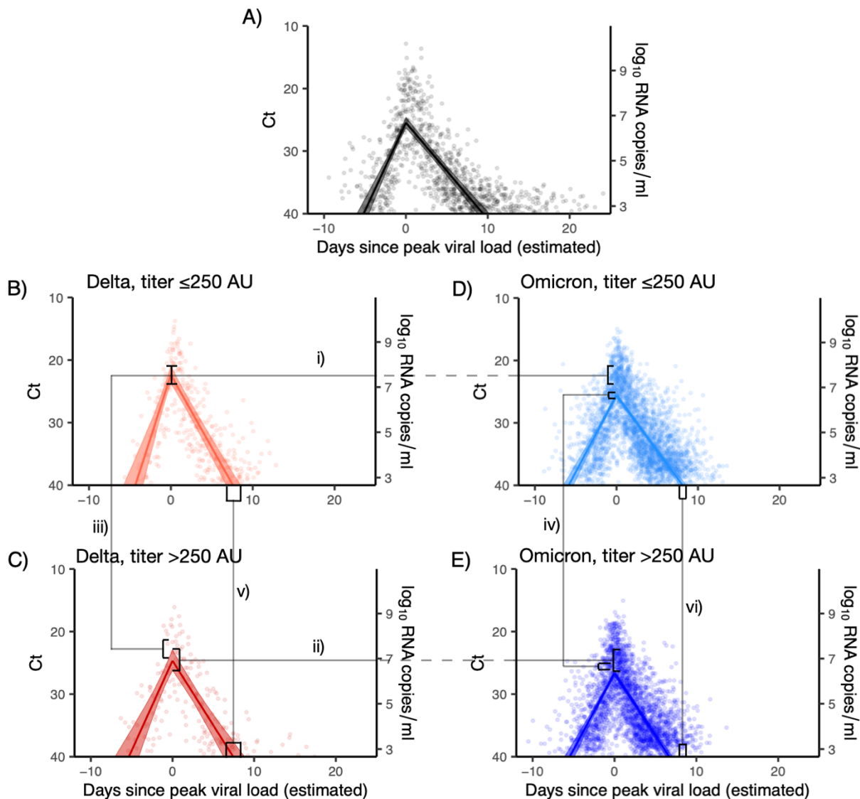
286 287 Figure 3. Estimated viral trajectories by variant and titer. Points depict measured Ct values, lines depict 288 the estimated population mean viral trajectories, and shaded regions depict the 95% credible intervals for 289 the estimated population viral trajectories. A) Non-Delta and non-Omicron infections in individuals who were 290 previously unexposed (no prior record of vaccination or infection), B) Delta infections with titer ≤ 250, C) 291 Delta infections with titer > 250, D) Omicron infections with titer ≤ 250, E) Omicron infections with titer > 292 250. Peak viral loads were higher for Delta infections than for Omicron infections when stratifying by titer (i 293 and ii), and titers ≤ 250 were associated with higher viral loads when stratifying by variant (iii and iv). Low 294 titers were also associated with longer clearance times (v and vi).
