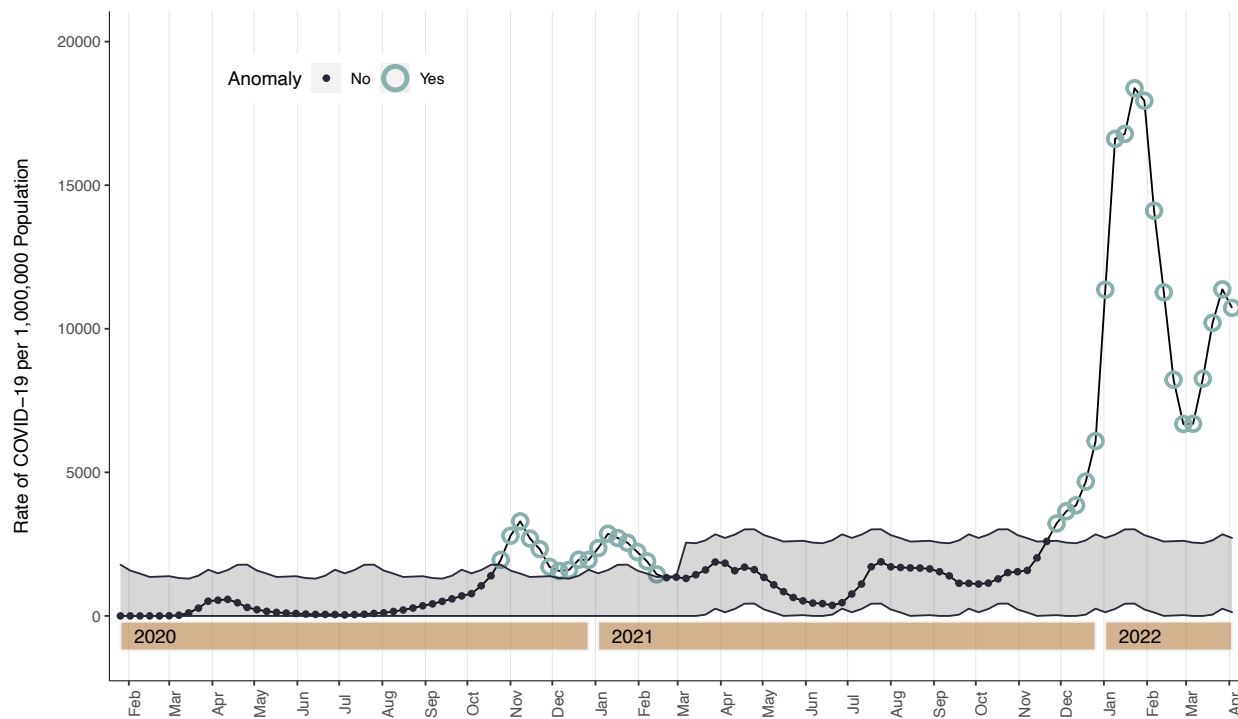
Figure s12. Twitter time series decomposition with generalized extreme studentized deviate (GESD) anomaly detection of EU-5 Country COVID-19 case rates, Mar 7, 2020 – Apr 9, 2022, with 50% maximum anomalies, Data Source: OWID
