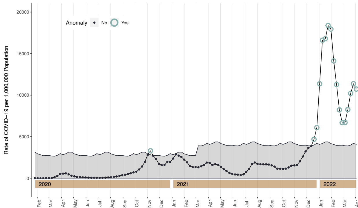
Figure s4. Twitter time series decomposition with generalized extreme studentized deviate (GESD) anomaly detection of EU-5 Country COVID-19 case rates, Mar 7, 2020 – Apr 9, 2022, with 5% maximum anomalies, Data Source: OWID
