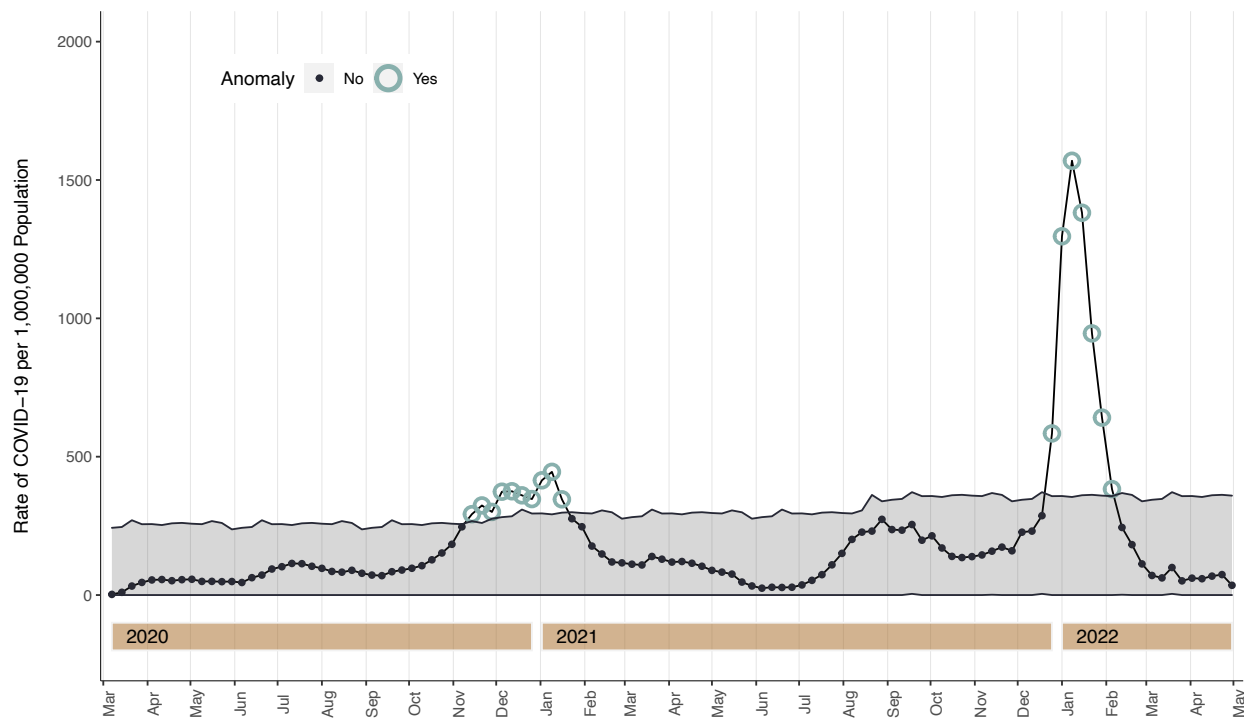
Figure s13. Twitter time series decomposition with generalized extreme studentized deviate (GESD) anomaly detection of US COVID-19 case rates, Mar 7, 2020 – Apr 9, 2022, with 30% maximum anomalies, Data Source: US CDC
