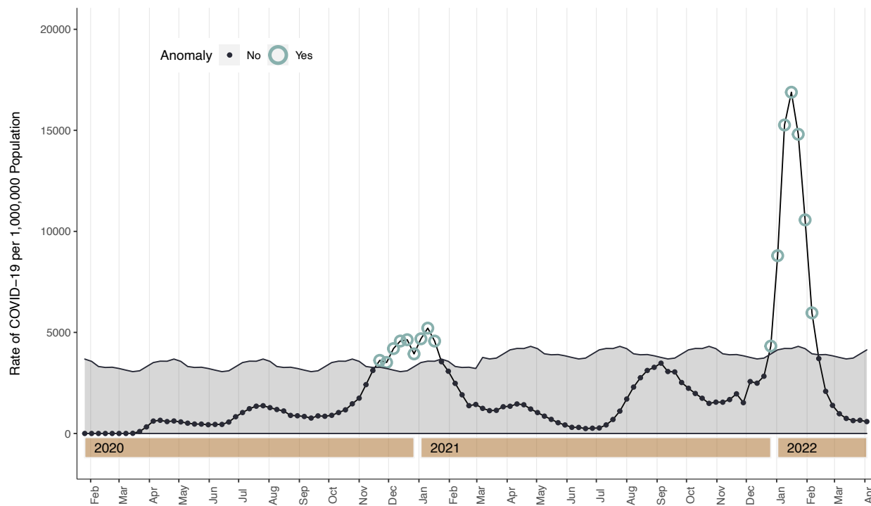
Figure s11. Twitter time series decomposition with generalized extreme studentized deviate (GESD) anomaly detection of US COVID-19 case rates, Mar 7, 2020 – Apr 9, 2022, with 50% maximum anomalies, Data Source: OWID
