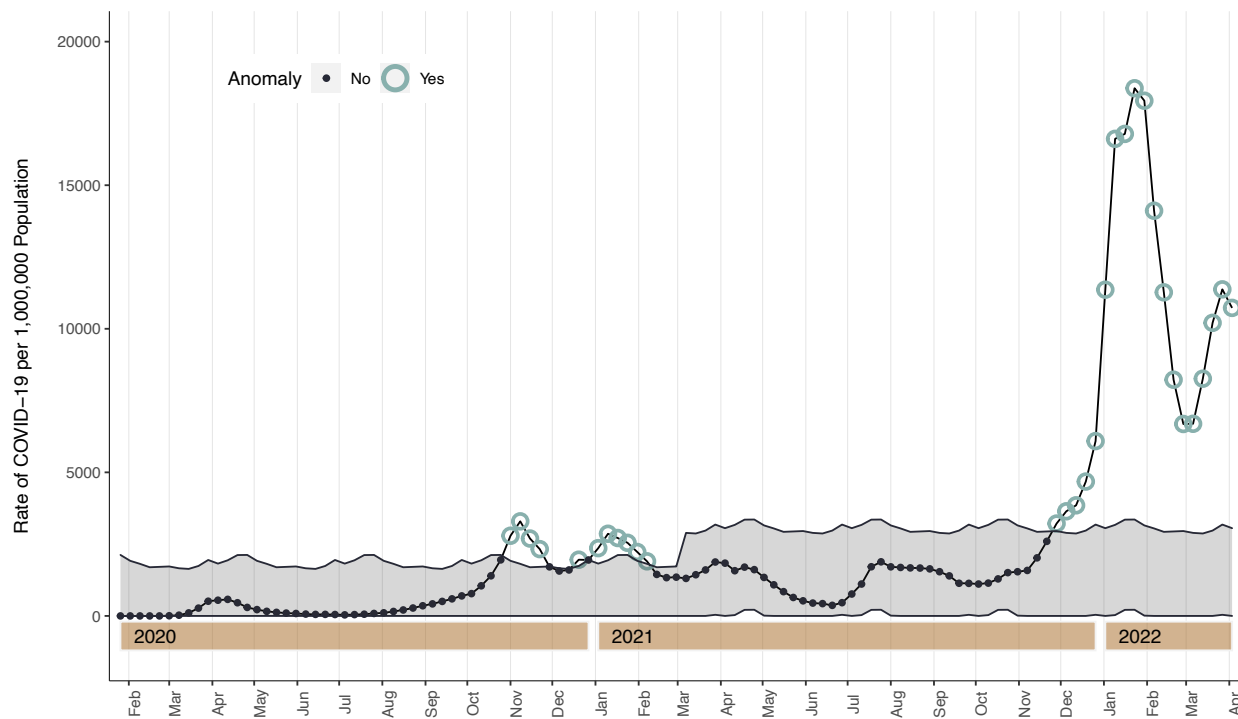
Figure s8. Twitter time series decomposition with generalized extreme studentized deviate (GESD) anomaly detection of EU-5 Country COVID-19 case rates, Mar 7, 2020 – Apr 9, 2022, with 20% maximum anomalies, Data Source: OWID
