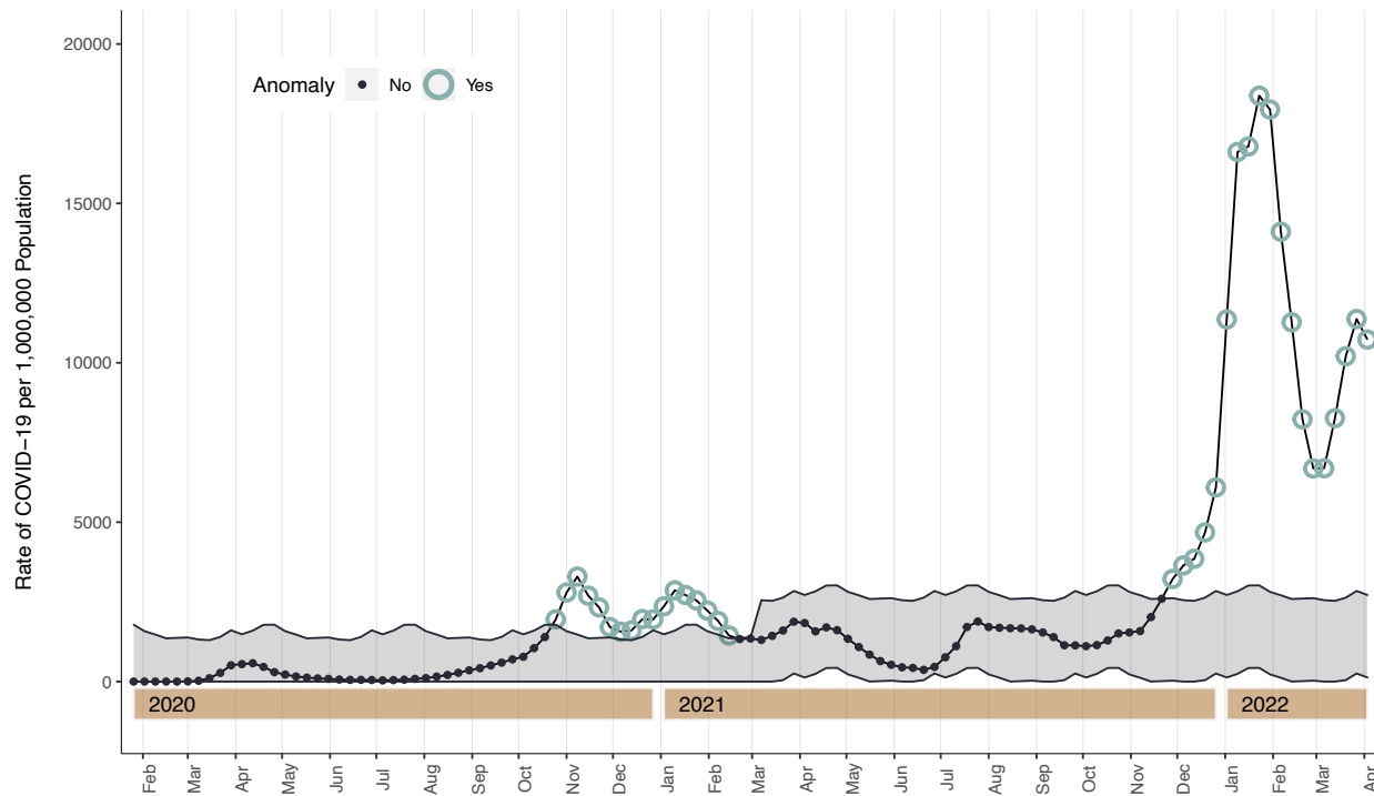
Figure s10. Twitter time series decomposition with generalized extreme studentized deviate (GESD) anomaly detection of EU-5 Country COVID-19 case rates, Mar 7, 2020 – Apr 9, 2022, with 40% maximum anomalies, Data Source: OWID
