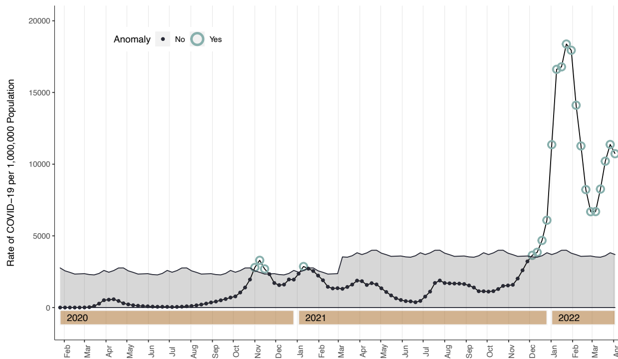
Figure s6. Twitter time series decomposition with generalized extreme studentized deviate (GESD) anomaly detection of EU-5 Country COVID-19 case rates, Mar 7, 2020 – Apr 9, 2022, with 10% maximum anomalies, Data Source: OWID
