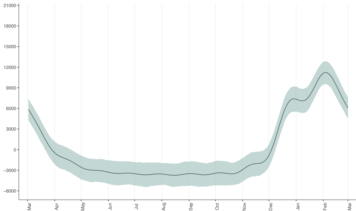
Figure s14. Seasonal component of Influenza cases from the Prophet decomposed model with Markov chain Monte Carlo Simulated 95% uncertainty intervals, Mar 1, 2014 – Apr 10, 2020, holiday-adjusted, United States. Data Source: US CDC
