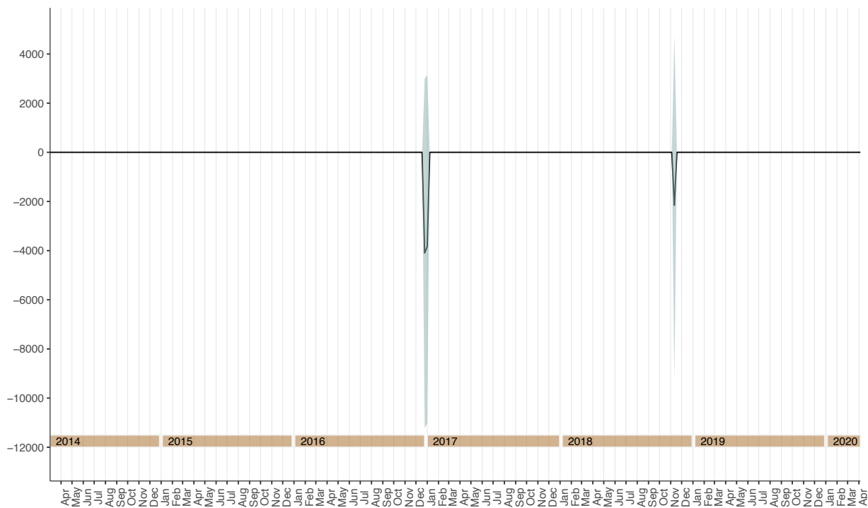
Figure s15. Holiday component of Influenza cases from the Prophet decomposed model with Markov chain Monte Carlo Simulated 95% uncertainty intervals, Mar 1, 2014 – Apr 10, 2020, holiday-adjusted, United States. Data Source: US CDC
