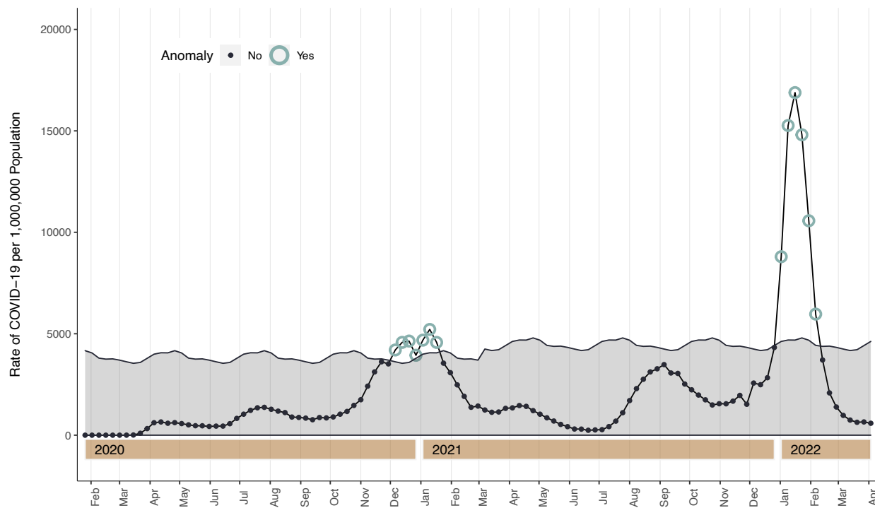
Figure s5. Twitter time series decomposition with generalized extreme studentized deviate (GESD) anomaly detection of US COVID-19 case rates, Mar 7, 2020 – Apr 9, 2022, with 10% maximum anomalies, Data Source: OWID
