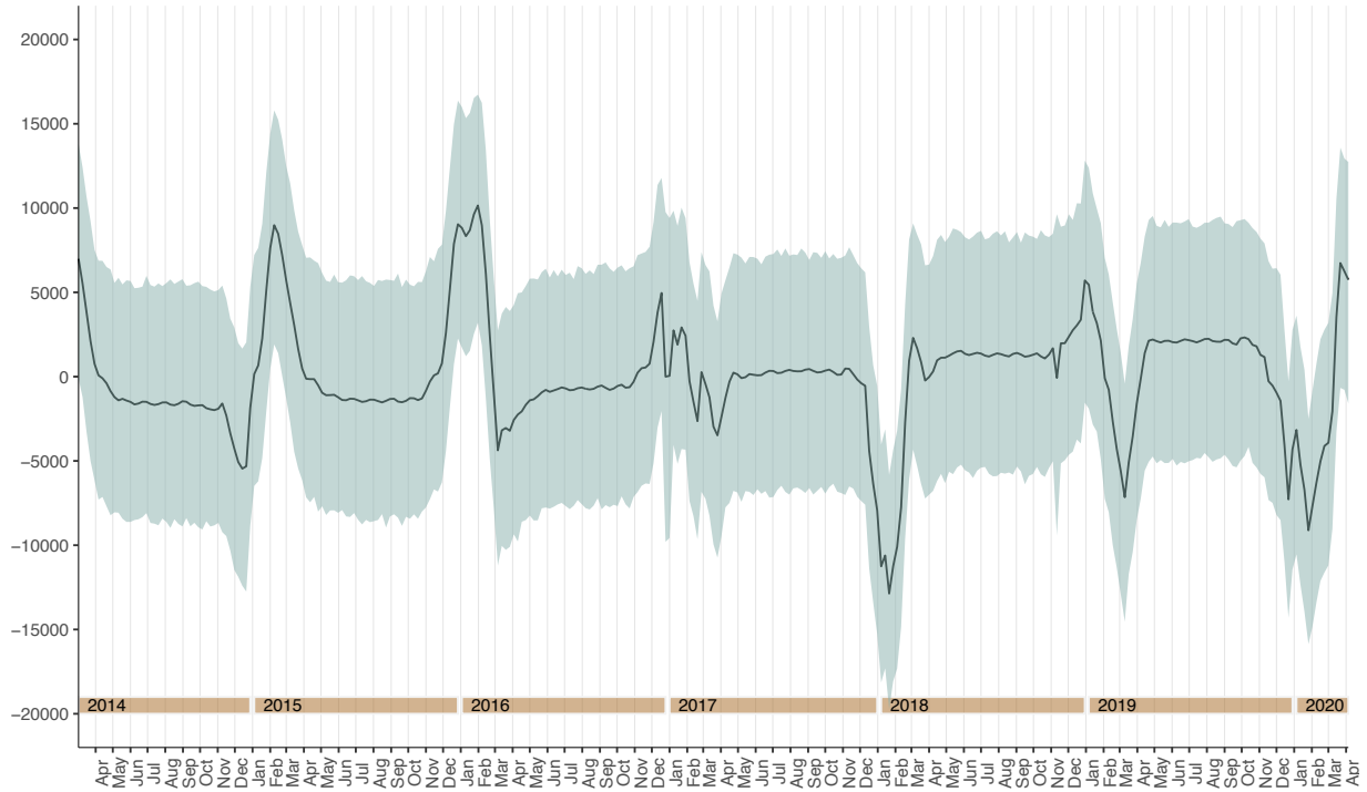
Figure s17. Residual component of Influenza cases from the Prophet decomposed model with Markov chain Monte Carlo Simulated 95% uncertainty intervals, Mar 1, 2014 – Apr 10, 2020, holiday-adjusted, United States. Data Source: US CDC
