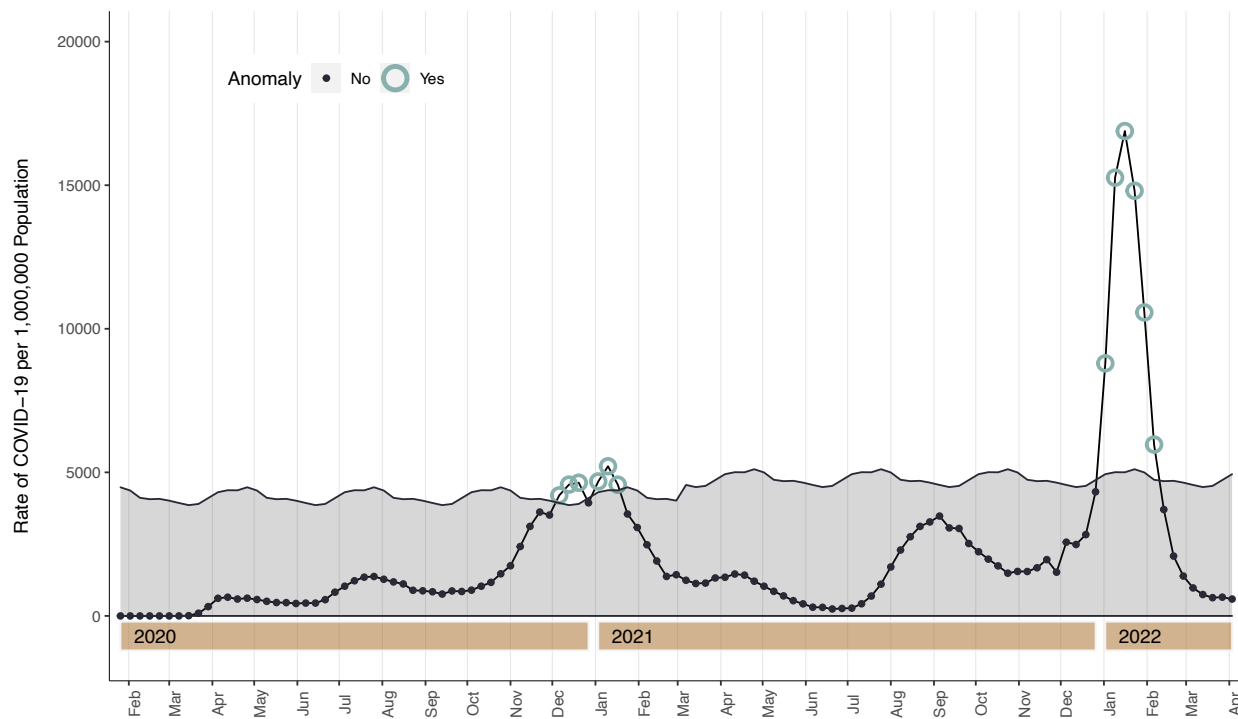
Figure s1. Twitter time series decomposition with generalized extreme studentized deviate (GESD) anomaly detection of US COVID-19 case rates, Mar 7, 2020 – Apr 9, 2022, with 1% maximum anomalies, Data Source: OWID
