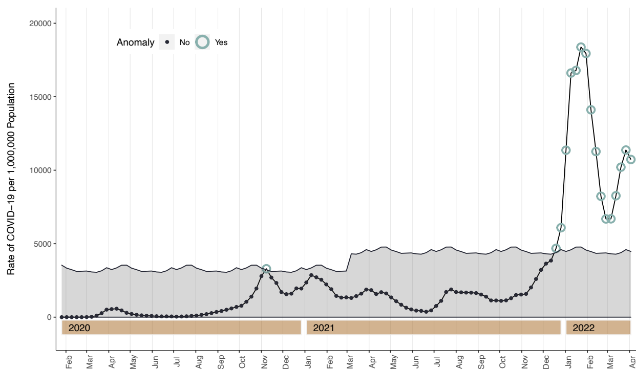
Figure s2. Twitter time series decomposition with generalized extreme studentized deviate (GESD) anomaly detection of EU-5 Country COVID-19 case rates, Mar 7, 2020 – Apr 9, 2022, with 1% maximum anomalies, Data Source: OWID
