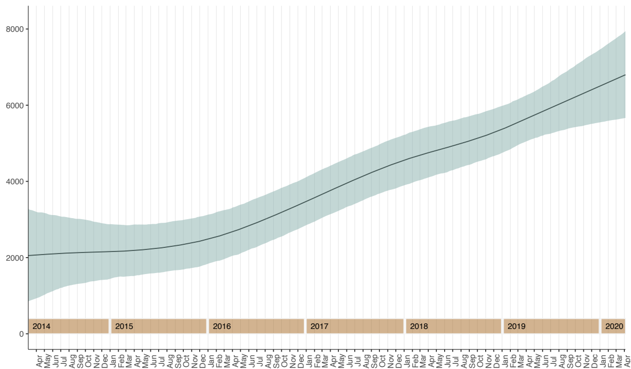
Figure s16. Trend component of Influenza cases from the Prophet decomposed model with Markov chain Monte Carlo Simulated 95% uncertainty intervals, Mar 1, 2014 – Apr 10, 2020, holiday-adjusted, United States. Data Source: US CDC
