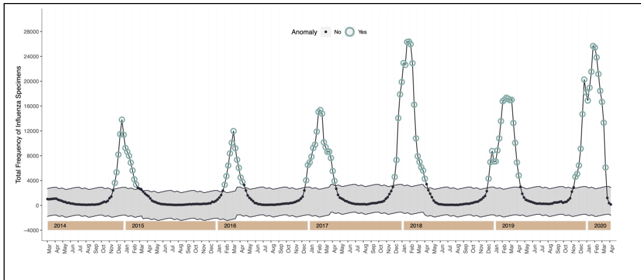
Figure 4: Twitter time series decomposition with generalized extreme studentized deviate (GESD) anomaly detection of Influenza cases, Mar 1, 2014 – Apr 10, 2020. Shaded areas represent the normal range of data points. Data Source: United States Centers for Disease Control and Prevention FluView
