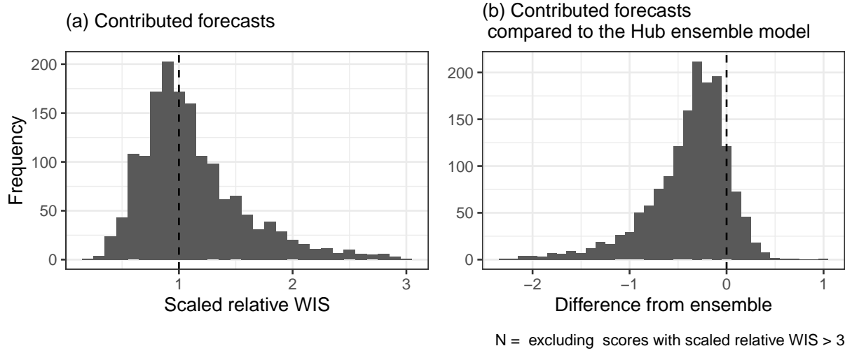
Figure 2: Comparison of scores between participating model forecasts and Hub ensemble of all available forecasts for each target
