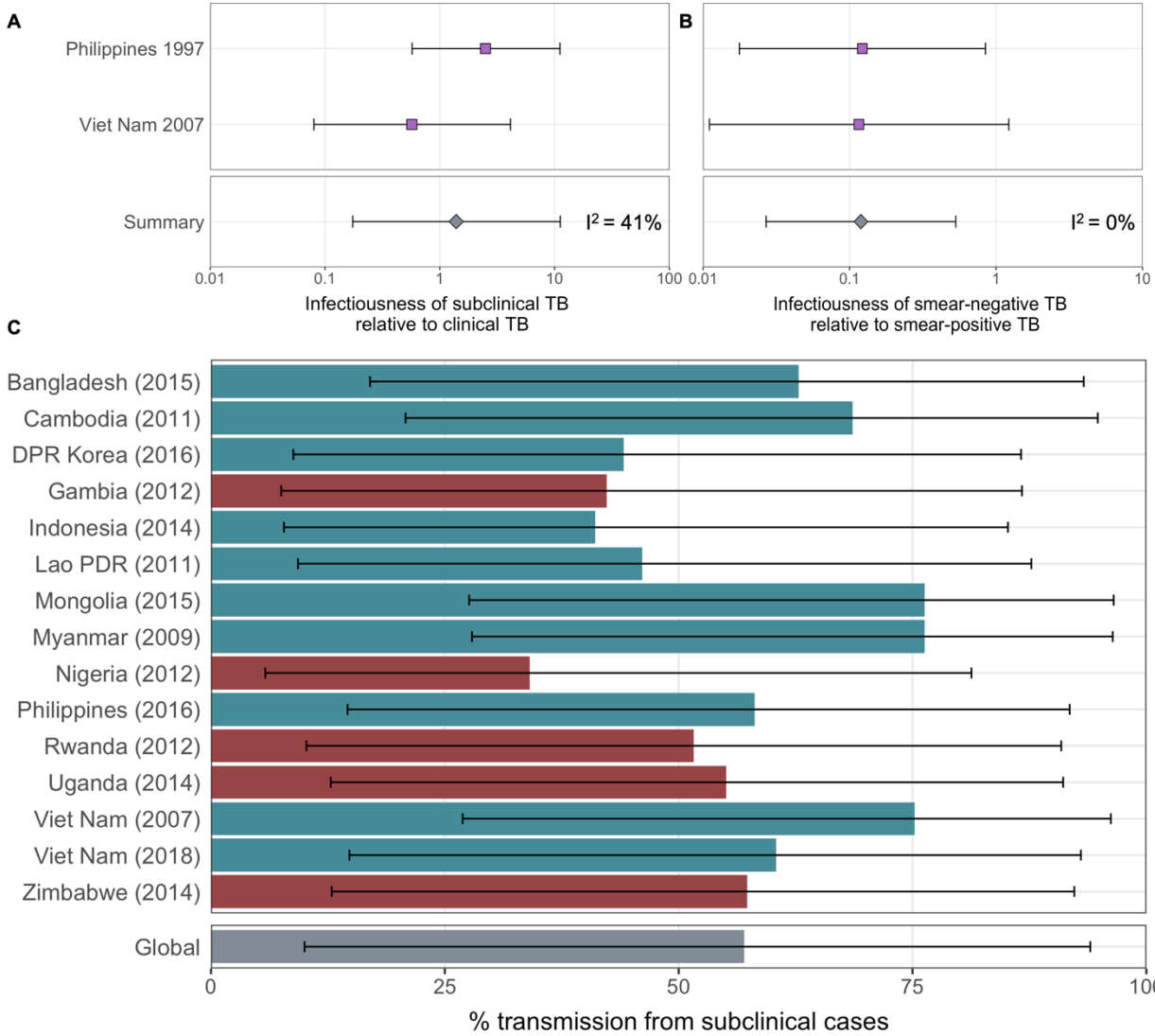
Supplementary Figure 6: Affected results for Sensitivity Analysis 2. Figure details are as per Figure 2A-B and Figure 3D in the main text.
