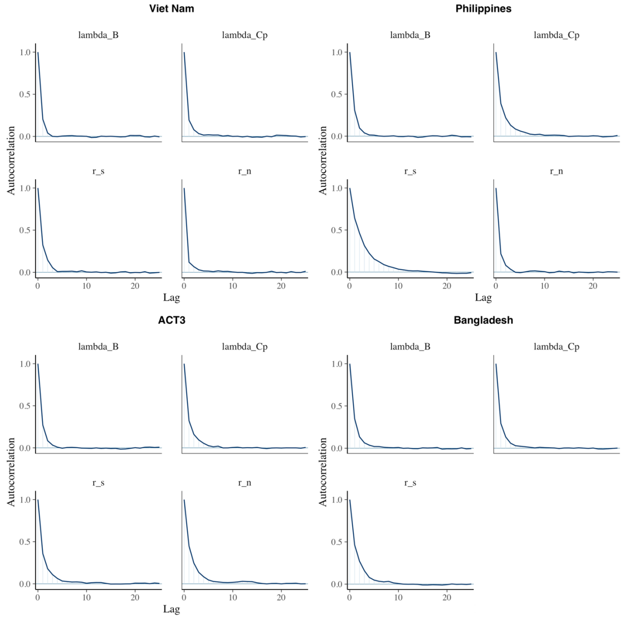
Supplementary Figure 5: Autocorrelation plots for each model.
