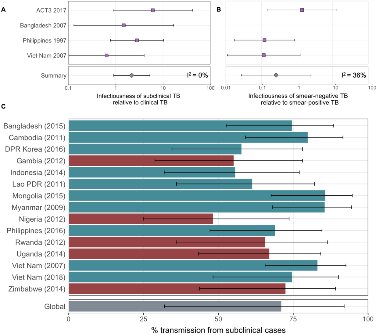
Supplementary Figure 7: Affected results for Sensitivity Analysis 2. Figure details are as per Figure 2A-B and Figure 3D in the main text.
