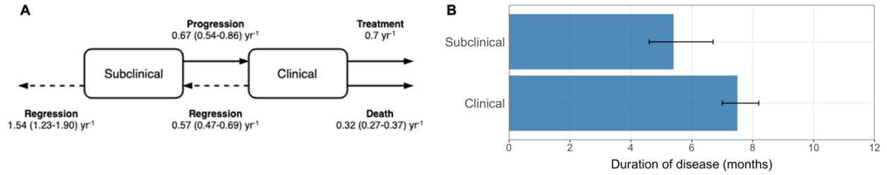
Supplementary Figure 1: Competing risk model (A) with transition rates from [22] used to estimate the durations of subclinical and clinical TB (B).
