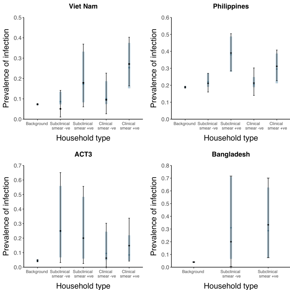
Supplementary Figure 2: Model fits for each model. Shown are prevalence of infection in members of households with different index case types (background, subclinical and smear-negative, subclinical and smear-positive, clinical and smear-negative, clinical and smear-positive). Error bars show median and 95% credible intervals. Shaded regions show posterior median and 95% posterior intervals. +ve = positive , -ve = negative .
