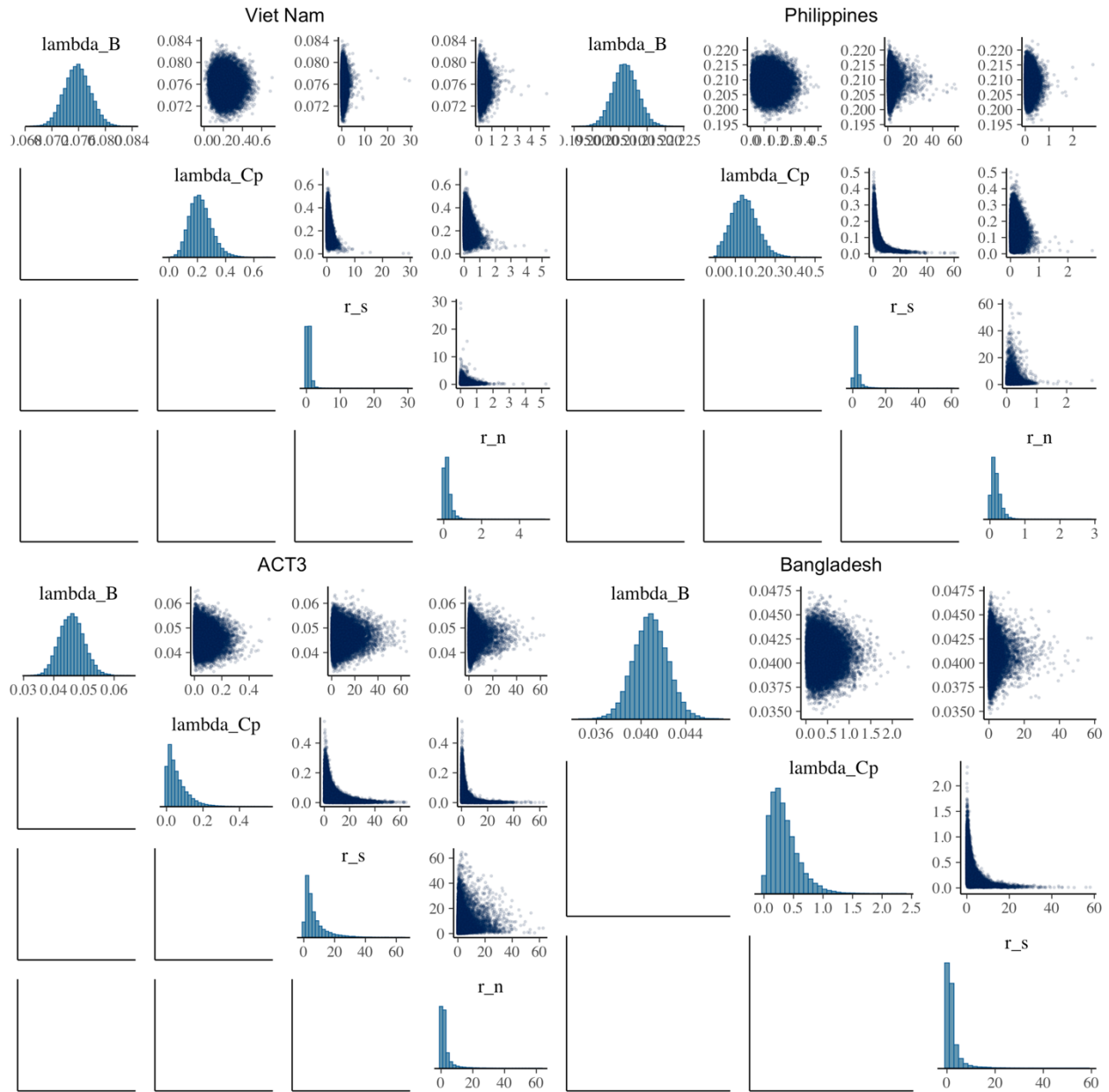
Supplementary Figure 4: Correlation plots for each model.
