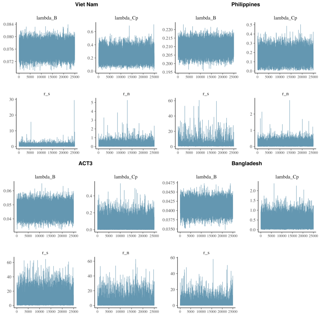
Supplementary Figure 3: Trace plots for each model.
