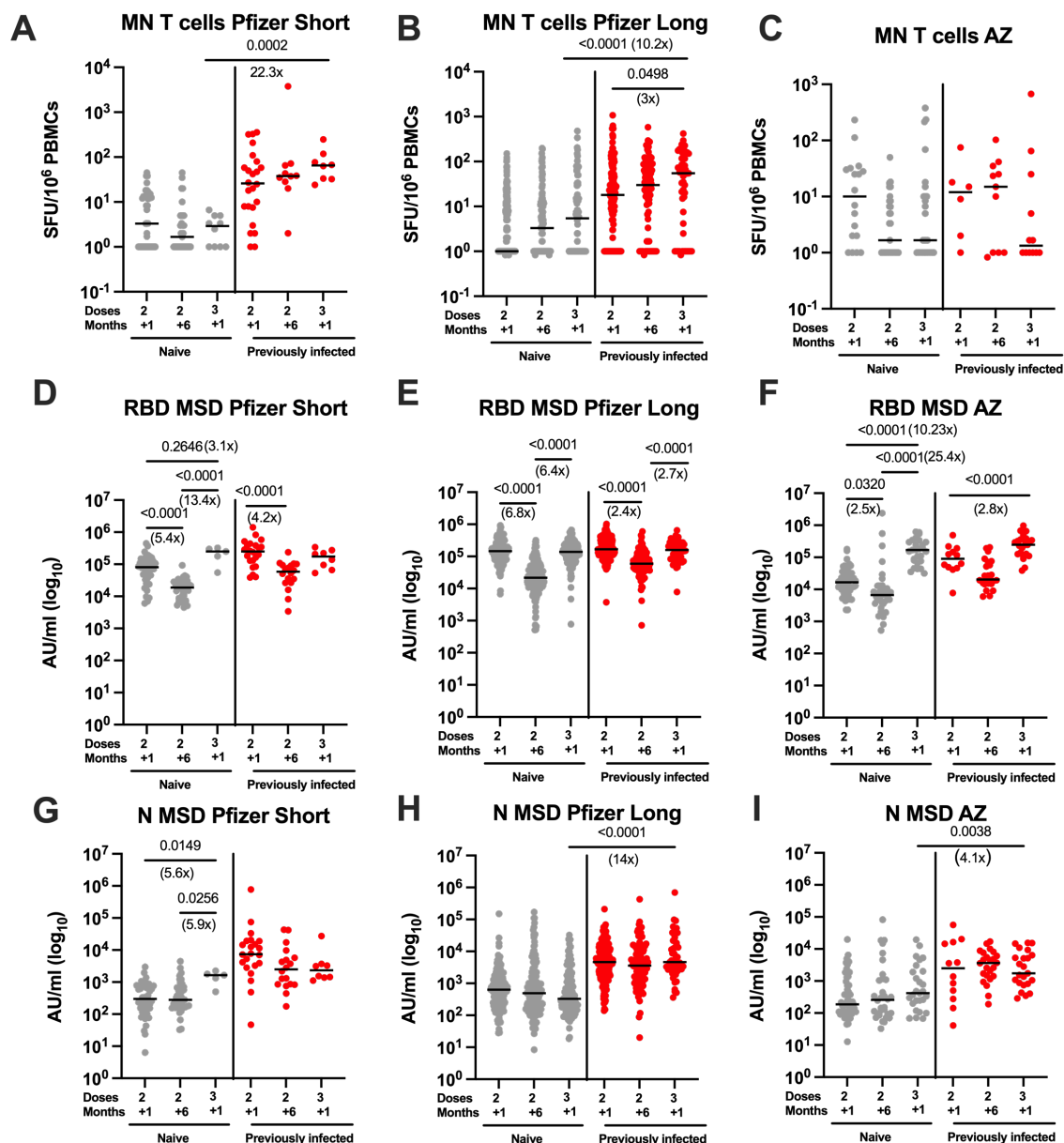
Figure S3: T cell and IgG Antibody responses to membrane protein, nucleocapsid protein and receptor binding domain.
