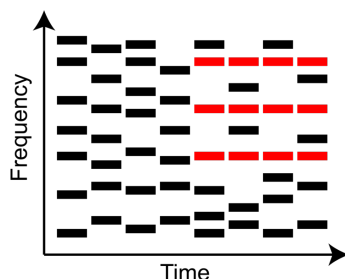
Figure 1. A schematic spectrogram of SFG stimulus.
