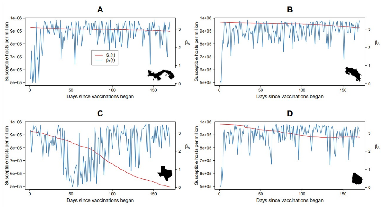
Fig. S1. Susceptible hosts per million (red lines) and the estimated daily infection coefficient \beta_A(t) (blue lines) of the ancestral strain A estimated from the Ensemble Kalman Filter routine
