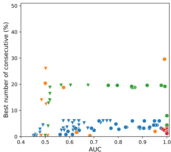
((d)) Time-series length 250
