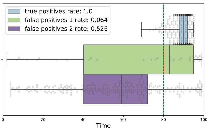
((c)) Wilk's Theorem
