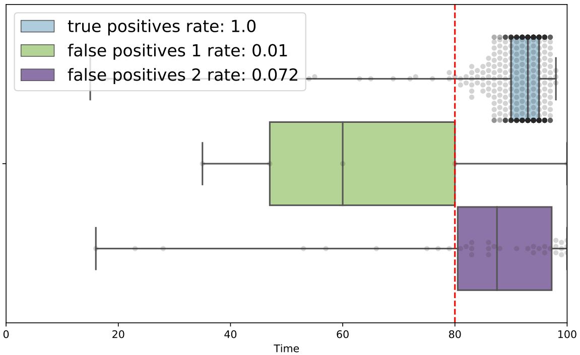
Figure 5: Quickest detection performance for different distributions f and g . Find \sigma_1^2 as the variance of the first 25 time-points of a time-series of length 100. For our 500 simulation sets, we find \sigma_1 \in [20.5, 53.4] . In this example, we take \sigma_1 = 40 and \sigma_2 = 10 and use a 6 consecutive points constraint, as before.
