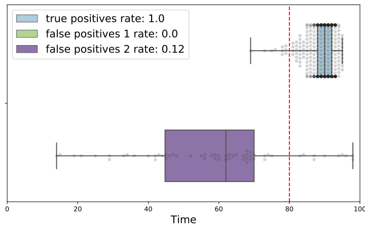
((e)) Modified Bayesian information criterion
