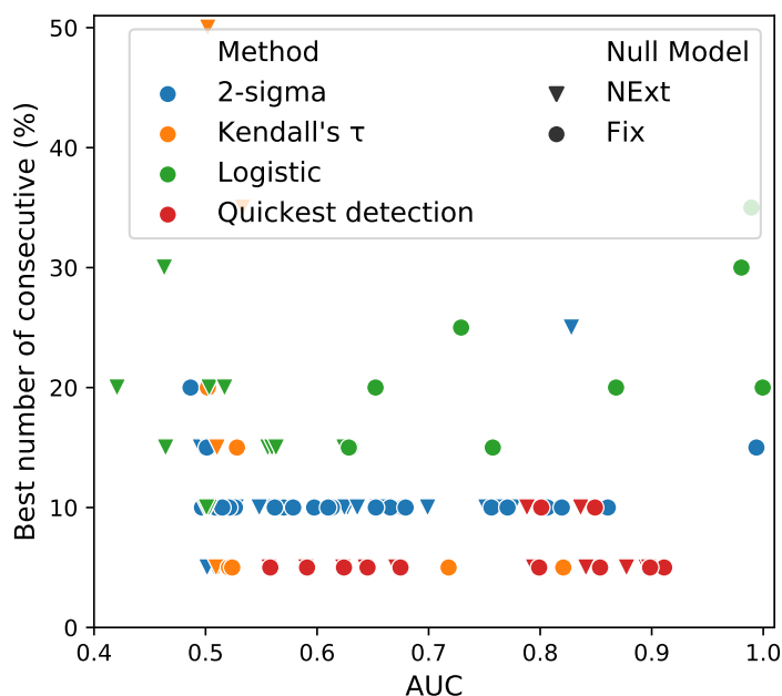
((a)) Time-series length 20
