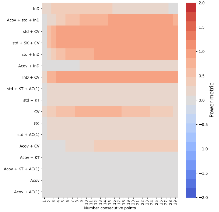
((b)) Logistic composite
