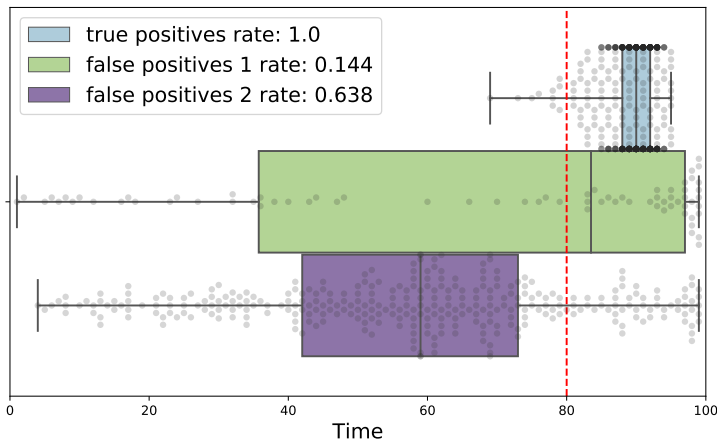
((a)) Hannan-Quinn information criterion
