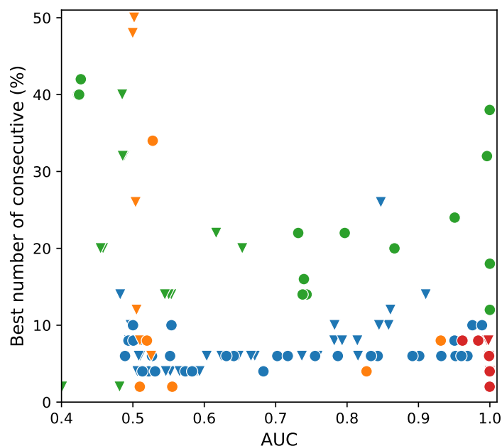
((b)) Time-series length 50
