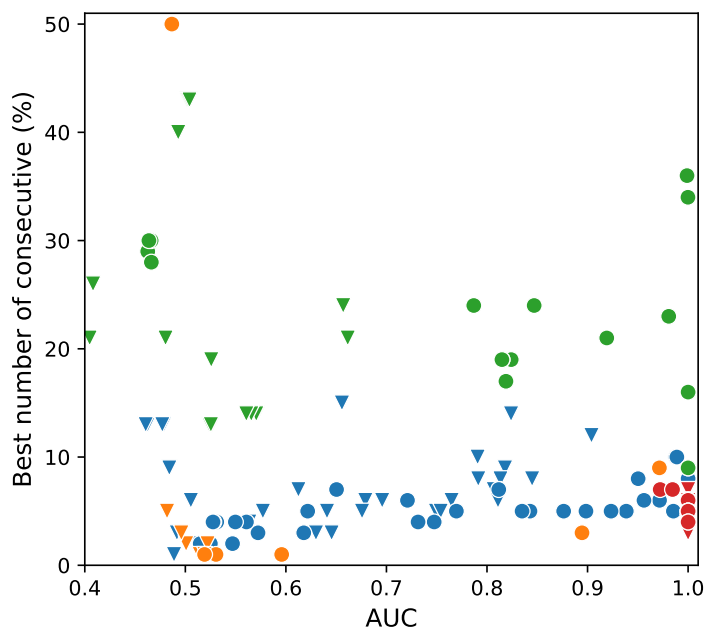
((c)) Time-series length 100
