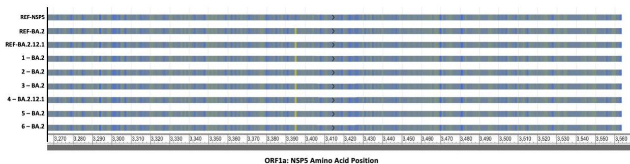
Supplemental Figure 1. Amino acid sequence of NSP5 (main viral protease, or Mpro) for individuals with recurring infection following nirmatrelvir-ritonavir treatment, compared to reference WT genome (GenBank YP_009725301.1). Ref-BA.2 (USA/MA-MGB-06410/2022) and Ref-BA.2.12.1 (USA/MA-MGB-05617/2022) genomes were collected via MGH surveillance sequencing and used as lineage-specific references. No mutations were found in drug-resistance conferring regions of the NSP5 gene of the six sequenced specimens.
