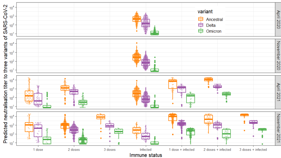
Figure 4 Predicted neutralization activity to three variants by immune status and date of sampling. Immune status was determined based on vaccinated status and infection status of the participants.
