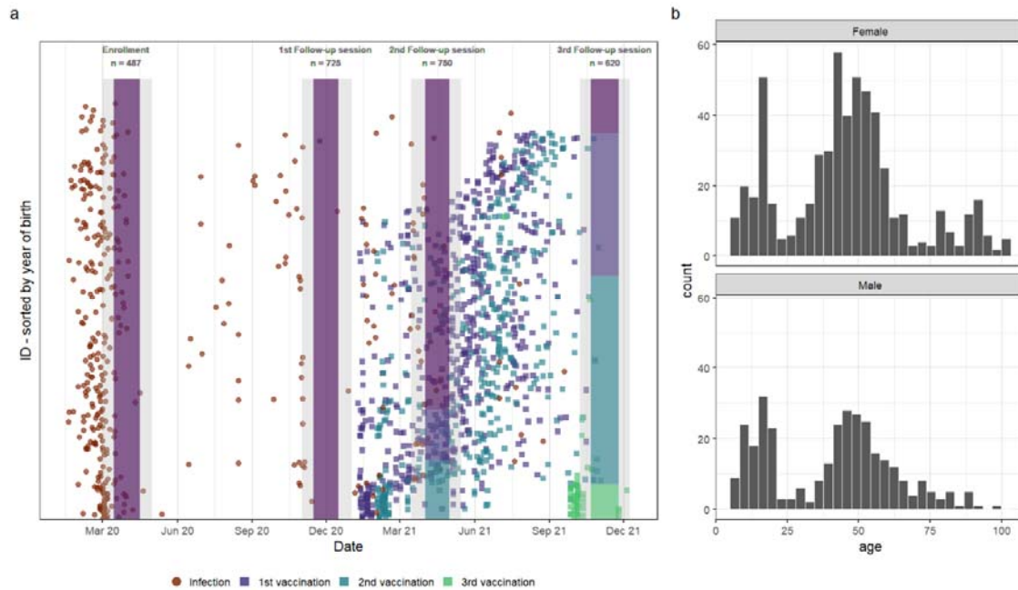
Figure 2 Overview of the study design and study population. (a) Analyses were based on four sessions of data and sera collection. Vaccination coverage is shown by the four stacked bar plots. Individual vaccination dates are shown in squares, color defines first, second and third dose. (b) Distribution of the study population by age and gender.
