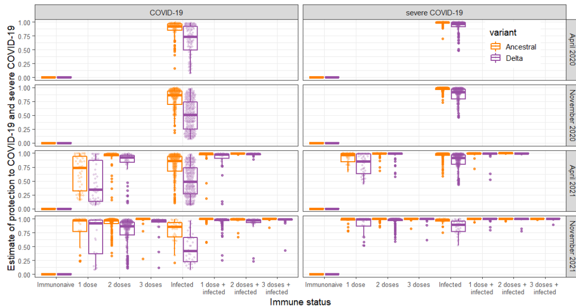
Figure 5. Estimates of reduced risk to COVID-19 and severe COVID-19 due to an infection with the ancestral and Delta variant among participants of the COVID-Oise cohort. Results are presented by sample collection sessions and by immune status due to vaccination and/or past infection.
