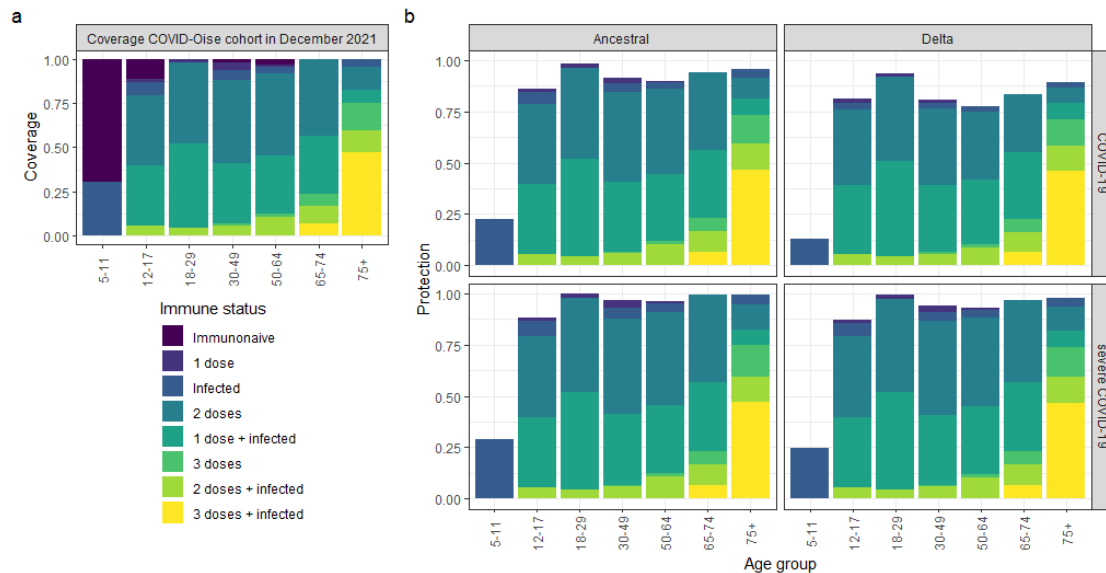
Figure 6. Aggregated protection against COVID-19 and severe COVID-19 in December 2021. (a) Coverage of vaccination and infection status by age group in participants of COVID-Oise cohort in December 2021. (b) Stacked median reduced risks to COVID-19 and severe COVID-19 by variant and age group.
