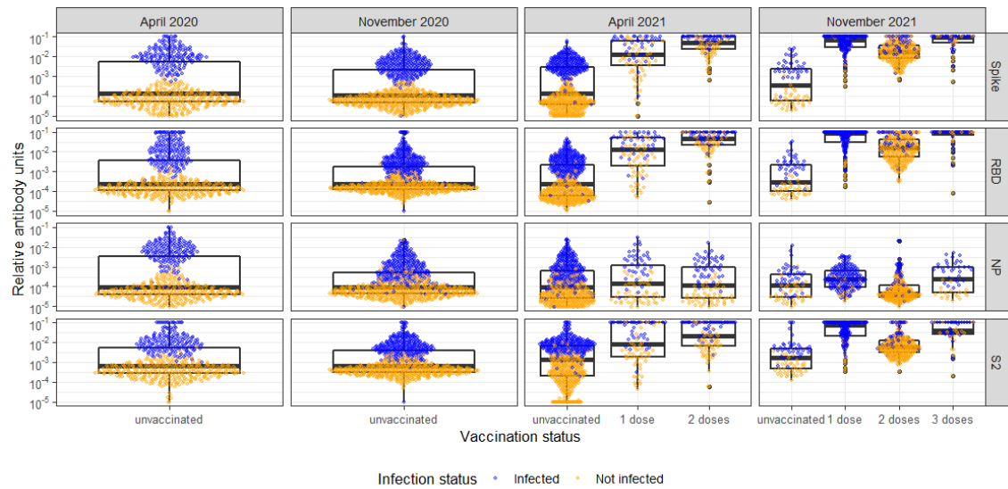
Figure 3. IgG antibody levels to the SARS-CoV-2 ancestral strain by vaccination status, moment of sampling and type of antigen. IgG antibodies are expressed as relative antibody units. Colours depict infection status.
