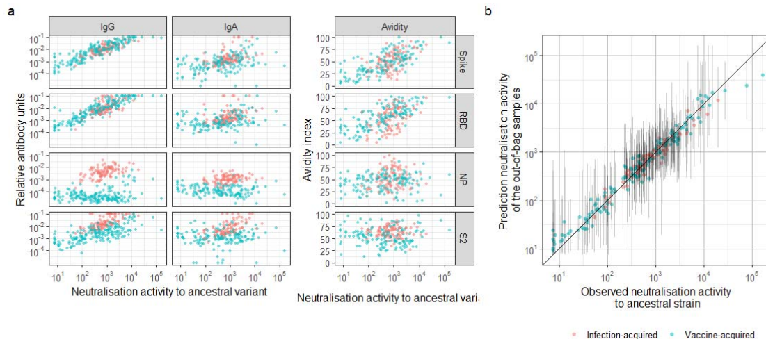
Figure 1. Establishment of a prediction model for neutralization activity based on measured antibody levels. a) Correlation between relative antibody units of Spike, RBD, NP and S2, for IgG, IgA and avidity and neutralizing activity to ancestral variant. b) Prediction of neutralization activity to the ancestral strain of SARS-CoV-2. The predictions were derived from a random forest regression model containing the following biomarkers: Spike IgG, RBD IgG, Spike IgG avidity, S2 IgG, RBD IgA and RBD IgG avidity.
